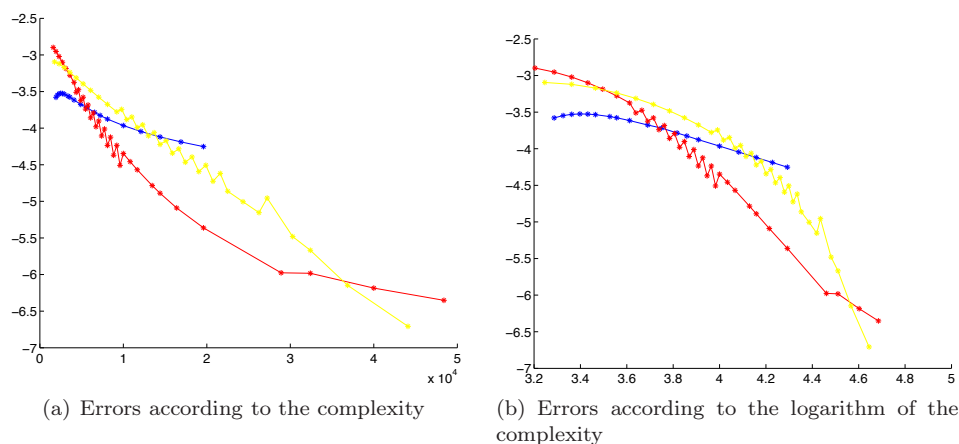
Figure 3.21: Errors on the energy according to the logarithm of the complexity
