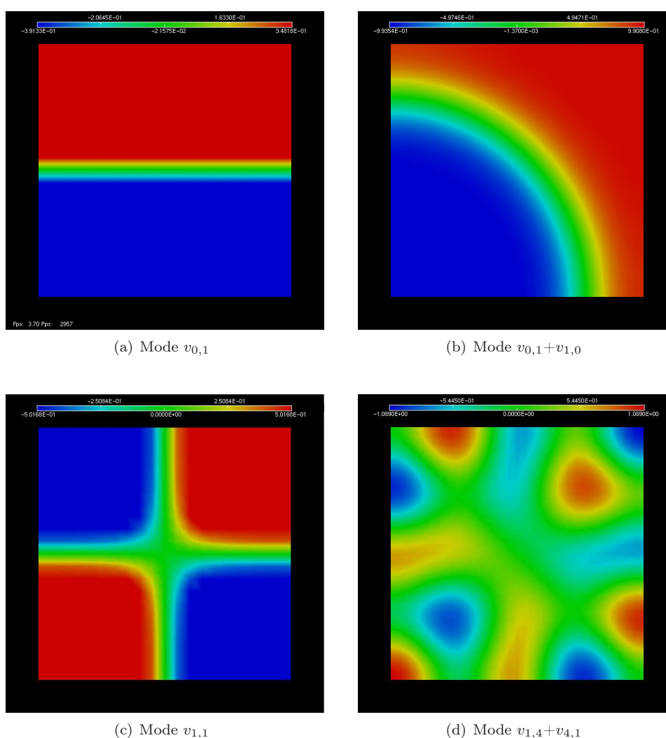
Figure 3.24: Asymptotic equilibria in the Maier-Paape-Miller nomenclature.
