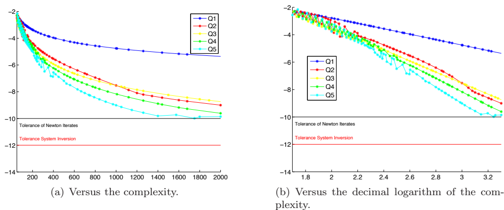
Figure 3.22: Comparison between the L^2 errors under the same complexity.
