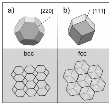
Figure 3. The tetraikadecahedron or Kelvin cell (a) and the rhombic dodecahedron (b) are the unit cells of two cubic foam structures. A view of the edges of such structures projected on a plane, respectively, normal to the [220] and [111] directions is shown in the lower part of each figure.
