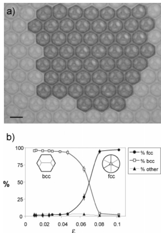
Figure 8. (a) In the photograph, a region of interest with well-defined crystalline order is highlighted. The scale bar represents 200\ \mu\text{m} . (b) The percentages of bubbles in fcc, bcc, or other structures are shown as a function of liquid volume fraction \epsilon . The typical error bars correspond to uncertainty in the position of the point A due to the size of the pixels. The inset shows typical patterns seen in bcc or fcc foam.
