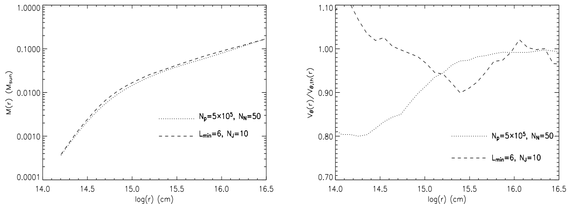
Figure 5.7: (left): Total integrated mass in the equatorial plane at t_0 as a function of the radius for AMR calculations with \ell_{\text{min}} = 6 , N_J = 10 (dashed-line) and for SPH calculations with N_p = 5 \times 10^5 , N_N = 50 (dotted line). (Fig.5.7right): Ratio between numerical and theoretical azimuthal velocities at t_0 as a function of the radius in the equatorial plane for the same calculations.
