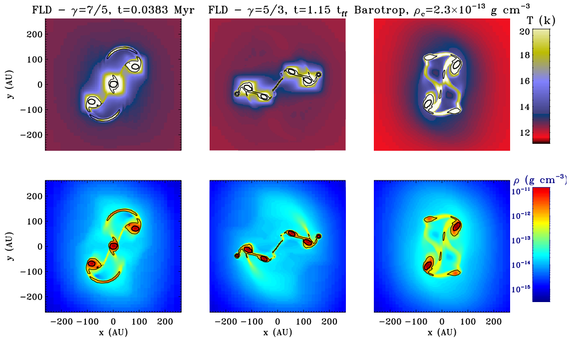
Figure 6.6: Density and temperature maps in the equatorial plane at time t = 38.3 \text{ kyr} ( 1.15 t_{\text{ff}} ), for three calculations run with the FLD approximation and \gamma = 7/5 ( left ), the FLD approximation and \gamma = 5/3 ( middle ) and with a barotropic EOS using \rho_{\text{ad}} = 2.3 \times 10^{-13} \text{ g cm}^{-3} and \gamma = 5/3 ( right ).
