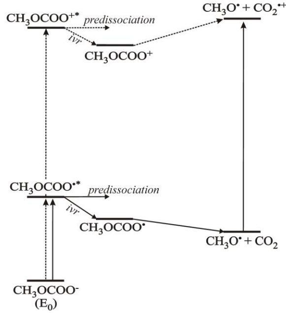
Figure IV.3-5: Illustration of the neutral (full line) and ionic (dotted line) processes occurring during the neutralization-reionization of \text{CH}_3\text{OCOO}^- . For each ion, the corresponding translational energy is indicated in brackets. ivv stands for intramolecular vibrational relaxation (for the sake of clarity, no activation energy is shown for dissociation of methylcarbonate neutral, even though this feature is present (see next section)).
