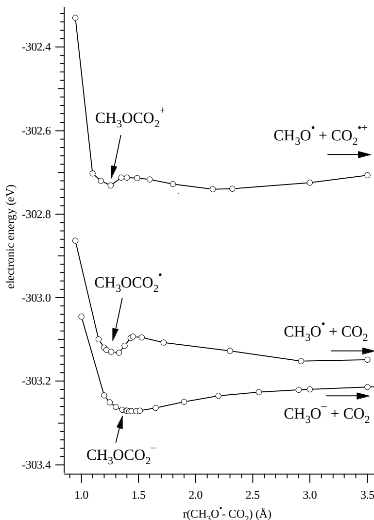
Figure IV.4-1: Projection of the [\text{C}_2\text{H}_3\text{O}_3]^{-/+} potential-energy surfaces on the r(\text{CH}_3\text{O}^\bullet - \text{CO}_2) coordinate as determined by single point energy calculations (MP2/6-311++G(3df,3pd)//MP2/6-311++G(d)). Here, the \text{CH}_3\text{O}^\bullet - \text{CO}_2 bond was kept frozen, while all other parameters of the species were fully optimized. The PESs have been extrapolated from several optimized structures of anion, radical and cation, indicated by a circle (○).
