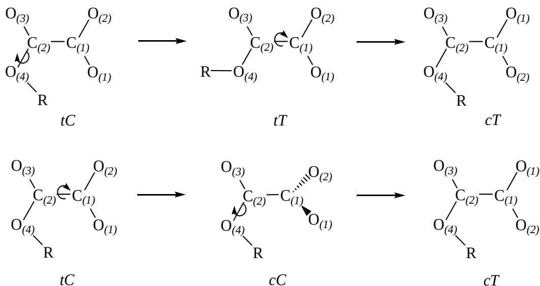
Scheme V.2-2: The two mechanisms for passage of the conformation tC to the conformation cT for alkylloxalate radicals ROCOOCO\cdot ( R = H, CH_3, C_2H_5, i\text{-}C_3H_7 , and t\text{-}C_4H_9 ).
