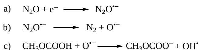
Scheme II.2-1: The three steps of the NICI of methylcarbonate with N 2 O as reagent gas.
