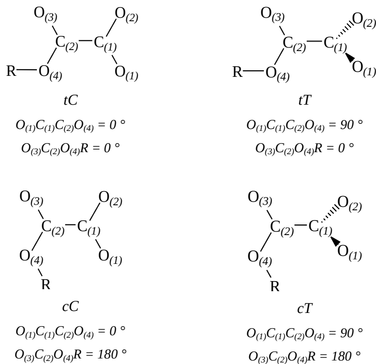
Chart V.2-1: The four conformations of alkyloxalates anions \text{ROCOCOO}^- ( 6 - to 10 - , \text{R} = \text{H} , \text{CH}_3 , \text{C}_2\text{H}_5 , i\text{-C}_3\text{H}_7 , and t\text{-C}_4\text{H}_9 ) for limiting values of the dihedral angles O_{(1)}C_{(1)}C_{(2)}O_{(4)} and O_{(3)}C_{(2)}O_{(4)}R .
