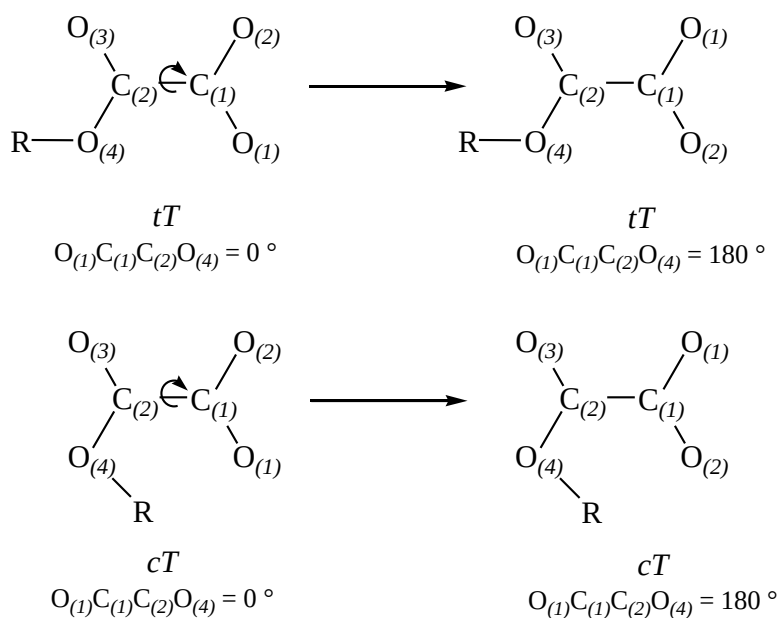
Scheme V.2-1: The conformational structure of alkyloxalates ROCOCOO^- ( R = H, CH_3, C_2H_5, i-C_3H_7 , and t-C_4H_9 ) is conserved by rotation of 180^\circ around the C_{(1)}-C_{(2)} axis due to the symmetry of the carboxylate group.
