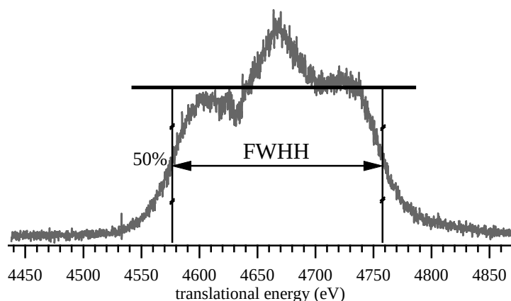
Figure IV.3-7: Method used to measure the FWHH associated to the \text{CO}_2^{*+} signal obtained by dissociation of transient \text{CH}_3\text{OCOO}^* and which gives access to the kinetic energy released in the course of this process.
