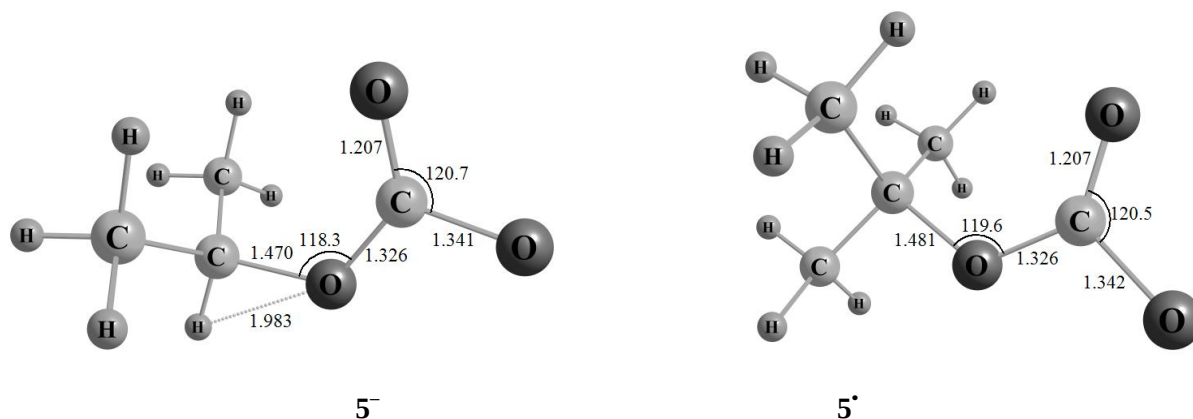
Chart III.2-1: Optimized geometries of alkyloxalate ions and radicals 1^{-\bullet} to 5^{-\bullet} obtained at the MP2/6-311++G(d) level of theory.
