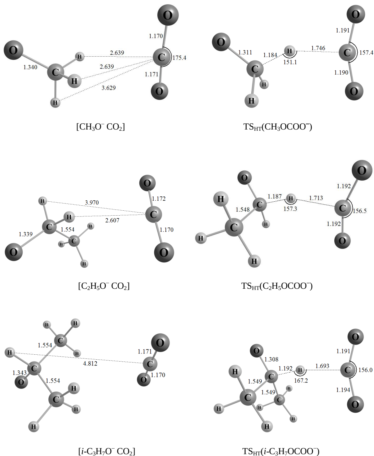
Chart III.4-1: Optimized structures of the ion-neutral complexes [RO - CO 2 ] and the transition states TS HT for methyl-, ethyl, and i -propylcarbonates (R = CH 3 , C 2 H 5 , and i -C 3 H 7 ) (bond lengths in Å, angles in degree).
