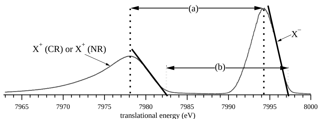
Figure IV.2-3: The two methods to measure the translational energy losses Q_{\min, \text{CR}, \text{exp.}} or Q_{\min, \text{NR}, \text{exp.}}(\text{X}^+) . The translational energies of the parent and fragment ions are obtained from (a) the top of the peaks or (b) by the extrapolation of the high-energy onset of the ion signals to the baseline.
