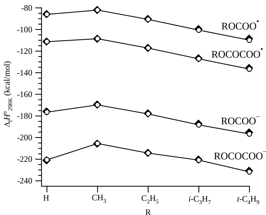
Figure VI.1: Standard heats of formation obtained for alkylcarbonate and alkylloxalate ions and radicals \text{ROC}\dot{\text{O}}\text{O}^{-\bullet} and \text{ROCOC}\dot{\text{O}}\text{O}^{-\bullet} ( \text{R} = \text{H}, \text{CH}_3, \text{C}_2\text{H}_5, i\text{-C}_3\text{H}_7, \text{and } t\text{-C}_4\text{H}_9 ), using atomization energies ( \blacklozenge ) and bond-separation reactions ( \circ ).
