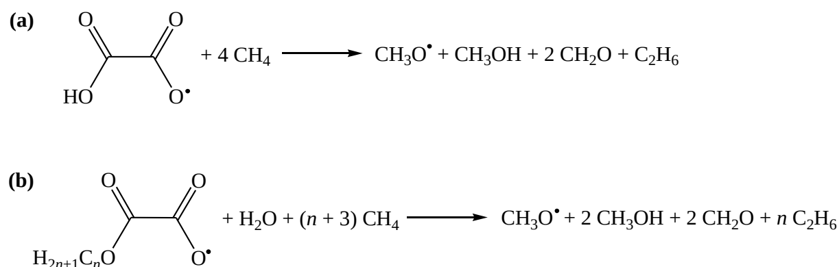
Scheme V.3-1: Bond-separation reactions used for the determination of the standard heats of formation of (a) hydrogen oxalate radical 6 • and (b) alkyloxalate radicals 7 • to 10 • (for n = 1 to 4).
