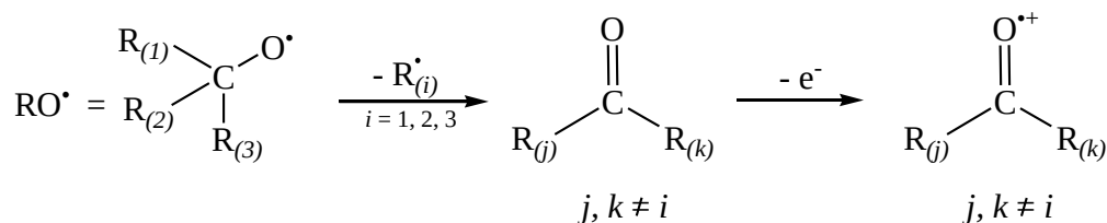
Scheme III.5-1: Fragmentation occurring for an alkoxy radical \text{RO}^\bullet (with side chains bearing three or less carbon atoms) and the fragments obtained after reionization to cation according to Hornung. 41
