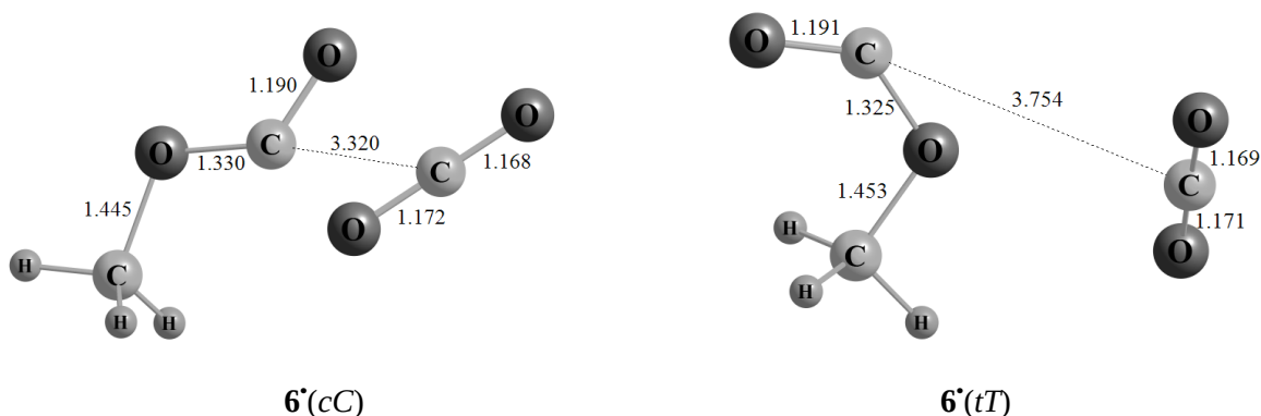
Chart V.2-6: Optimized structures of the conformers cC and tT of methyloxalate 6 • according to MP2/6-311++G(d) calculations.
