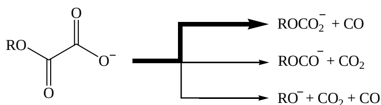
Scheme V.4-1: General dissociation scheme of alkylloxalates \text{ROCOCOO}^- for \text{R} = \text{H}, \text{CH}_3, \text{C}_2\text{H}_5, i\text{-C}_3\text{H}_7, \text{and } t\text{-C}_4\text{H}_9 . The bold arrow indicates the main dissociation pathway.
