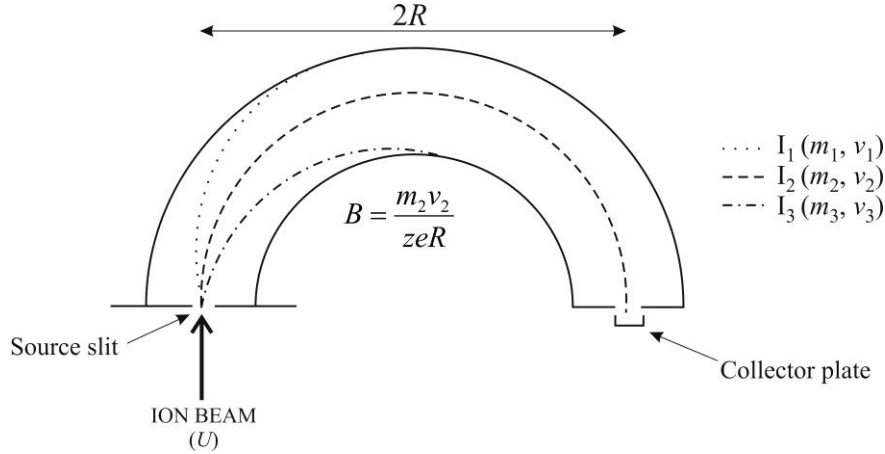
Figure II.2-2: Illustration of ion selection in a magnetic sector. The ion beam is constituted in this example of three ions I_1(m_1, v_1) , I_2(m_2, v_2) and I_3(m_3, v_3) of charge z . In the conditions of the experiment (accelerating voltage U , magnetic field B ), only I_2 has a circular trajectory of radius R which is the radius of the magnetic sector and is transmitted to the collector plate. The radii of the trajectories of I_1 and I_3 are too large or too small, respectively, and these ions are not transmitted further.
