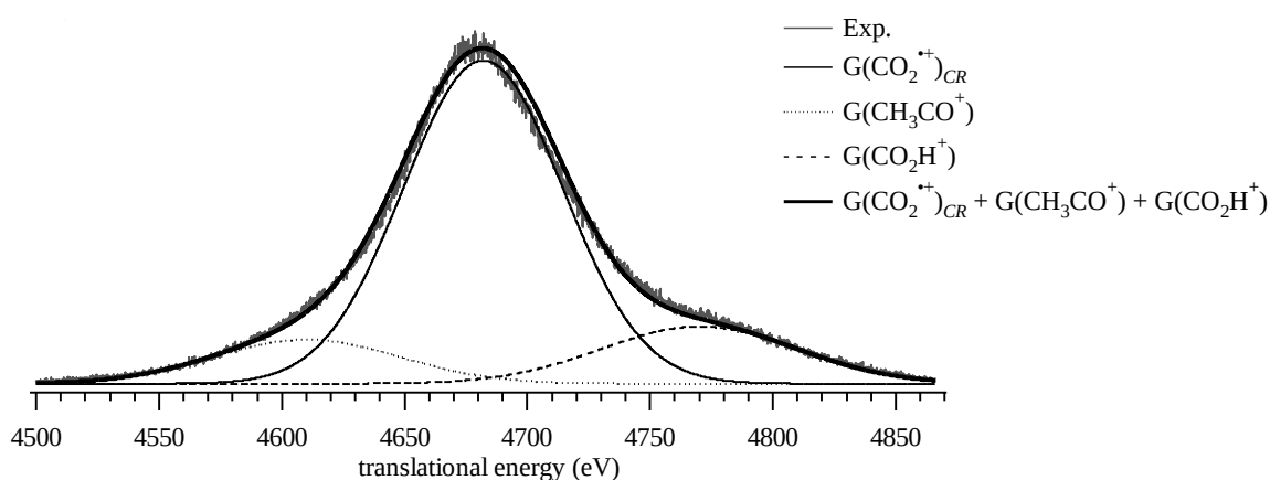
Figure IV.3-2: Fit of the TE signal of \text{CO}_2^{*+} , \text{CH}_3\text{CO}^+ , and \text{CO}_2\text{H}^+ formed from dissociation of \text{CH}_3\text{OCOO}^+ obtained by CR from \text{CH}_3\text{OCOO}^- .
