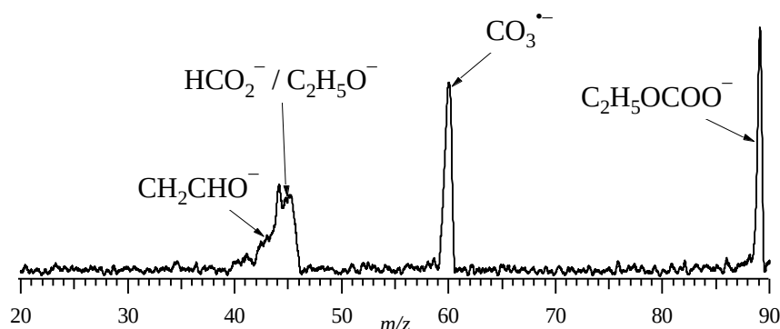
Figure III.5-1: \text{NR}^- spectrum of B1-mass selected \text{C}_2\text{H}_5\text{OCOO}^- \text{ } 3^- ( m/z = 89 ) using \text{O}_2 (C2, 80 % T) and Xe (C3, 80 % T).
