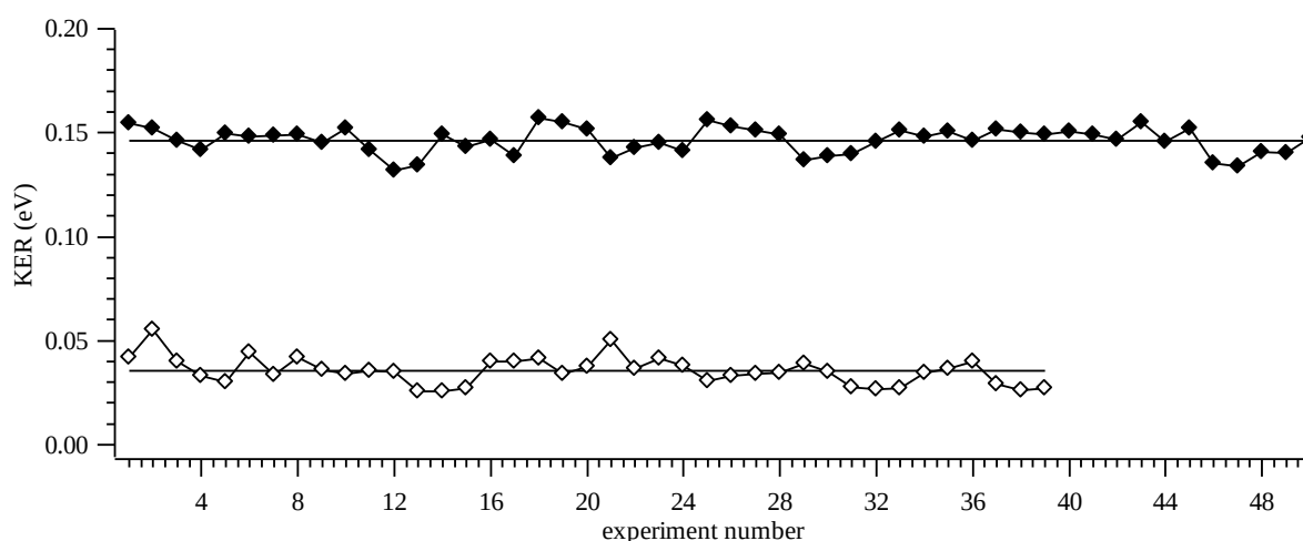
Figure IV.3-8: All KER values (eV) obtained from the \text{CO}_2^{*+} signal formed from CR (◇) or NR (◆) experiments of \text{CH}_3\text{OCOO}^- .
