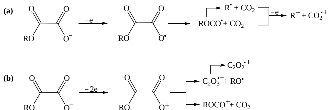
Scheme V.5-2: General scheme of dissociation of (a) alkylloxalate radicals \text{ROCOCOO}^* and (b) (carboxyalkyl)carboxyl ions \text{ROCOCOO}^+ , both obtained by vertical electron transfer from the corresponding alkylloxalate anions ( \text{R} = \text{C}_2\text{H}_5 , i\text{-C}_3\text{H}_7 , and t\text{-C}_4\text{H}_9 ).
