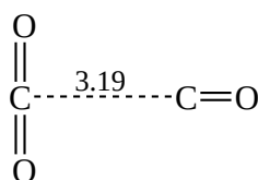
Chart V.4-1: Structure of most stable isomer of ^1\text{C}_2\text{O}_3 . The bond length (in Å) is taken from Peppe et al. 15
