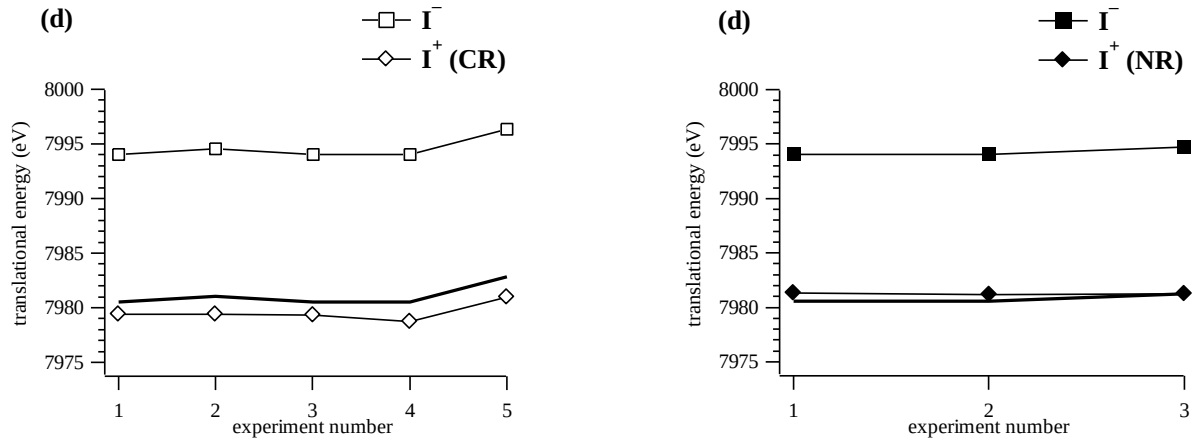
Figure IV.2-5: All TE values obtained for \text{X}^- and \text{X}^+ (formed by CR or NR of \text{X}^- ) for the atomic gases (a) O, (b) \text{Cl}^* , (c) \text{Br}^* , and (d) \text{I}^* . One experiment (termed 1,2,..) consists in the recording of the TE spectrum of the ion \text{X}^- followed by that of \text{X}^+ (CR or NR) (see text). Each experiment number is related to a square and a diamond of the same color ( \square/\diamond or \blacksquare/\blacklozenge ) which correspond to average TEs of \text{X}^- and of \text{X}^+ (CR, white or NR, black). Further, in each graph, a bold line indicates the expected TE of \text{X}^+ (CR or NR), obtained by subtracting (IE(\text{X}^*) - EA(\text{X}^*)) to the TE of \text{X}^- . As discussed above, these TEs values are measured on the tops of the peaks.
