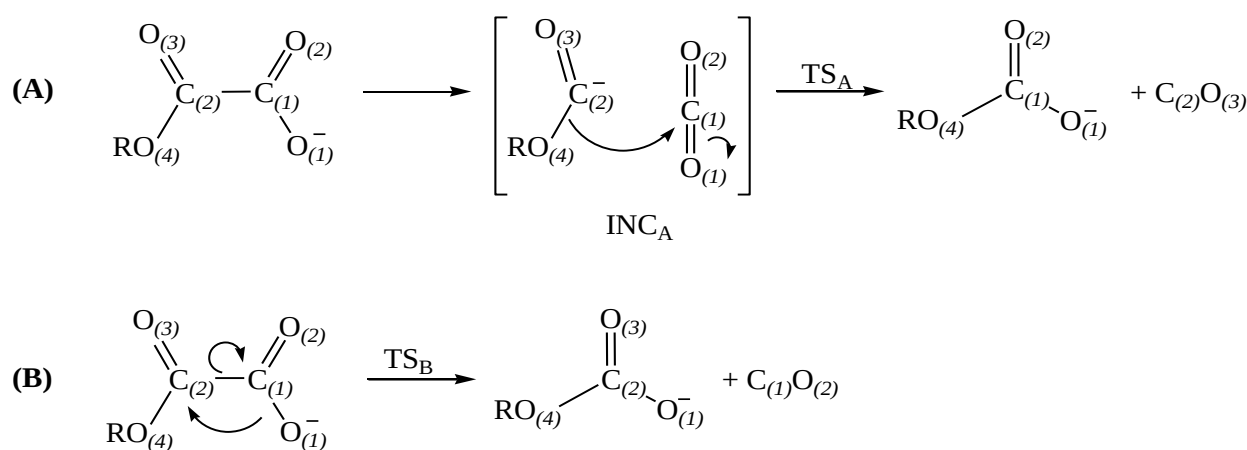
Scheme V.4-2: Two mechanistic variants for the decarbonylation of alkylloxalates \text{ROCOCOO}^- ( \text{R} = \text{H}, \text{CH}_3, \text{C}_3\text{H}_5, i\text{-C}_3\text{H}_7, \text{and } t\text{-C}_4\text{H}_9 ).
