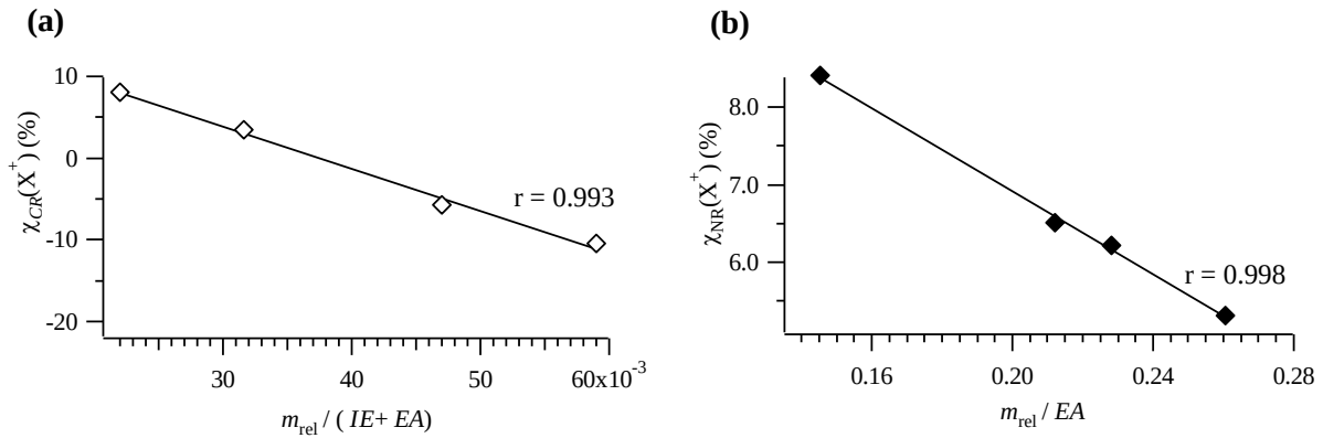
Figure IV.2-6: Variation of (a) the relative error \chi_{\text{CR}}(X^+) as a function of m_{\text{rel}} / (IE + EA) and of (b) \chi_{\text{NR}}(X^+) as a function of m_{\text{rel}} / EA . The values of \chi_{\text{CR}}(X^+) and \chi_{\text{NR}}(X^+) are taken from Table IV.2-2 and correspond to the deviation of the experimental kinetic energies losses for the atomic ions submitted to \text{CR}^+ ( \diamond ) and \text{NR}^+ ( \blacklozenge ) experiments compared to theory. Linear fits (full line) are indicated for each type of experiments as well as the resulting correlation coefficients r . 20
