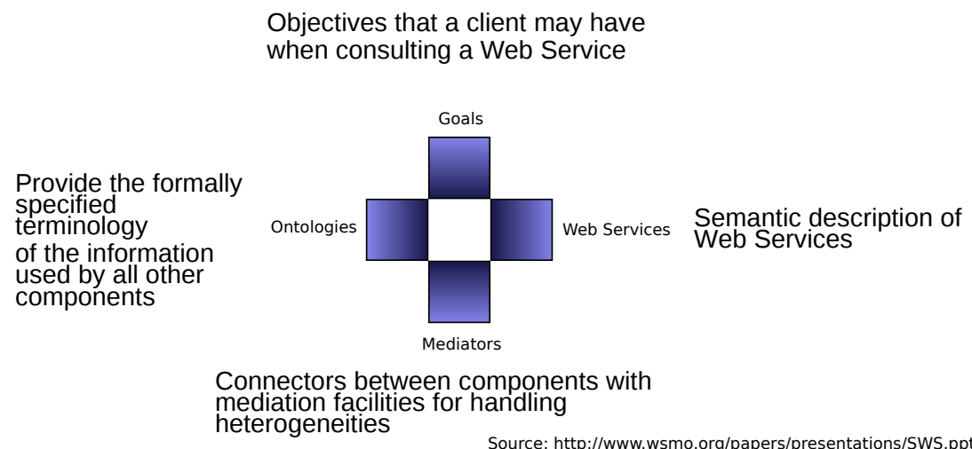
Figure 3.5: The four facets of WSMO services.
