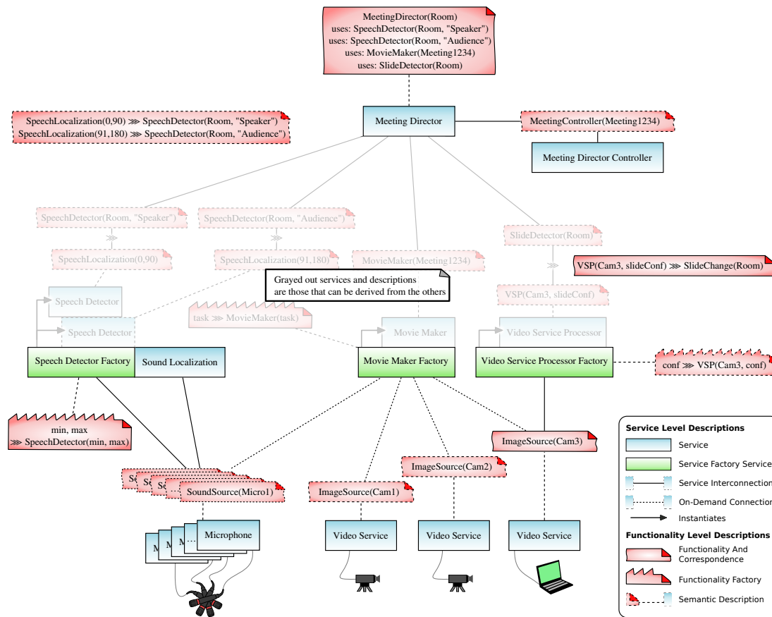
Figure 6.6: Automatic Cameraman: What Can be Derived. Same figure as 6.5 but showing what has to be provided by designers. Lighter parts of the schema are all the elements that are automatically derived and instantiated.
