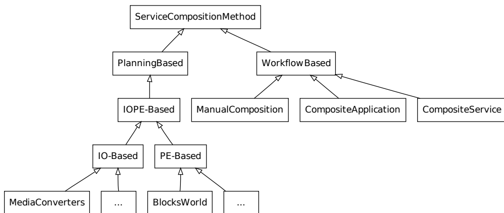
Figure 3.6: Classification of Service Composition Methods.
