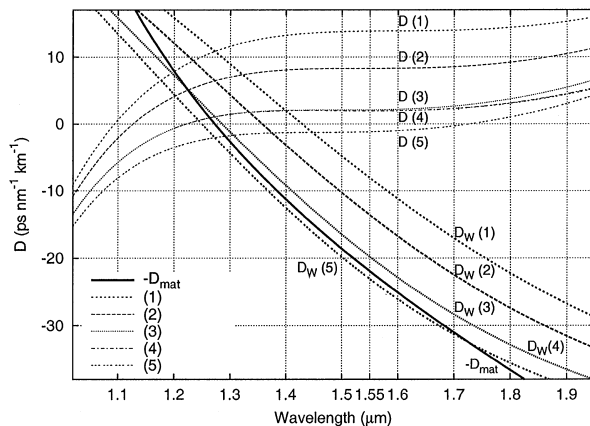
Fig. 4. Waveguide dispersion D_W , dispersion D for the MOF structures that we proposed, and sign-changed material dispersion -D_{mat} . Unless stated, the total number of rings N_r in the MOF is three. The line style of a MOF structure is identical for D_W and D . \Lambda and the diameters are given in micrometers. d_n is the hole diameter of the n th ring, and d_{n_1-n_2} denotes the hole diameter of the n_1 th to n_2 th rings. (1) \Lambda = 1.9 , d_1 = 0.559 , d_2 = 0.782 , d_3 = 0.894 ; (2) \Lambda = 1.8 , d_1 = 0.529 , d_2 = 0.741 , d_3 = 0.847 ; (3) \Lambda = 1.7 , d_1 = 0.5 , d_2 = 0.7 , d_3 = 0.8 ; (4) N_r = 4-7 , \Lambda = 1.7 , d_1 = 0.5 , d_2 = 0.7 , d_{3-7} = 0.8 ; (5) \Lambda = 1.65 , d_1 = 0.485 , d_2 = 0.679 , d_3 = 0.776 .
