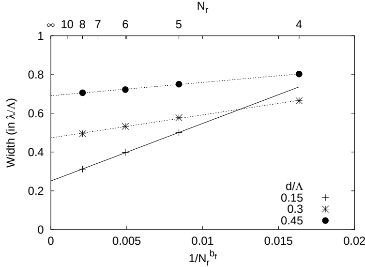
FIG. 3.20 – Half-width of the negative Q peak of the fundamental mode as a function of 1/N_r^{bf} . The width of the peak converges to a non-vanishing value. Here b_f \simeq 2.97 . This figure must be compared to Fig. 3.12 obtained for the second mode.
