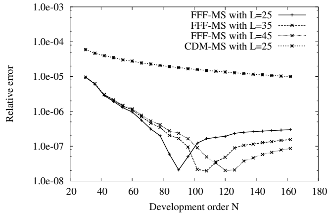
FIG. 2.31 – Modulus of the relative difference between the effective indices n_{\text{eff}} computed with the FFF-MS for 25, 35 and 45 slices in the S -algorithm, and with the MM result, versus the Fourier expansion order N (for the MM the number of Fourier-Bessel coefficients is equal to 12).
