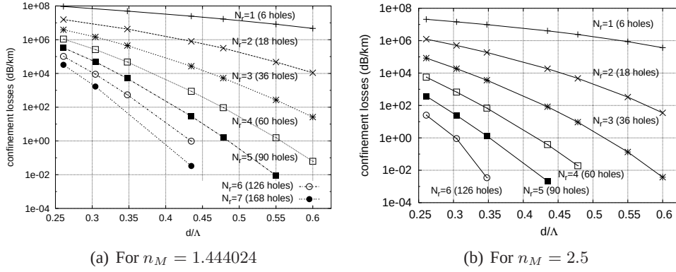
FIG. 3.5 – Confinement losses (in dB/km with a log-scale) versus the ratio (d/\Lambda) and the number N_r of hole rings around the solid core. The MOF are based on a C_{6v} triangular lattice of air holes in an infinite matrix. The pitch \Lambda is equal to 2.3 \mu\text{m} , and \lambda = 1.55 \mu\text{m} . N_r is the number of air hole rings surrounding the solid core.
