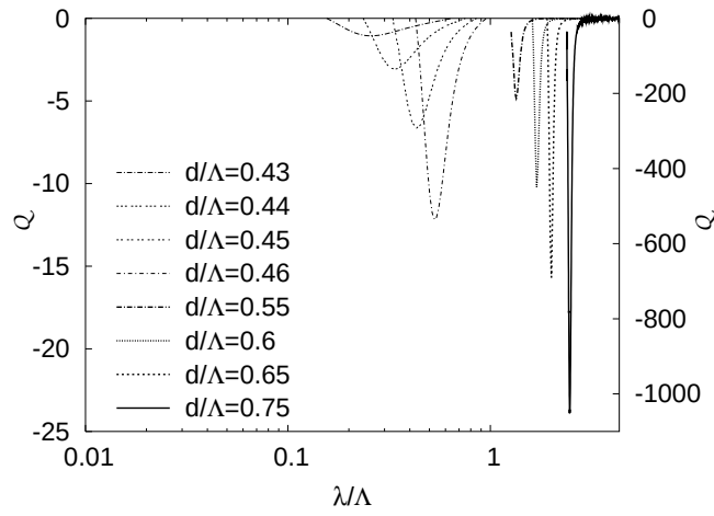
FIG. 3.14 – Q as a function of the normalized wavelength \lambda/\Lambda for eight d/\Lambda ratios for a 7-ring MOF made from a high index matrix ( n_{\text{mat}} = 2.5 ) with \Lambda = 2.3 \mu\text{m} . The thin curves (left) are associated with the left-hand y -scale (lowest d/\Lambda and |Q| values), while the thick curves use the right y -scale.
