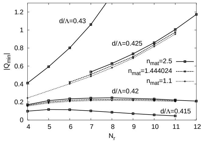
FIG. 3.16 – |Q_{\min}| as a function of N_r for three values of the matrix index n_M = n_{\text{mat}} , for several close d/\Lambda values.
