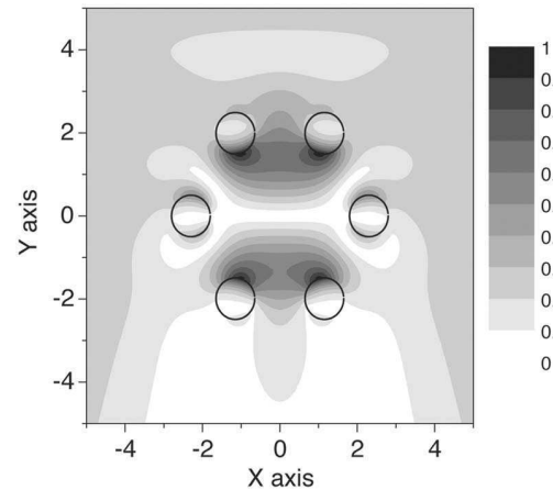
Fig. 17. Normalized |E_z| field map obtained thanks to the partial excitation (see Fig. 19 for the complete excitation) of the MOF fundamental mode belonging to the C4 symmetry class ( \theta_{\text{inc}}=0^\circ ). The studied fiber is the same as in Fig. 14.
