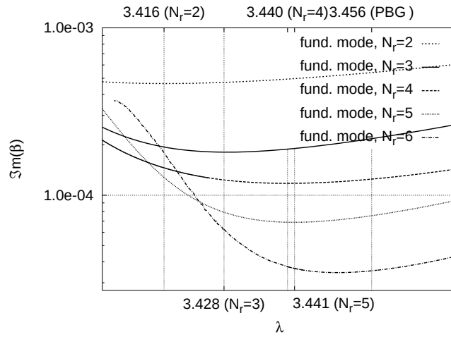
FIG. 3.36 – Losses \Im m(\beta) of the fundamental mode of several finite size MOFs ( N_r = 2, 3, 4 , and 5 ) versus the wavelength (note the y log-scale). The wavelengths of the different finite structures associated with the lowest losses \lambda_{opt} are materialized with vertical lines. The wavelength corresponding to the middle of the photonic bandgap (PBG) of the infinite lattice \bar{\lambda}_{gap} is also shown.
