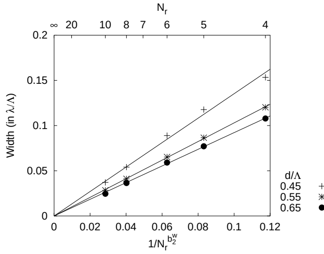
FIG. 3.12 – Width of the cutoff of the second mode as a function of the number of rings for three different values of d/\Lambda . The depicted quantity is the half-width of the \mathcal{Q} peak as a function of N_r^{-b_2^w} . Here b_2^w \simeq 1.55 . The width of the cutoff transition clearly goes to zero as the number of rings increases.
