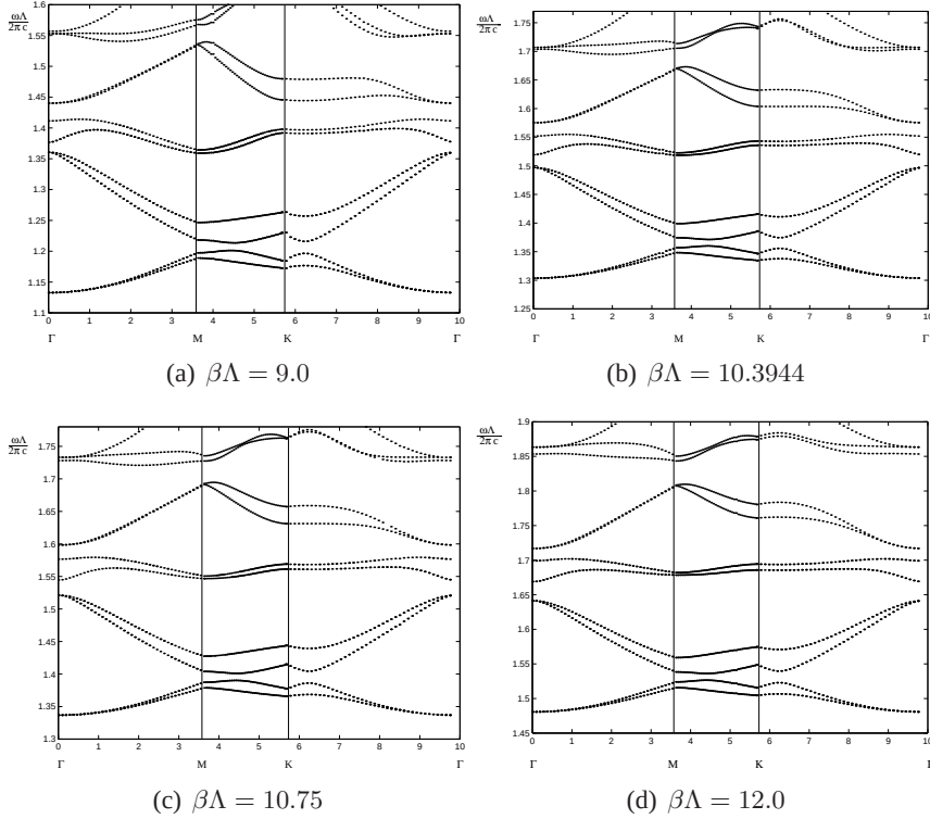
FIG. 3.33 – Dispersion curves of the Bloch waves associated with a triangular lattice of circular cylindrical inclusions ( n_i = 1.0 ) in an infinite silica matrix ( n_M = 1.39 ). The geometrical parameters are : \Lambda = 5.7816 \mu\text{m} , inclusion diameter d = 4.026 \mu\text{m} . These curves have been obtained for an out-of-plane propagation, i.e. \beta \neq 0 . The x -axis is associated with the route of the transverse wave vector along the edge of the irreducible Brillouin zone (see Appendix B.1.3 page 201). The y -axis represents the normalized frequency \omega\Lambda/(2\pi c) in which \omega is the frequency (angular) and c is the speed of light in vacuum.
