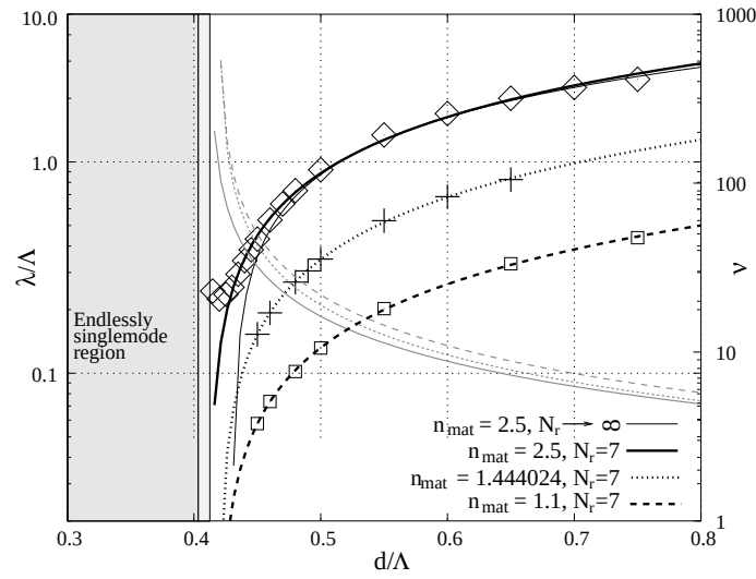
FIG. 3.17 – Phase diagram for the second mode. The points correspond to the computed values of (\lambda/\Lambda)_{\text{S.M.}} for the three matrix indices for N_r = 7 ; the thick black curves to the fits. The thin solid black curve is associated with the fit of the extrapolated results for N_r \rightarrow \infty computed for n_{\text{mat}} = 2.5 . The grey region is the approximate "endlessly" single mode region valid for the three matrix indices for N_r \geq 7 . Grey curves (right-hand scale) show the value of \nu at cutoff for the same refractive indices as the corresponding black curves.
