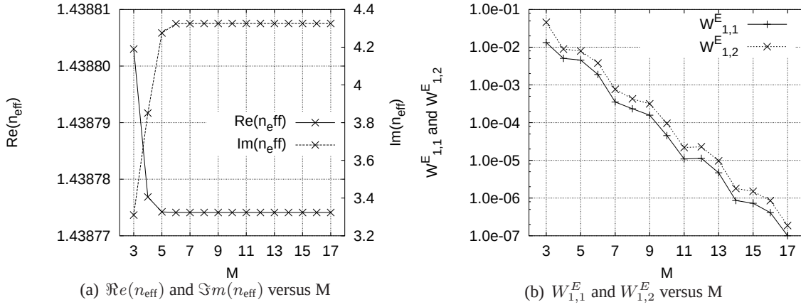
FIG. 2.12 – Convergence of n_{\text{eff}} and of W^E with respect to M . The data are the same as in table 2.2. ( 1.0e - 0N means 1.0 \times 10^{-0N} ).
