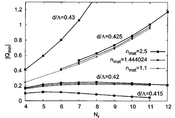
Fig. 3. |Q_{\text{min}}| as a function of N_r for three values of matrix index n_{\text{mat}} for several close d/\Lambda values.
