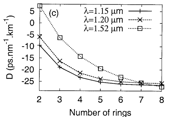
Fig. 5. (a) Dispersion and (b) losses as a function of the wavelength, and number of rings N_r [the types of curves have the same values for (a) and (b)]. Pitch \Lambda 2.0 \mu\text{m} ; hole diameter d , 0.5 \mu\text{m} . (c) Dispersion for three wavelengths as a function of the number of rings N_r for the same MOF.
