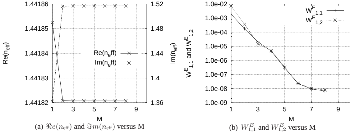
FIG. 2.13 – Convergence of n_{\text{eff}} and of W^E with M , the MOF is the same as in Fig. 2.12 except that the hole diameters are equal to 1.5 \mu\text{m} . ( 1.0e - 0N means 1.0 \times 10^{-0N} )
