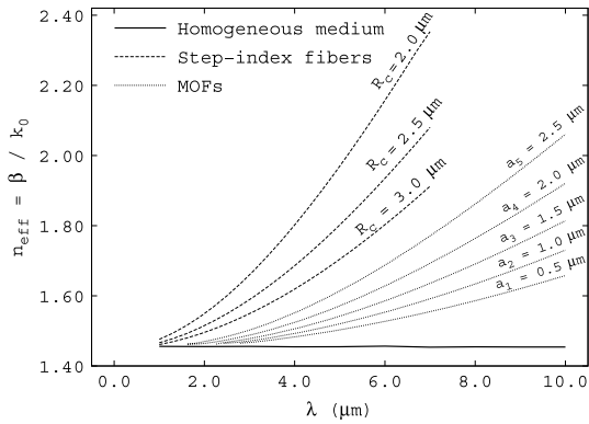
Figure 7. Comparison of the nonlinear effective index of the spatial soliton versus the wavelength in different nonlinear waveguides and in a homogeneous nonlinear medium. The solid core MOFs studied have four rings of air holes with various radii a and \Lambda = 6.0 \mu\text{m} . The index contrast of the step-index fibres with various core radii fulfils the WGA.
