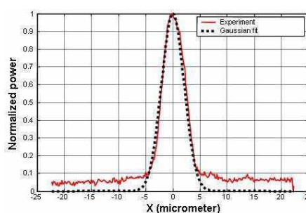
Fig. 3. (b) experimental Mode Field Diameter measurement
