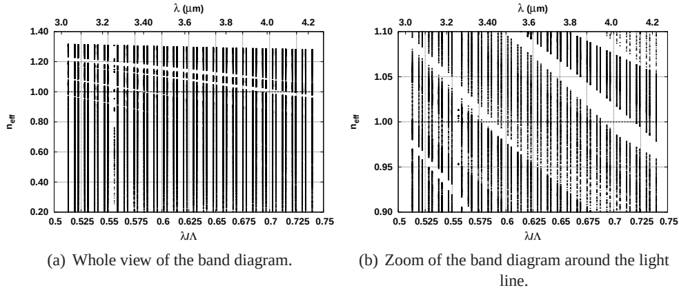
FIG. B.6 – Computed Band diagram of a triangular lattice of circular inclusions of low refractive index n_{cyl} = 1 in a high refractive index matrix n_{mat} = 1.39 . The white region represent the parameter space in which no modes can propagate in the periodic structures, i.e. full finite photonic bandgaps.
