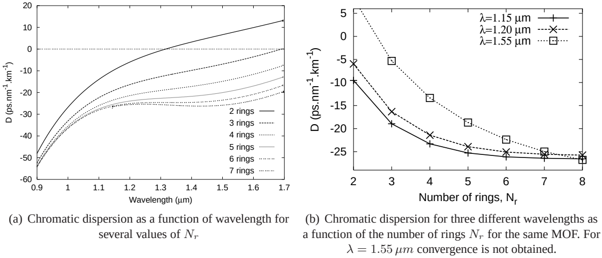
FIG. 3.27 – Chromatic dispersion as a function of the number of rings N_r . Pitch \Lambda = 2.0 \mu\text{m} ; hole diameter d = 0.5 \mu\text{m} .
