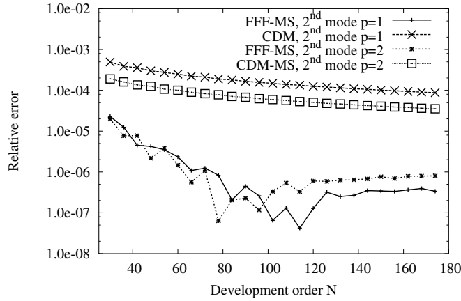
FIG. 2.35 – Comparisons of the effective index relative error versus the Fourier expansion order N , for the higher modes of symmetry classes p = 1 and p = 2 with the highest effective index real part. The results for the FFF-MS and the CDM-MS are shown. The studied MOF is the six-hole test MOF described in the text.
