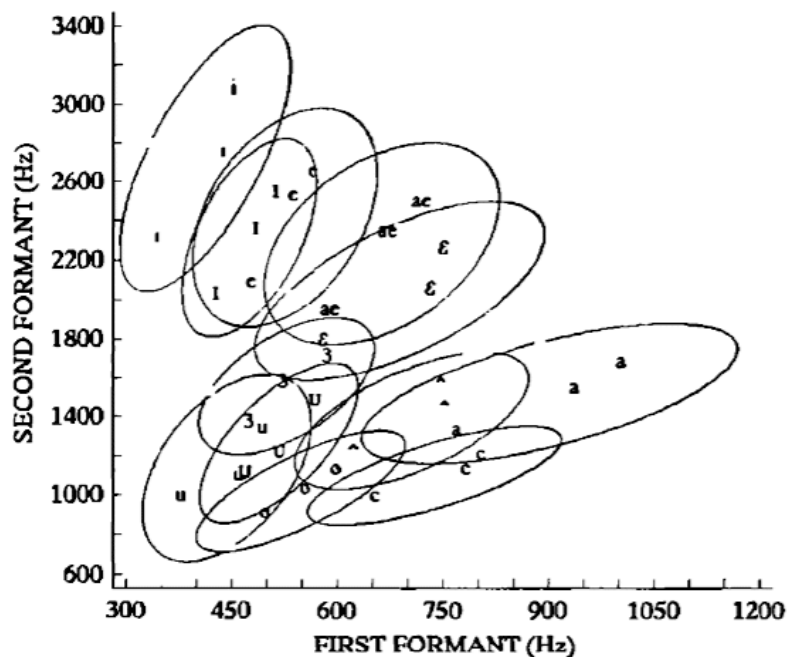
FIG. 3. Average values of F1 and F2 for men, women, and child talkers for 12 vowels with ellipses fit to the data ("æ"=/æ/, "ɑ"=/ɑ/, "ɔ"=/ɔ/, "ʌ"=/ʌ/, "ɝ"=/ɜ:/).
