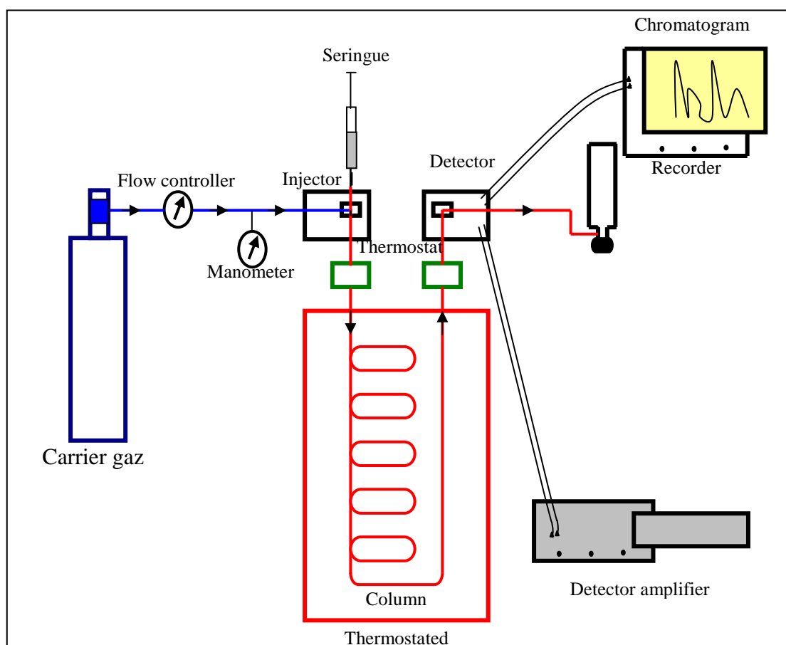
Figure 33: Gaz chromatography.
