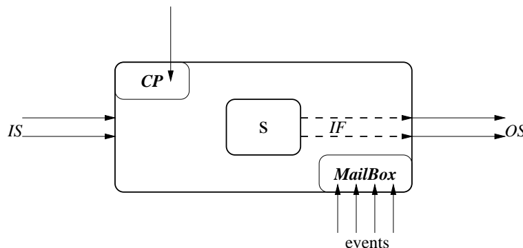
FIG. 2.17 – HPTS : architecture
