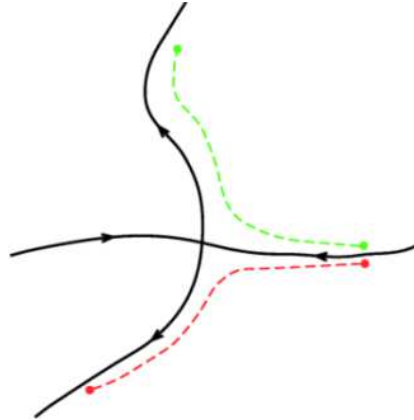
Figure 2.8: Two points on either side of a separatrix will diverge from each other. The quasi vertical separatrice is equivalent to the unstable manifold, whereas the quasi horizontal separatrice represents the stable manifold. The intersection between the two black lines is the hyperbolic point.
