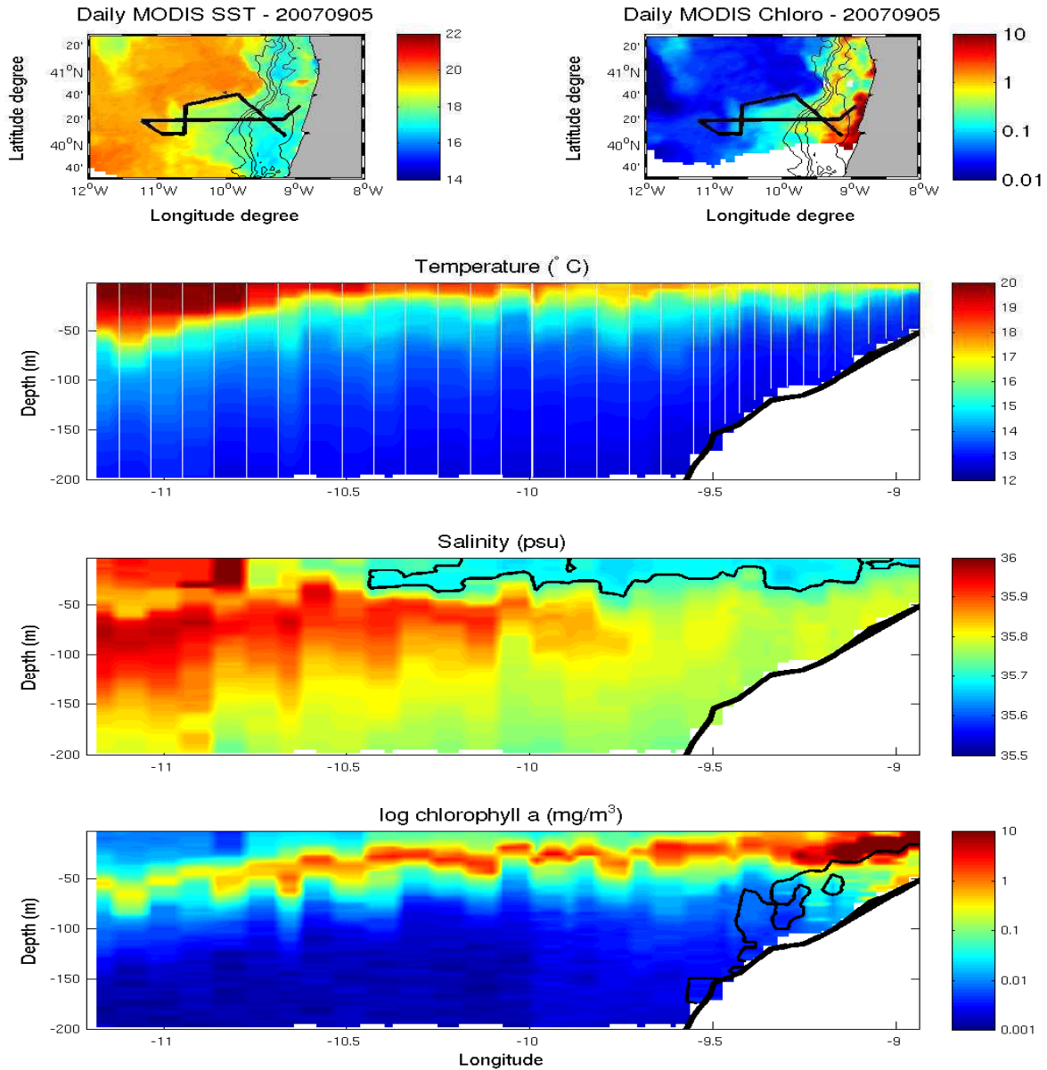
Figure 18: Two upper vignettes: SST ( ^{\circ}C ) and chlorophyll a concentration ( mg/m^3 ) from MODIS Aqua over the central IPUS on the 05/09/2007. The black thick lines superimposed represent the filament network performed. Three lower panels: longitude versus depth sections of CTD sensors for the EW transect inside the filament (temperature in ^{\circ}C , salinity (psu) and chlorophyll a concentrations from the fluorometer converted in mg/m^3 ). The black line in the chlorophyll a section indicates the minimum of dissolved oxygen concentration ( < 200 \mu mol/kg ). The black line in the salinity section contours the WIBP plume ( < 35.7 psu). The white vertical lines indicate the measurement positions; thick black lines represent the observed bathymetry.
