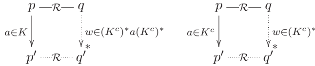
FIG. 1.3 – Relation de (bi)simulation.
