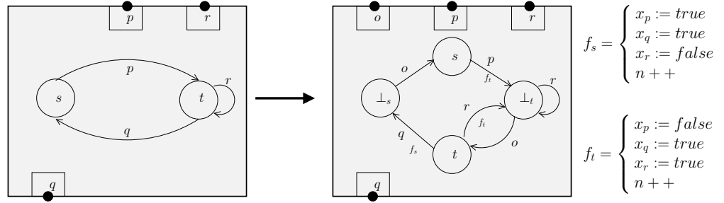
Figure 5.9: Transformation of atomic component.
