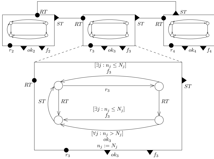
Figure 5.12: Token-based Conflict Resolution Protocol for the BIP models in Figures 5.1 and 5.8.
