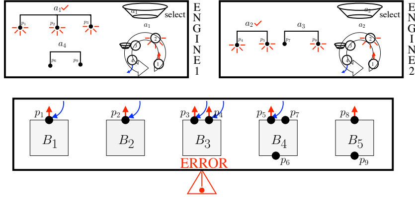
Figure 5.3: Violating BIP semantics when badly distributed interactions.
