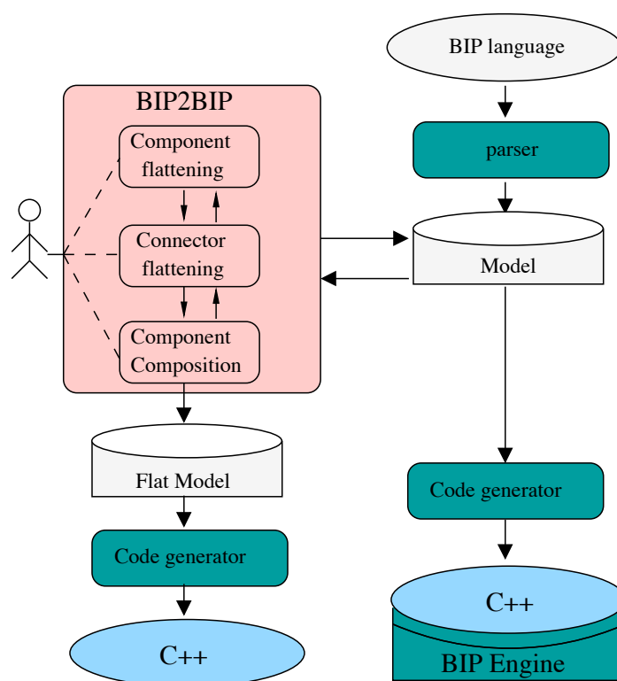
Figure 6.1: BIP2BIP toolset: General architecture
