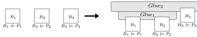
Figure 3.4: Composability of composition.
