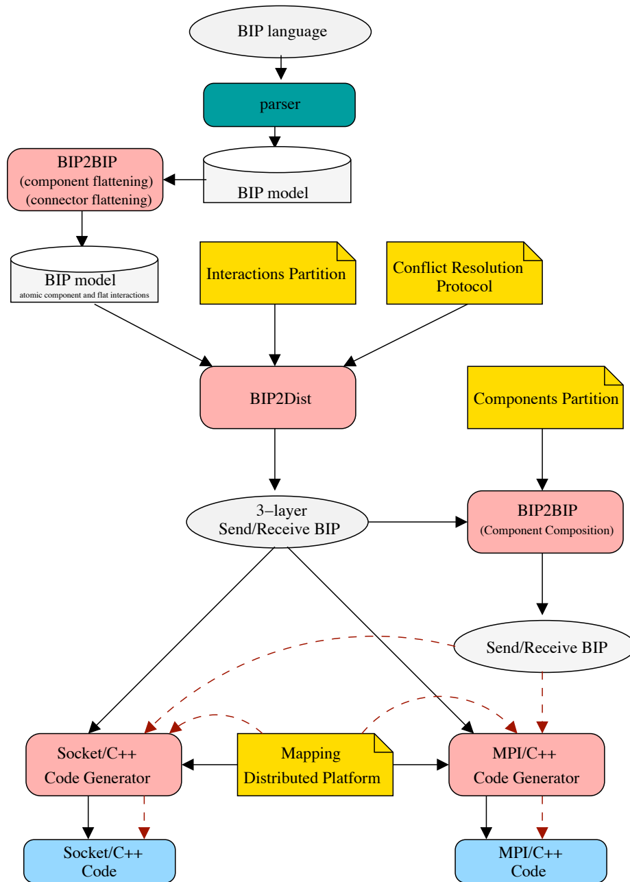
Figure 6.2: BIP2Dist toolset: General architecture
