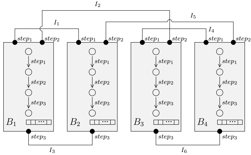
Figure 5.24: High-level BIP model for Bitonic Sorting Algorithm.
