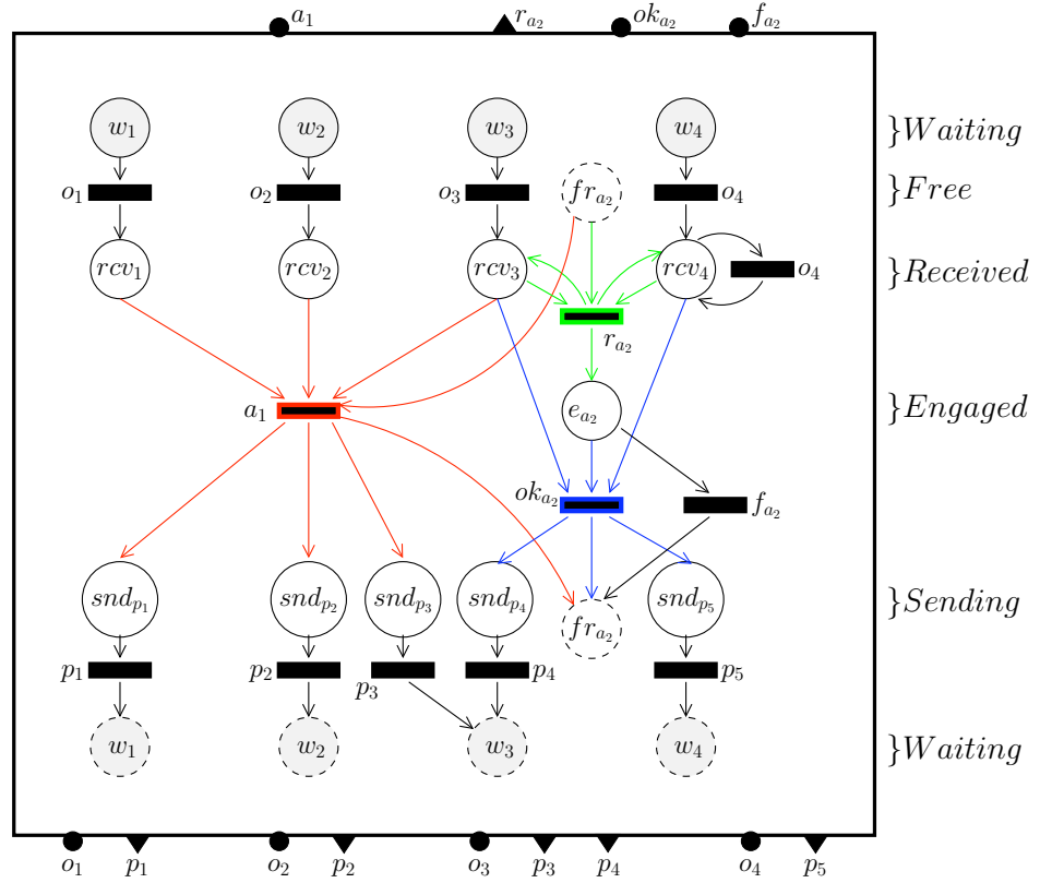
Figure 5.10: Component IP_1 in Figure 5.8.
