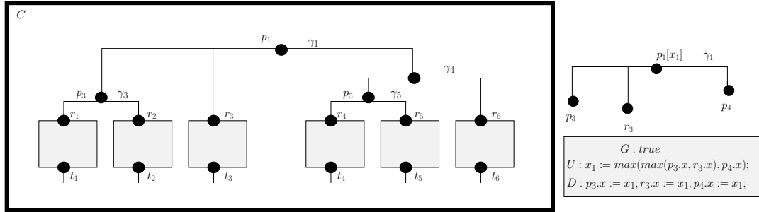
Figure 4.5: Connector glueing for example in Figure 4.3.
