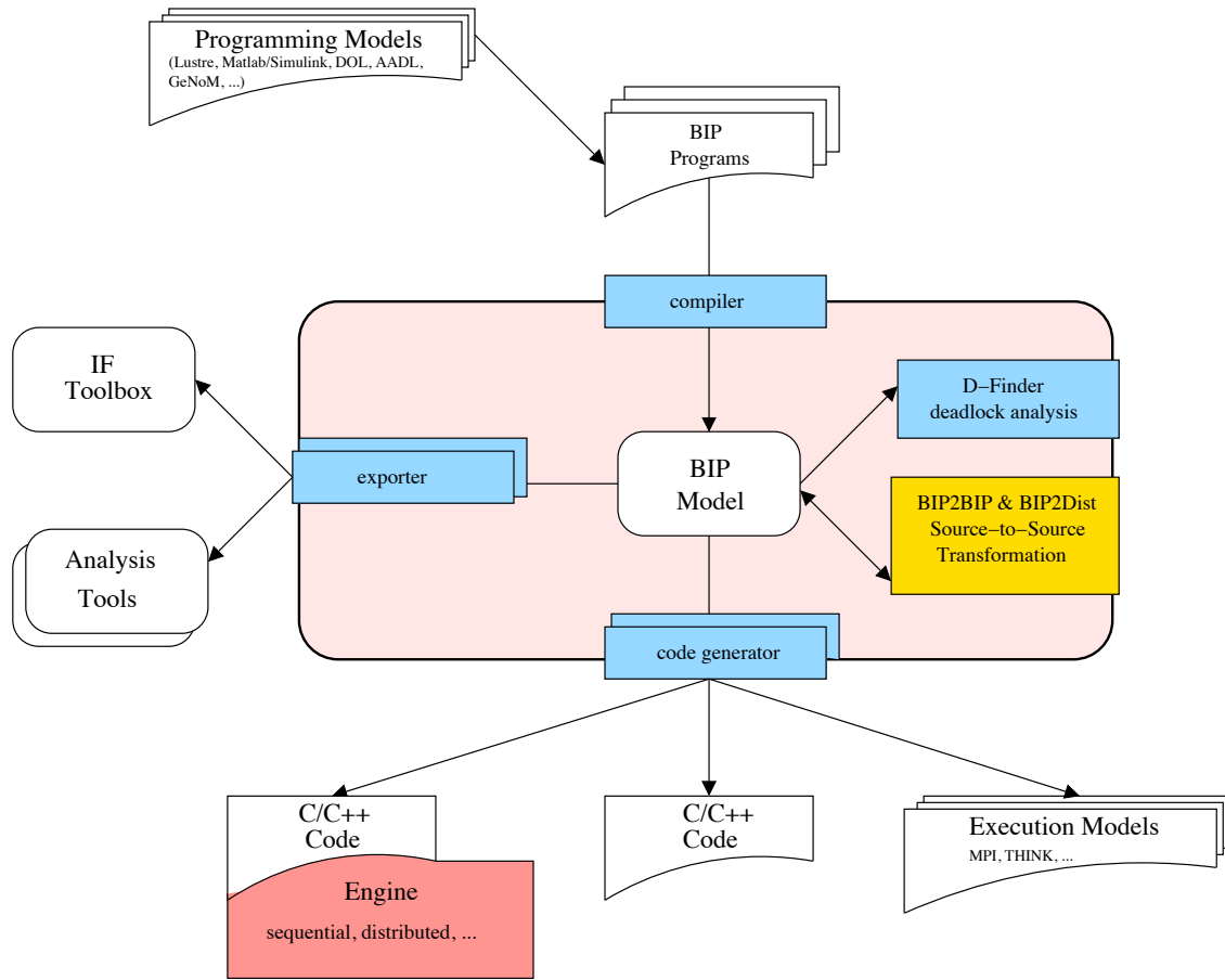
Figure 3.14: The BIP tool-chain.
