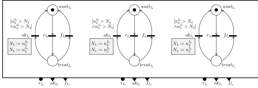
Figure 5.11: A centralized Conflict Resolution Protocol for Figure 5.8.
