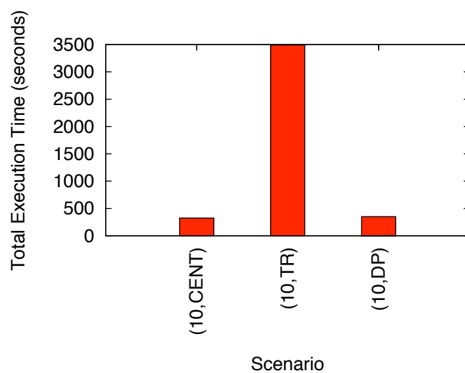
Figure 5.19: Performance of termination detection in diffusing computation in different scenarios (Torus 20 \times 20 ).
