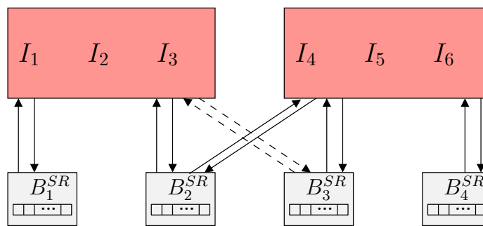
Figure 5.25: 3-layer Send/Receive BIP model for Bitonic Sorting Algorithm.
