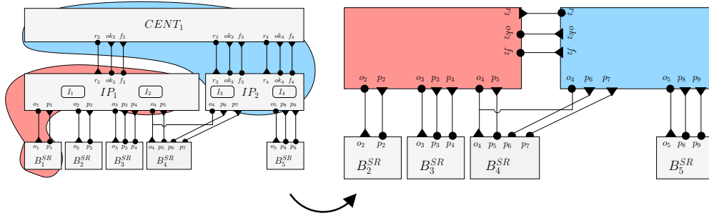
Figure 5.15: The impact of merging components.
