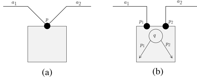
Figure 5.3: Violating BIP semantics when badly distributed interactions.
