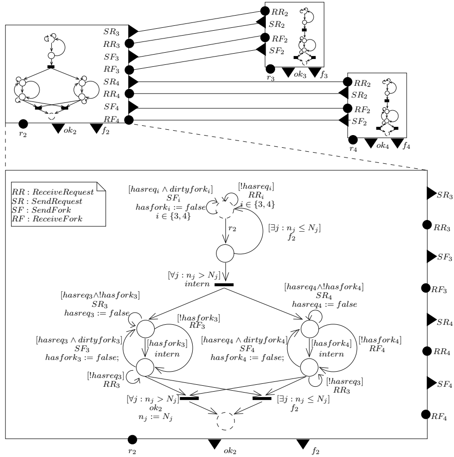
Figure 5.13: Dining philosophers-based Conflict Resolution Protocol for the BIP models in Figures 5.1 and 5.8.
