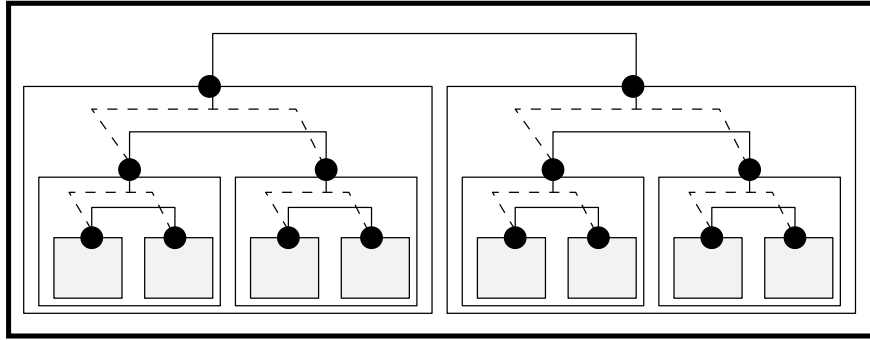
Figure 4.13: Concurrent sorting n = 4 .
