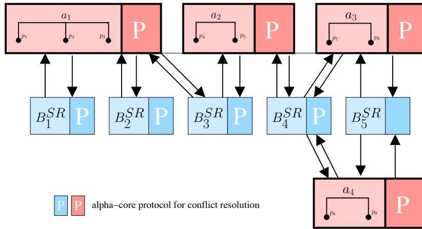
Figure 5.6: Resolving conflict interactions using alpha-core protocol.
