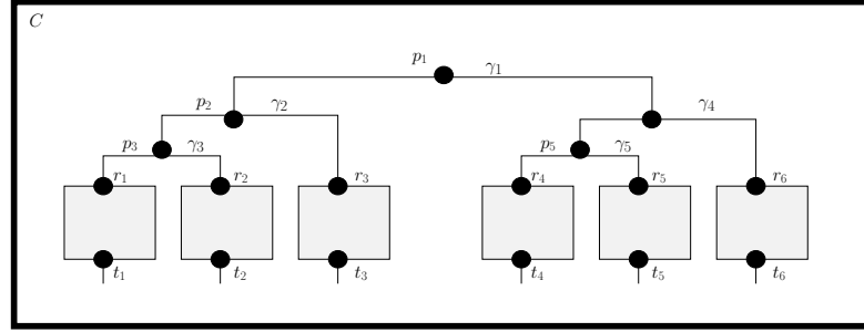
Figure 4.3: Component flattening for example in Figure 4.1.
