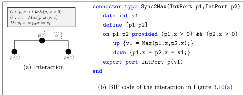
Figure 3.10: An example of a connector containing one interaction in BIP.
