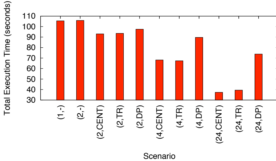
Figure 5.18: Performance of termination detection in diffusing computation in different scenarios (Torus 4 \times 6 ).
