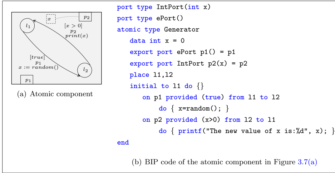
Figure 3.7: An example of an atomic component in BIP.
