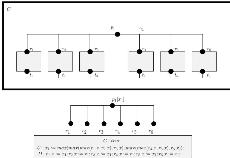
Figure 4.6: Connector flattening for example in Figure 4.3.
