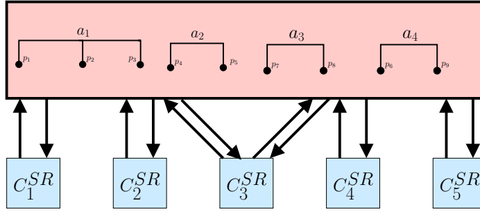
Figure 5.5: Drawbacks of conflict-free solution.
