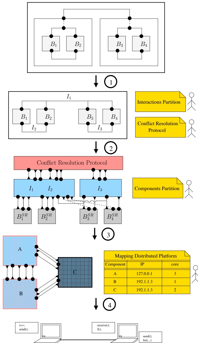
Figure 6.3: Design process to automatically generate distributed implementations
