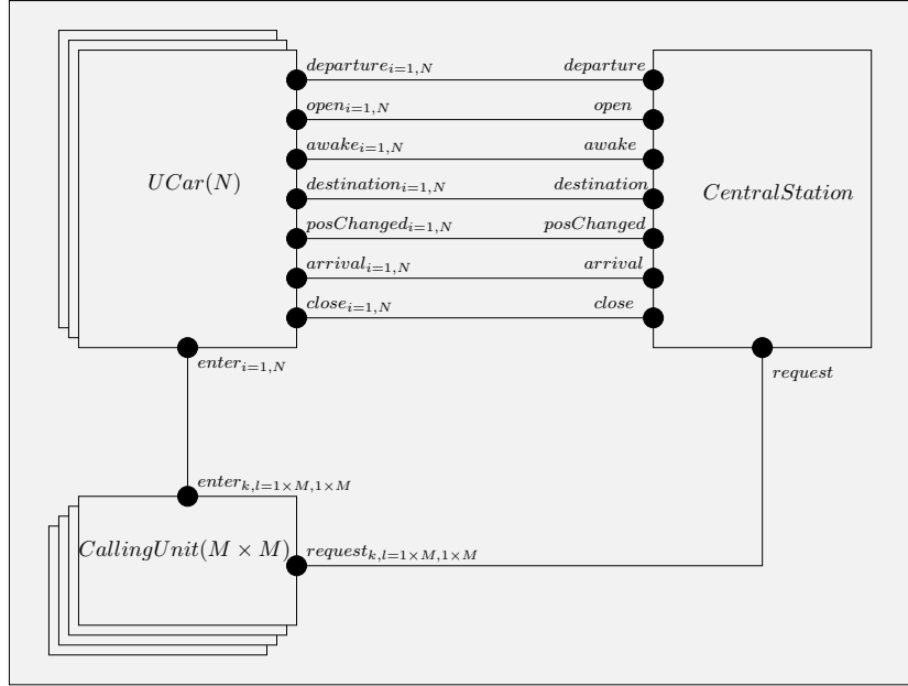
Figure 5.21: High-level BIP model for Utopar system.
