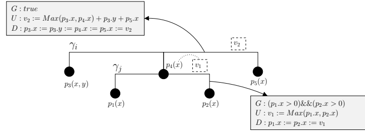
Figure 3.11: \gamma_i dominates \gamma_j .
