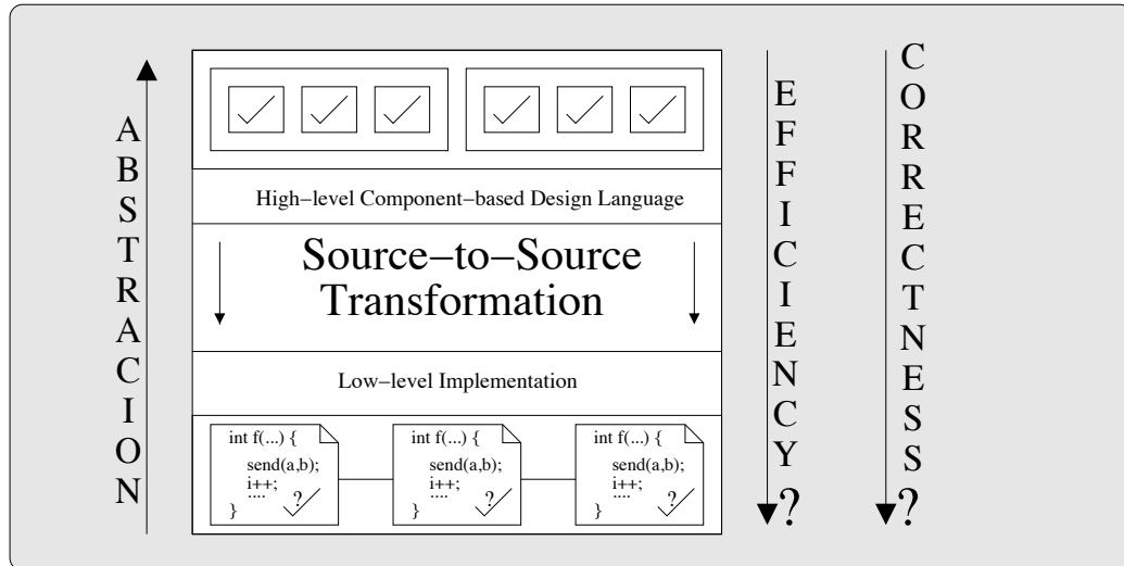
Figure 2.1: High-level component-based design into implementation.
