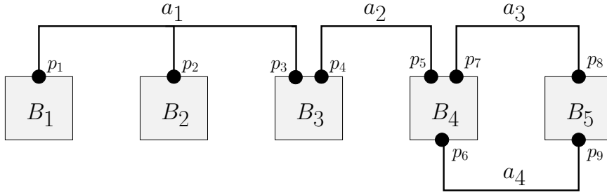
Figure 5.1: A simple high-level BIP model.
