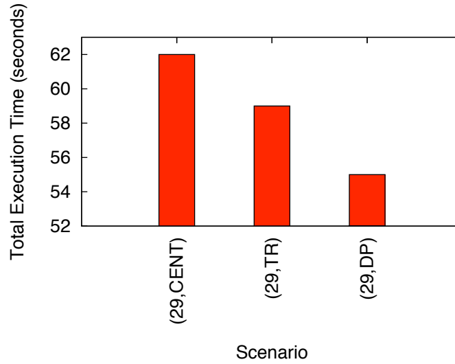
Figure 5.22: Performance of responding 10 requests per calling unit ( 25 = 5 \times 5 calling units, and 4 cars).
