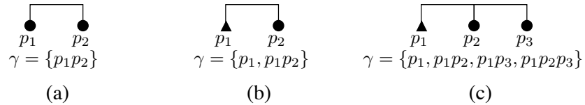
Figure 3.8: Connectors and their interactions.
