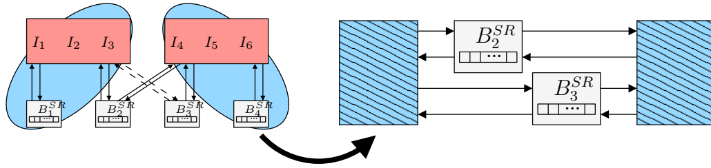
Figure 5.26: Component composition components in Bitonic Sorting 3-layer Send/Receive BIP model.
