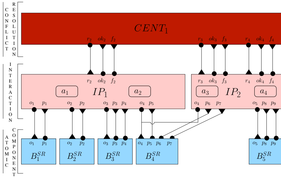
Figure 5.8: 3-layer Send/Receive BIP model of Figure 5.1.
