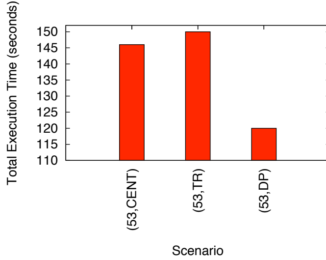
Figure 5.23: Performance of responding 10 request per calling unit ( 49 = 7 \times 7 calling units, and 4 cars).
