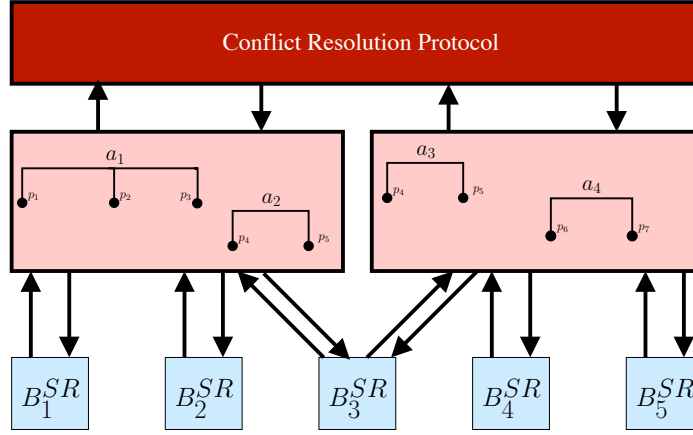
Figure 5.7: General overview of the 3-layer architecture.
