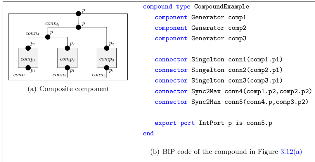
Figure 3.12: An example of compound component in BIP.
