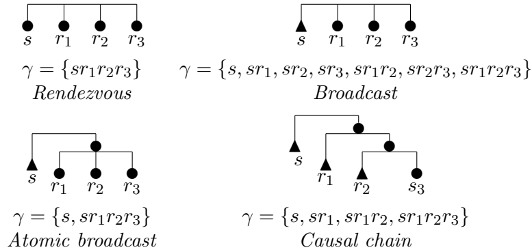
Figure 3.9: Graphic representation of connectors
