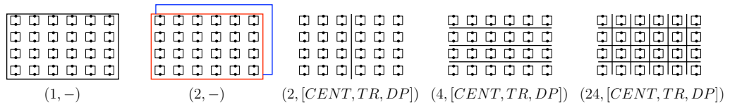
Figure 5.17: Different scenarios for diffusing computations.
