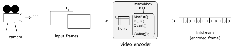
Figure 4.9: MPEG4 encoder structure.
