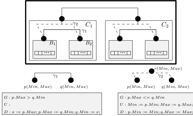
Figure 4.12: Concurrent sorting n = 2 .
