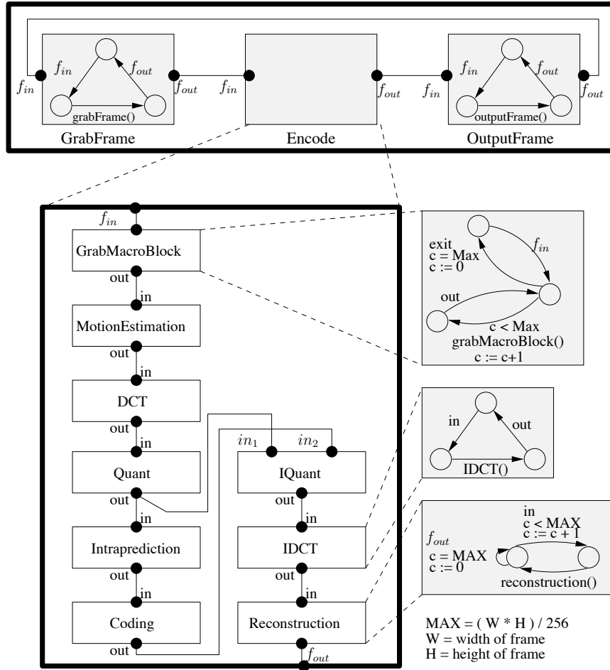
Figure 4.10: Encode component structure.
