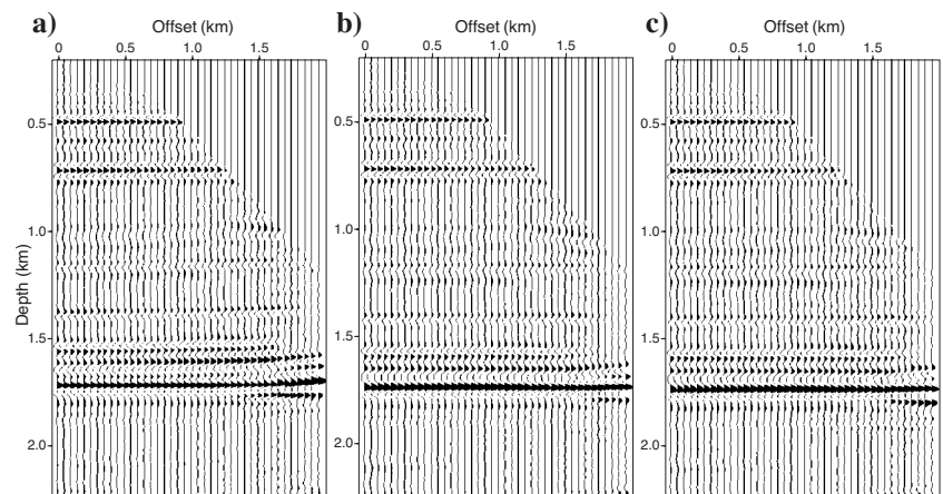
Figure 17. CIGs for x = 6800 m; (a) the initial velocity model v_{ini} , (b) the reference model v_{ref} , and (c) after prediction in the curvelet domain.
