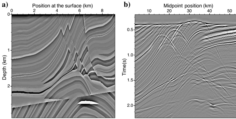
Figure 10. (a) Marmousi reflectivity model. (b) Associated ray + Born common-offset section (offset 600 m), generated in the exact velocity model v_{\text{ref}} (Figure 7a).
