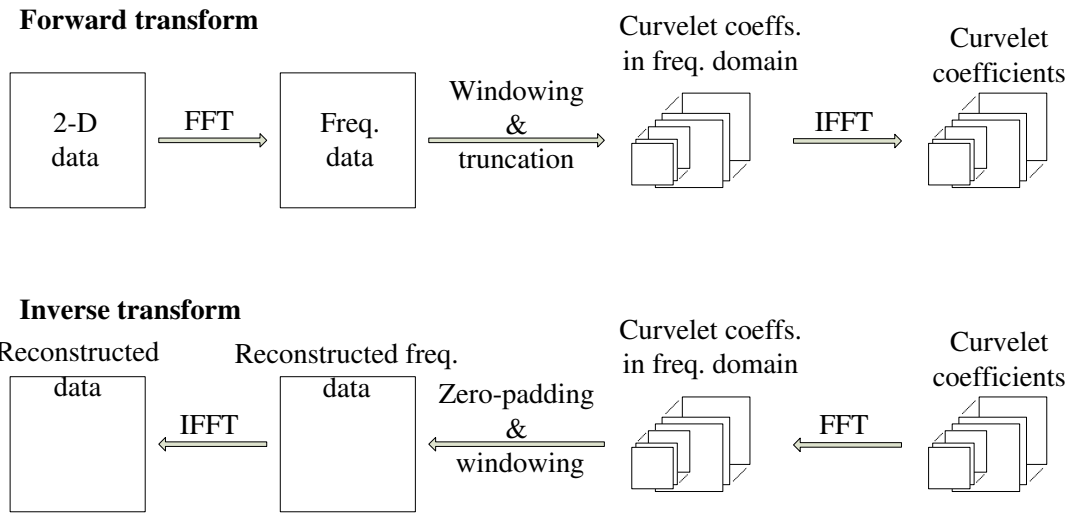
Fig. 4. Data flow structure of the FDCT forward and inverse transforms.
