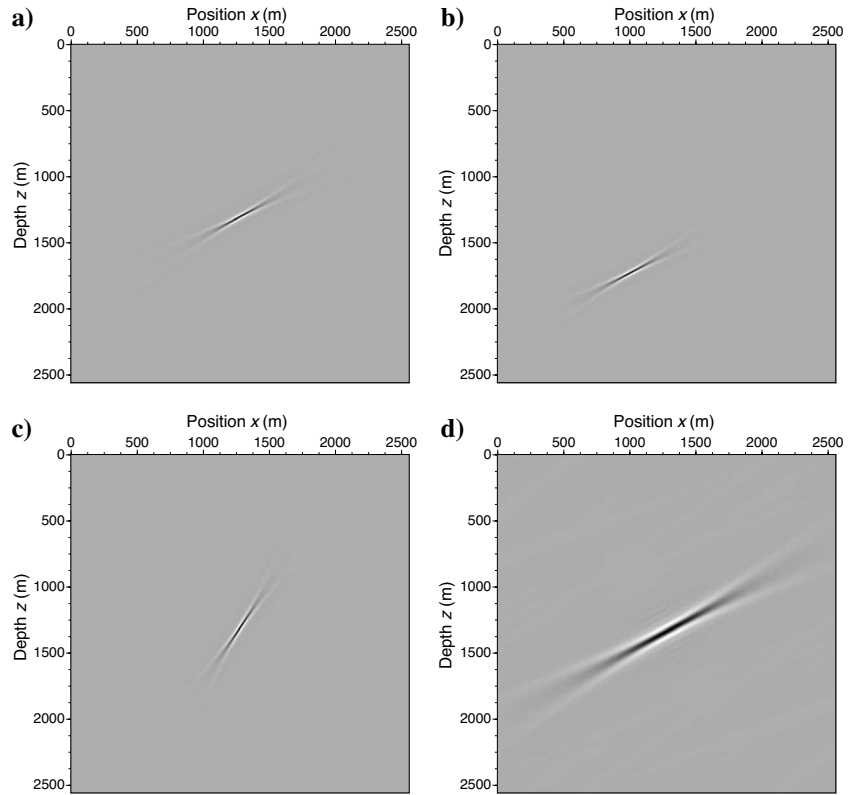
Figure 2. Curvelets in the spatial domain that can be deduced from (a) the reference curvelet by (b) translation, (c) rotation, and (d) dilation.
