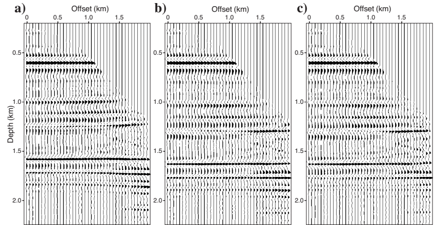
Figure 15. CIGs for position x = 6000 m; (a) initial velocity model v_{ini} , (b) the reference model v_{ref} , and (c) after prediction in the curvelet domain. The value v_{ref} corresponds to the exact velocity model.
