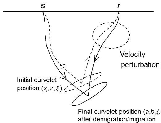
Figure 6. Illustration of image distortion. The migrated image is decomposed in the curvelet domain. Each curvelet is associated with a position (x_i, z_i) and a dip \tan \xi_i . It is first demigrated using the initial velocity model and remigrated in the perturbed velocity model.
