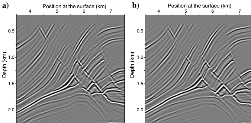
Figure 11. Kirchhoff common-offset section (for offset 600 m) migrated in (a) the initial velocity model v_{\text{ini}} and (b) the exact velocity model v_{\text{ref}} . The figure on the left is used as an initial image. The objective is to predict the image on the right, knowing v_{\text{ini}} and \delta v .
