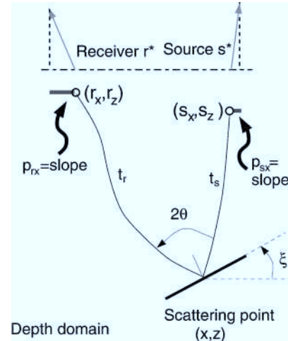
FIG. 9. In stereotomography (Billette and Lambaré, 1998), a general slope tomography method, the observed data consist of (s^*, r^*, t^*, p_s^*, p_r^*) , picked on seismograms. The model is given by the velocity model itself and the positions of the scattering points, defined by (x, z, t_s, t_r, \theta, \xi) . The cost function compares the characterized values at the extremities of the two ray segments from the scattering points to the data. In our method, the positions of the ray segment are automatically retrieved by migration, i.e., s_x = s^*, s_z = 0, r_x = r^*, r_z = 0, t_s + t_r = t^* . For migration at a common source, we also have p_{rx} = p_r^* . Only the slope at the source position may differ from the observed slope, providing a simpler cost function given by equation (36).
