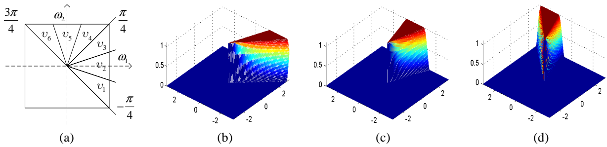
Fig. 8. (a) Essential supports of the angle functions v_i(\theta) as polar functions, and 3-D view of these polar function in the frequency plane, (b) 2-D angle functions v_1(\omega) , (c) 2-D angle functions v_2(\omega) , (d) 2-D angle functions v_3(\omega) .
