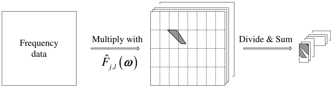
Fig. 17. Decimation in frequency domain of the UDCT. At each scale there are 2N_j windows, the first and second N_j data matrices are divided by D_{j,0} in (59) and D_{j,1} (60), respectively.
