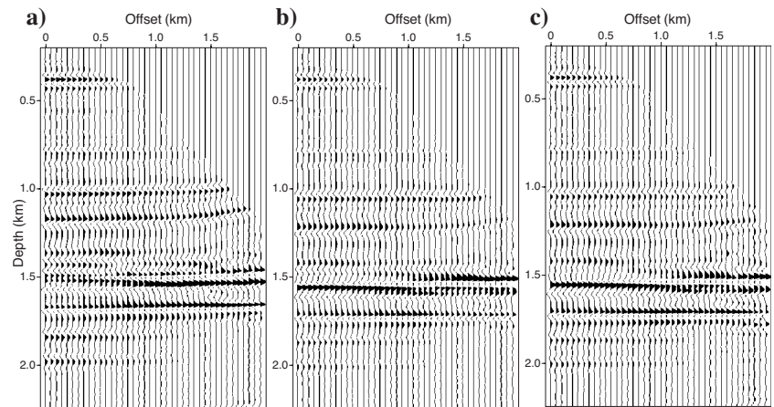
Figure 16. CIGs for x = 6400 m; (a) the initial velocity model v_{ini} , (b) the reference model v_{ref} , and (c) after prediction in the curvelet domain.
