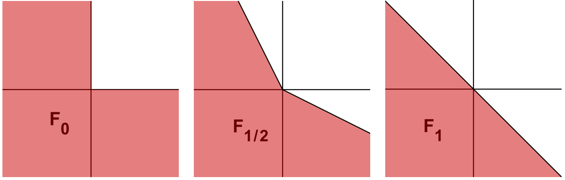
Figure 4.1: F_\beta for \beta=0, 1/2 and 1 in two dimensions
