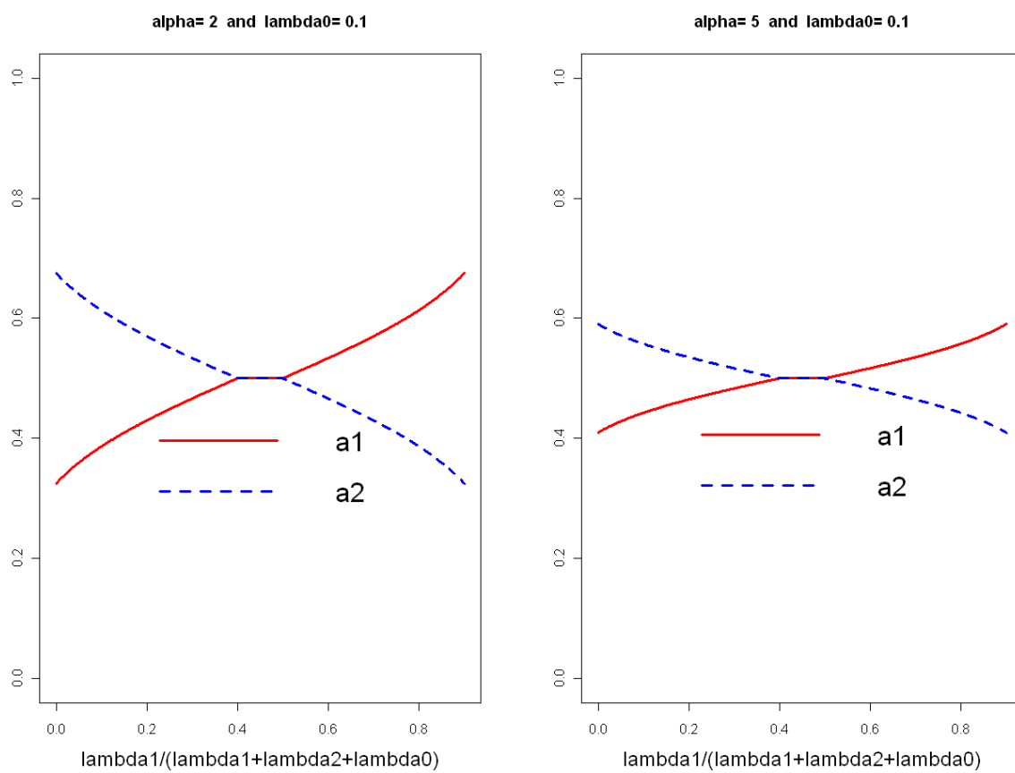
Figure 4.3: Optimal solution of the Case 2 for d = 2 and \lambda^{(0)} = 0.1
