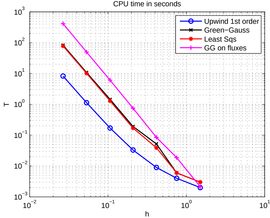
Figure 4.40: CPU time for different finite volume schemes.
