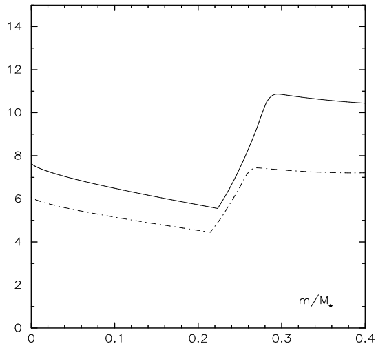
Fig. 8. Spitzer’s kinetic viscosity versus m/M_* , in the core of 3 M_{\odot} main sequence stars with X_c = 0.5 in two situations: SMC chemical composition (solid line) and Milky Way composition (dot-dashed curve).
