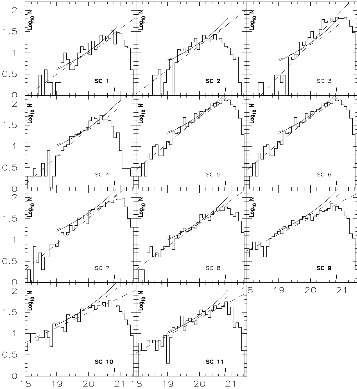
Fig. 2. Histograms : \log_{10} N (with N : number of objects within an I bin) versus I -magnitude for each of the 11 OGLE 2 fields towards SMC. Luminosity functions ( LF_{synth} ) are represented by dot-dashed lines for \alpha_{Salpeter} = 2.35 and by solid lines for \alpha = 2.85 . The dashed lines are fits to the histograms. Field labels are indicated, complete fields are in bold characters.
