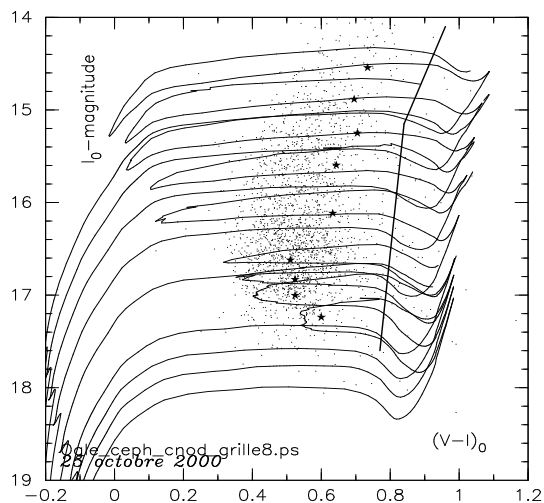
Fig. 3. Grid of evolutionary tracks with \alpha_{over} = 0.1 H_p , masses: 2.5, 2.65, 2.8, 3.0, 3.5, 4.0, 4.5, 5.0 and 5.5 M_{\odot} . “CA1” mixture of heavy elements. OGLE 2 data (dots) are fundamental and first overtone pulsators, the distance modulus is 18.94 from Laney & Stobies (1994), reddening and absorption are those given by OGLE for each cepheid. Locus where (\log T_{eff}, \log L/L_{\odot}) is read in the aim to establish “time average mass-luminosity relation are indicated by filled stars. Adopted red edge is plotted with help of broken line.
