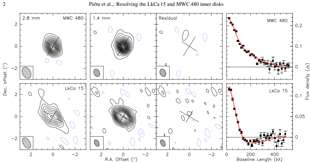
Fig. 1. Top row: Results for MWC 480. From left to right: 2.8 mm continuum image. The angular resolution is 1.09 \times 0.74 at PA 28^\circ , and the contour spacing is 1 mJy/beam (0.13 K, about 3.5\sigma ). The 1.4 mm continuum image: the angular resolution is 0.73 \times 0.53 at PA 33^\circ , and the contour spacing is 5 mJy/beam (0.33 K, 2.5\sigma ). The 1.4 mm residual from the best fit with the same contours. Right: 1.4 mm real part of the visibility vs baseline lengths. The points and error bars represent the measured values, and the curve indicates the visibilities of the best-fit disk model. The visibilities have been corrected from the disk orientation and inclination by compressing the V value by \cos(i) prior to circular averaging. Bottom row: Results for LkCa 15. The 2.8 mm image is obtained by considering baselines longer than 200 m (but no flux was lost in this process). The resolution is 1.06 \times 0.61 at PA 31^\circ , and the contour spacing is 0.75 mJy/beam (0.12 K, 2\sigma ). The 1.4 mm resolution is 0.66 \times 0.39 at PA 55^\circ , and the contour spacing is 1.5 mJy/beam (or 0.15 K, 1.7\sigma ). The crosses indicate the position, orientation, and aspect ratio of the disks.
