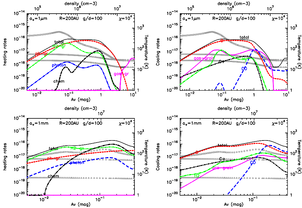
Fig. 9. Heating (left) and cooling (right) process for the models with small grains (top) and big grains (bottom) and a g/d ratio of 100 in \text{erg cm}^{-3} \text{s}^{-1} . H_2\text{-gr} is the heating due to H_2 formation on grains. ph\text{-gr} is the photoelectric effect on grain. photon is the direct heating of the gas by the photons and chem is the heating due to chemistry reactions (see text for details). Squares: gas temperature, triangles: upper and lower limit of dust temperature.
