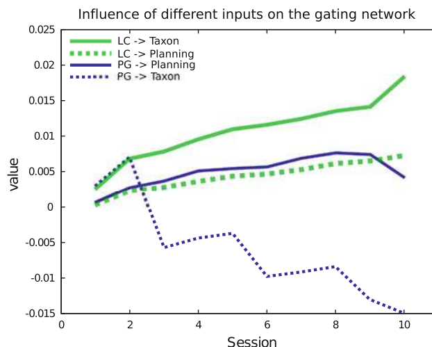
Fig. 11 Synaptic weights of the gating values in the gating network in Control group. Thick lines represent straight links (LC \rightarrow Taxon, PG \rightarrow Planning). Dotted lines represent cross links (LC \rightarrow Planning, PG \rightarrow Taxon)
