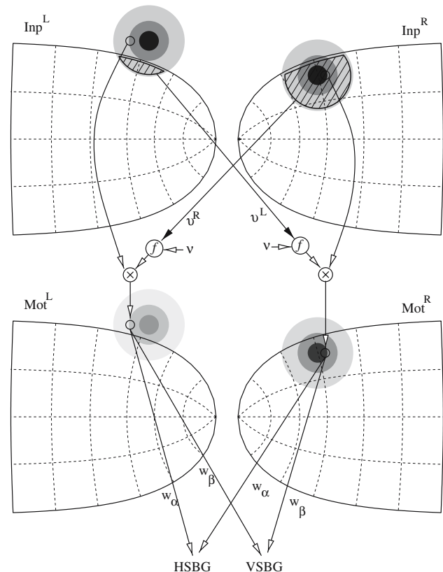
Fig. 2 Gluing method. A single target in the left hemifield but close to the vertical elicits activity in the input layers of both colliculi ( \text{Inp}^R and \text{Inp}^L ). In the motor layers ( \text{Mot}^R or \text{Mot}^L ) this activity is inversely modulated by the area of the contralateral activity within the boundary of its visual hemifield (hatched area, noted v^R and v^L ). Note that v is the sum of the activity of the whole shaded areas. In the motor layer, activity is, thus, much stronger in the right colliculus (coding the left hemifield) than in the left one. For a target further away from the vertical, there would be no activity left in the left motor layer. This distributed motor activity is the abstract \mathbb{R}^2 mapping assumed by the second property of our first proof, which can then be weighted, summed and sent to the horizontal and vertical SBG
