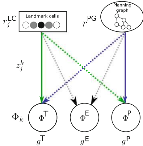
Fig. 3 Gating network. The inputs of the Taxon and Planning experts (LC and PG) are linked to the units in the gating network. The gating values g^k are weighted sums of the input values r_j with weights z_j^k . One of the three experts is selected according to a winner-take-all scheme
