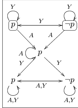
Figure 4.13: Internal model of type 2 associated to \{(M^r, w^r), (M^{r'}, w^{r'})\}
