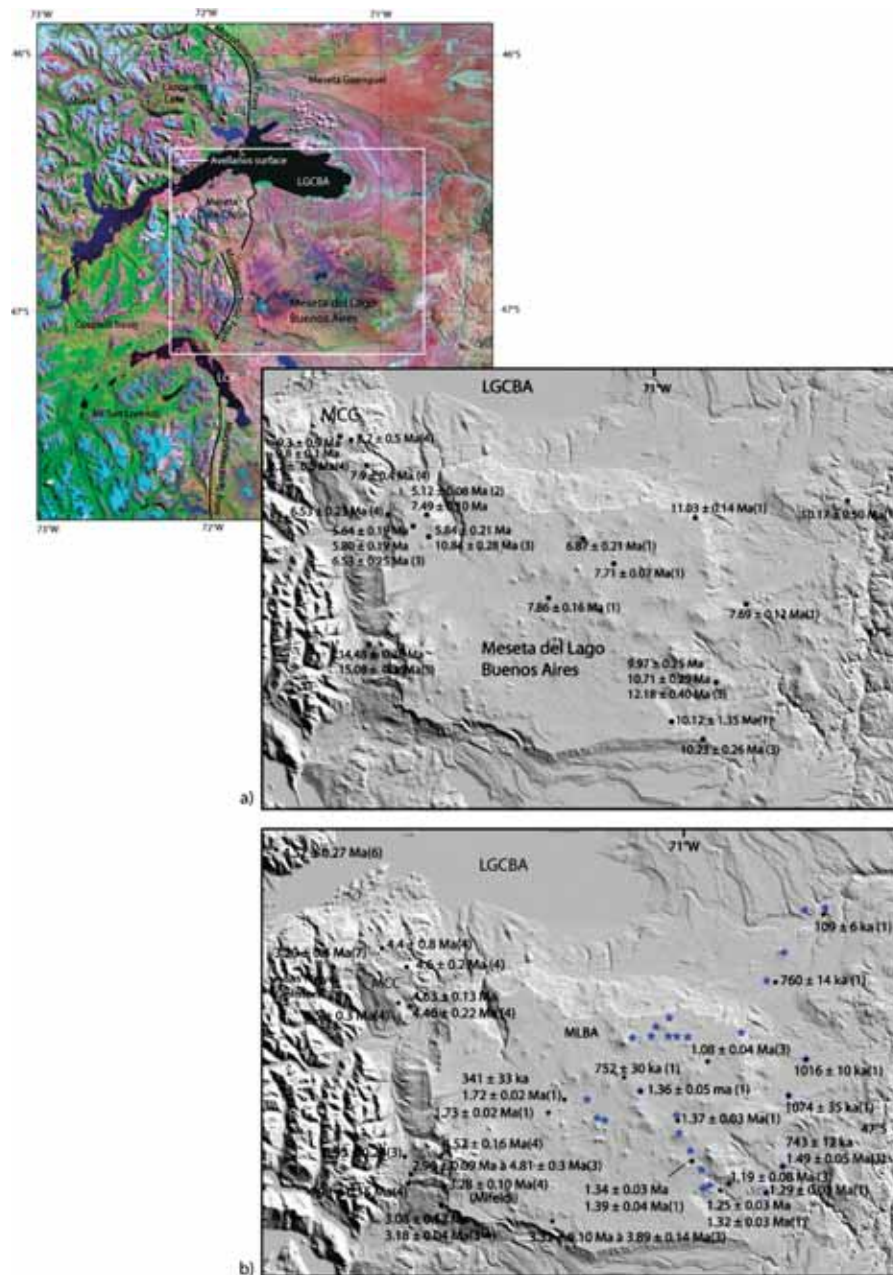
Fig. 5 Landsat 7 image of the internal part of Central Patagonia at the latitude of the Chile Triple Junction (see location in Fig. 4) and a compilation of published ages of volcanic rocks shown on a DEM of the Meseta del Lago Buenos Aires region (after Scalabrino et al., in preparation). Main Plateau (a) and Post Plateau (b) volcanics are shown separately. Black dots in Figure (a) correspond to dated samples. The origin of data is marked as numbers in brackets after each age, as follows: (1) Brown et al., 2004; (2) Mercer and Sutter, 1982; (3) Guivel et al., 2006; (4) Espinoza et al., 2005; (5) Espinoza, 2003; (6) Pelleter, 2003; (7) Suarez et al., 2000b. Grey stars in Figure (b) are the locations of the Pliocene-Pleistocene Post-Plateau lavas studied by Gorrington et al., (1997). LGCBA Lake General Carrera Buenos Aires, MLBA Meseta del Lago Buenos Aires, MCC Meseta Chile Chico
