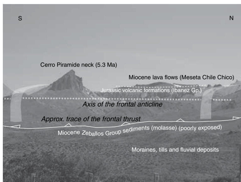
Fig. 6 The Cerro Piramide neck intruding the front of the Cordillera near Chile Chico (location Fig. 3).
