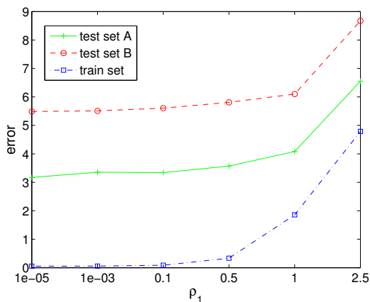
Figure 7.9: CoNLL 2003, \rho_2 = 0.001
