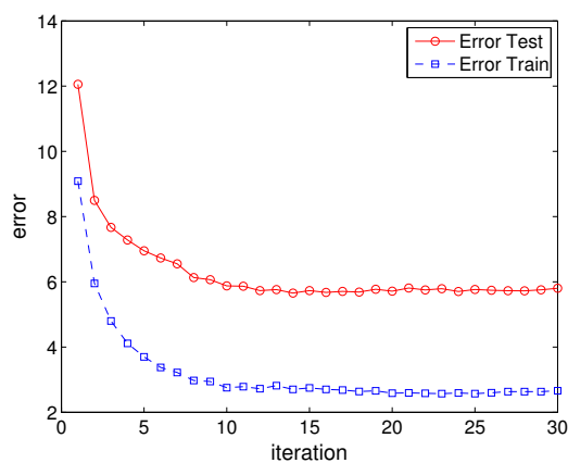
Figure 7.10: CoNLL 2000, error.
