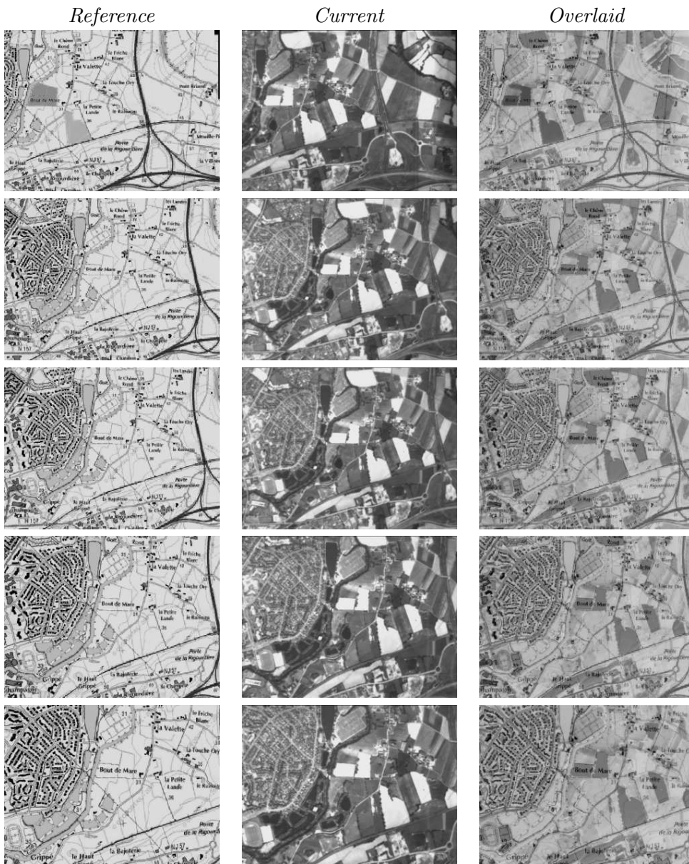
Figure 7.8: 6D Multi-modal MI-based visual servoing in a navigation task. The reference and resulting trajectories remain similar.
