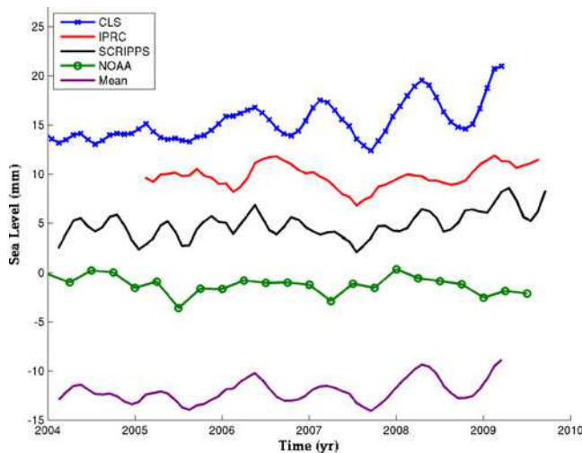
Fig. 9 Global mean steric sea level curves (seasonal signal removed) from CLS (blue curve), SCRIPPS (black curve) and IPRC (red curve) and NOAA (green curve) (left panel), and mean of SCRIPPS, CLS, and NOAA data (violet)
