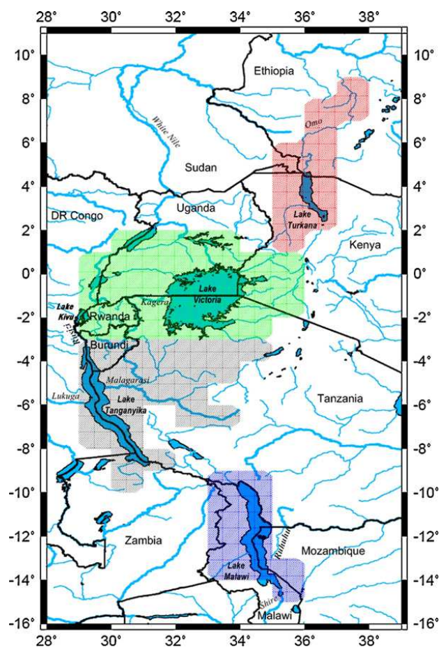
Fig. 1. Boundaries of the East African Great Lakes region. The lakes with their drainage basin selected for the study are: Lake Turkana (red), Lake Victoria (green), Lake Tanganyika (gray) and Lake Malawi (blue). The contours of the drainage basin were obtained from the drainage network provided by the model routing Total Runoff Integrating Pathways (TRIP, (Kundzewicz et al., 2004)).
