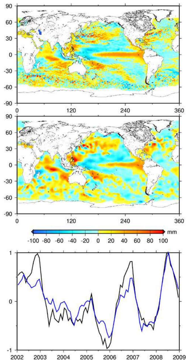
Fig. 6 EOF mode 2 spatial patterns of observed (upper panel) and steric-CLS data (middle panel) sea level. EOF mode 2 temporal curves (lower panel) of observed (black curve) and steric sea level (blue curve). Explained variances are 6% and 8% for observed and steric mode 2
