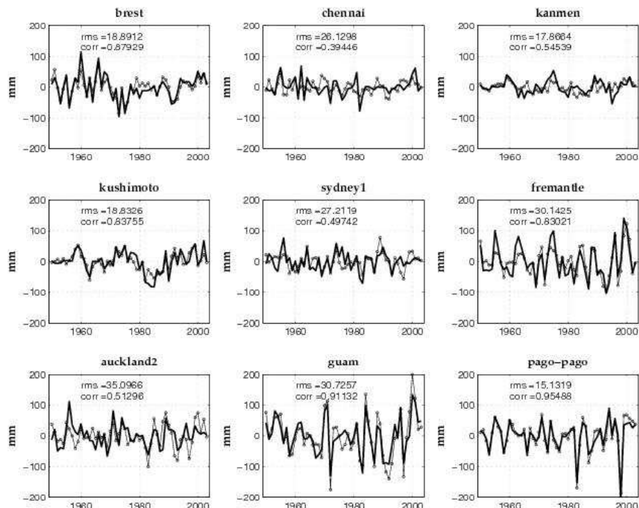
Fig. 7b. Same as (a) but with mean trend removed.
