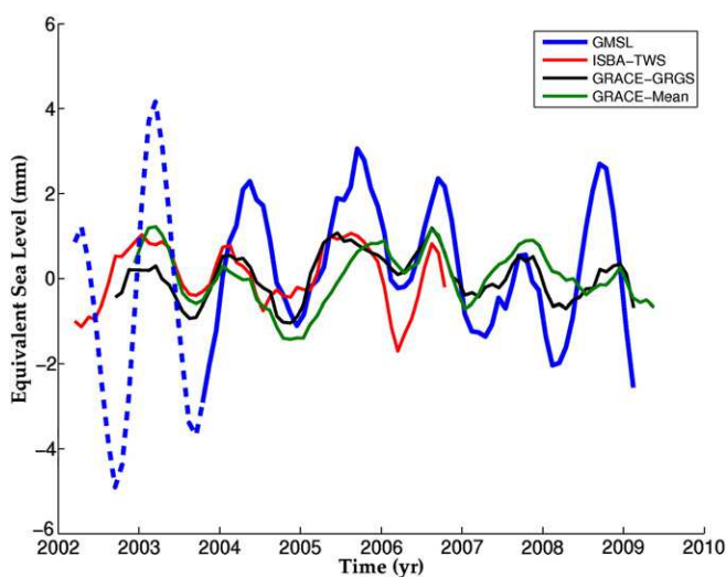
Fig. 2. Interannual variability of the altimetry-based global mean sea level (GMSL) corrected for thermal expansion over 2003–2009 (blue curve—data from Llovel et al., 2010b) and terrestrial water storage (expressed in equivalent sea level)—TWS-ESL from the ISBA-TRIP model (red curve) and GRACE (green curve: data from the mean CSR/GFZ/JPL; black curve: data from GRGS updated from Llovel et al., 2010a). The time series are detrended, and the seasonal cycle is removed. The time series are smoothed with a 3-month window.
