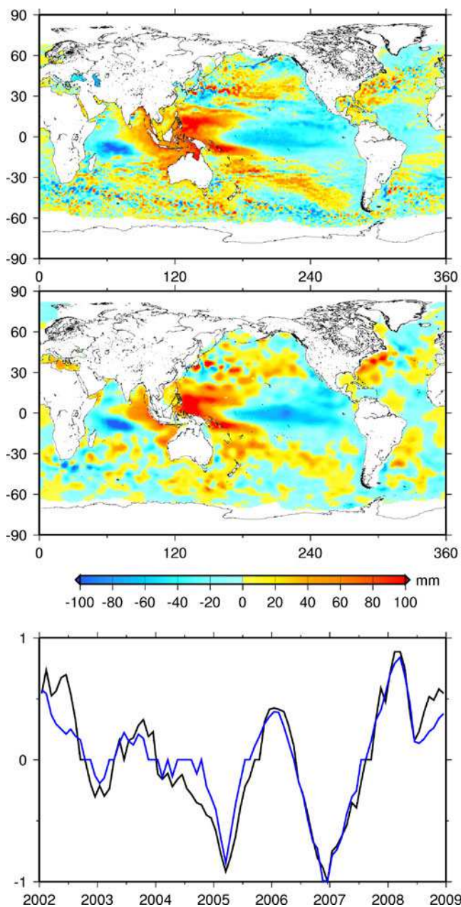
Fig. 5 EOF mode 1 spatial patterns of observed (upper panel) and steric-CLS data (middle panel) sea level. EOF mode 1 temporal curves (lower panel) of observed (black curve) and steric sea level (blue curve). Explained variances are 8% and 11% for observed and steric mode 1
