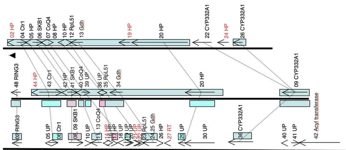
Fig. 1. Syntenic relationship at the CYP332A locus. Schemes at scale representing, from top to bottom, H. armigera , S. frugiperda , and B. mori . Arrows represent genes predicted by KAIKOGAAS. Only valid genes are shown (Fig. S1). Synteny links are shown with black dotted lines. In text boxes, gene ID, or for other genes, HP, unknown protein (UP; presence of a match to an EST with a threshold of 10^{-40} by BlastN). Synteny blocks (as defined in text) are shown as colored boxes spanning genes arrows in the case of H. armigera and S. frugiperda , below and above gene arrows in the case of S. frugiperda and B. mori , respectively. See Fig. S2 for gene name abbreviations.
