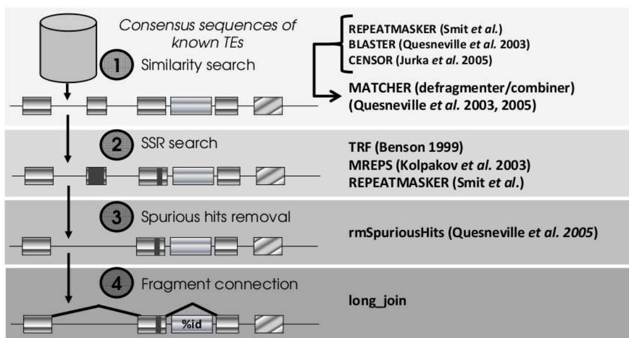
Figure 3: The four steps of the TEannot pipeline [22]
