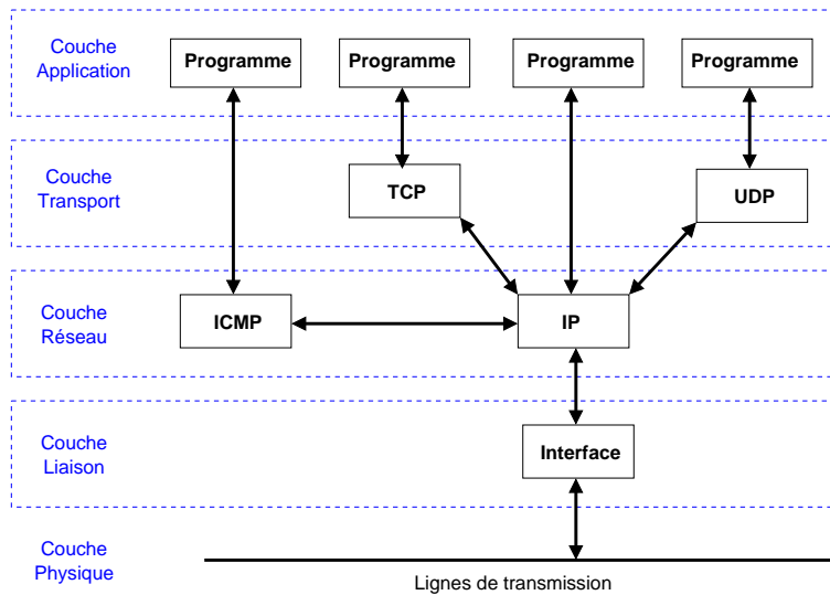
Figure C.1 – Architecture TCP/IP
