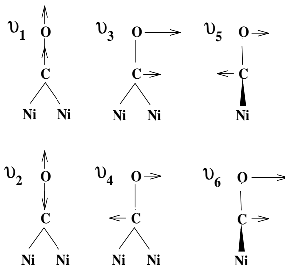
Figure 1.5: Normal modes of on-top and bridge-bonded CO (from Richardson and Bradshaw [47]).
