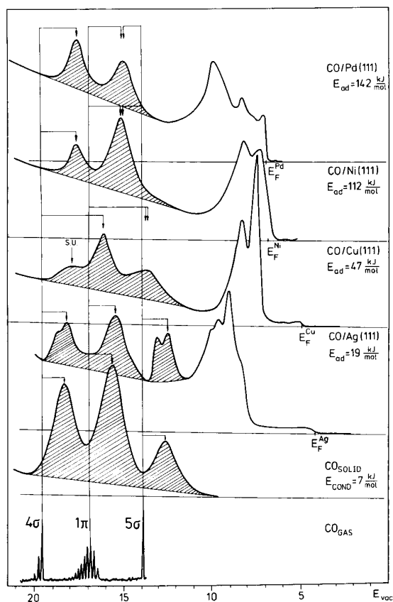
Figure 1.1: Different adsorbate systems in normal emission, the binding energy E_B = h\nu - E_{kinetic} is given with respect to the vacuum level E_{vac} (from [41]). One can see a shifting of ionization potentials and a broadening depending on the substrates.
