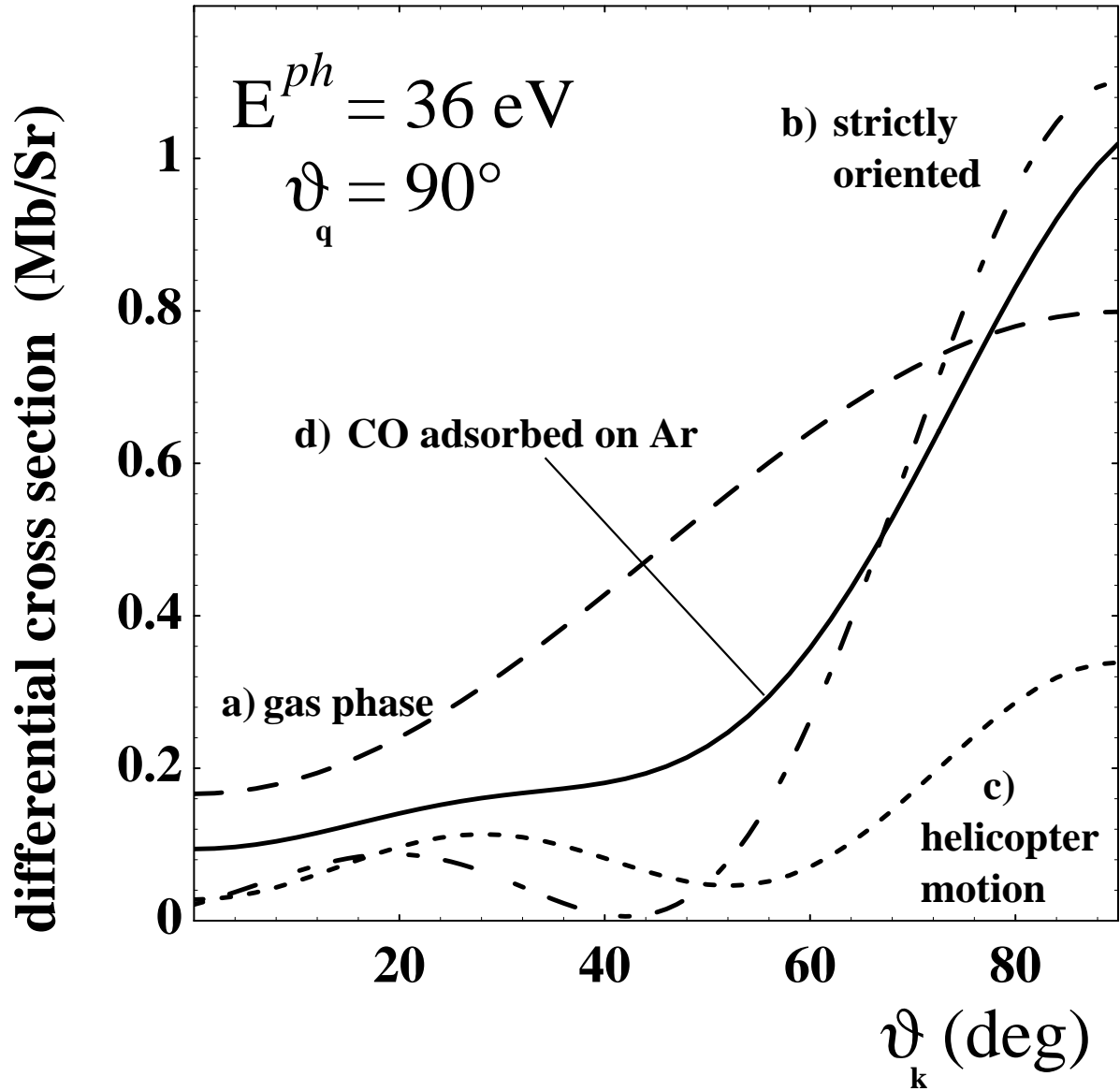
Figure 3.9: Angular distribution of photoelectrons emitted from CO/Ar in the case of B^2\Sigma_{1/2}^- \leftarrow X^1\Sigma_0^+ excitation. The photon is linearly polarized with \vartheta_q = 90^\circ , \varphi_q = 0^\circ and its energy is 36 eV. The electrons are emitted in the plane defined by the polarization vector of the light and the surface normal ( \varphi_k = 0^\circ ). Four models were considered: a) gas phase, b) 'oriented-in-space' (intensity scaled by a factor of 1/10), c) 'helicopter motion', d) hindered rotation model (from Büchner and Raşeev [11]).
