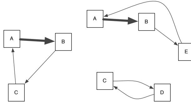
Figure 3.4: Sample SCC (Figure 3.3) decomposed into three minimal cycles.
