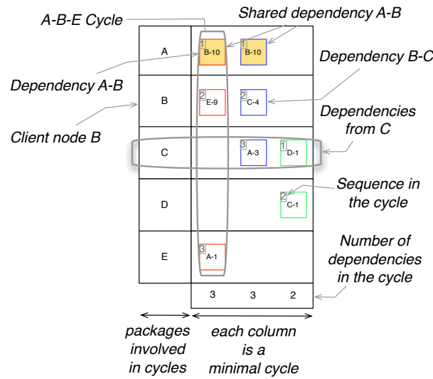
Figure 6.4: CYCLETABLE for Figure 6.1 sample graph.
