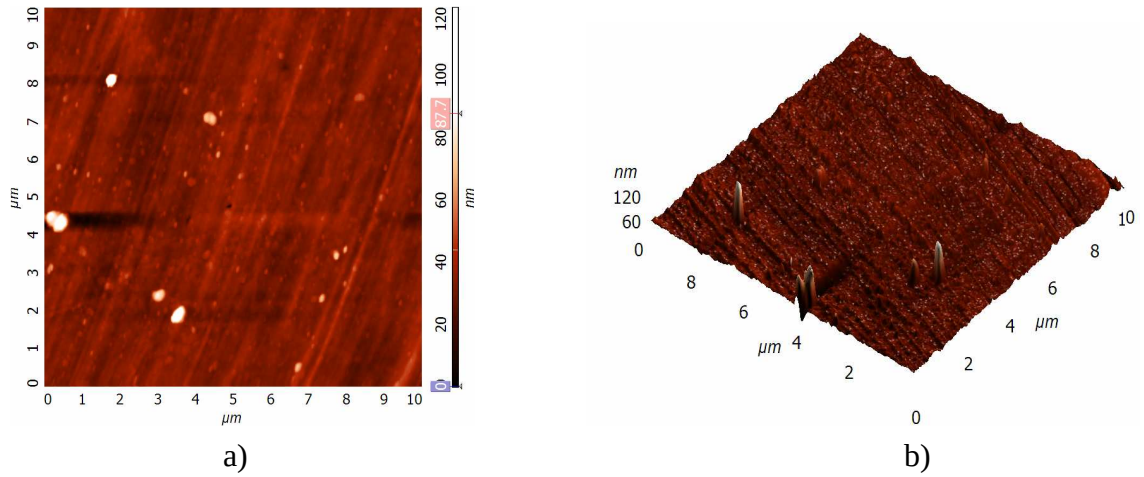
Figure 48: AFM images of untreated PP plate; a) height and b) 3D image.
