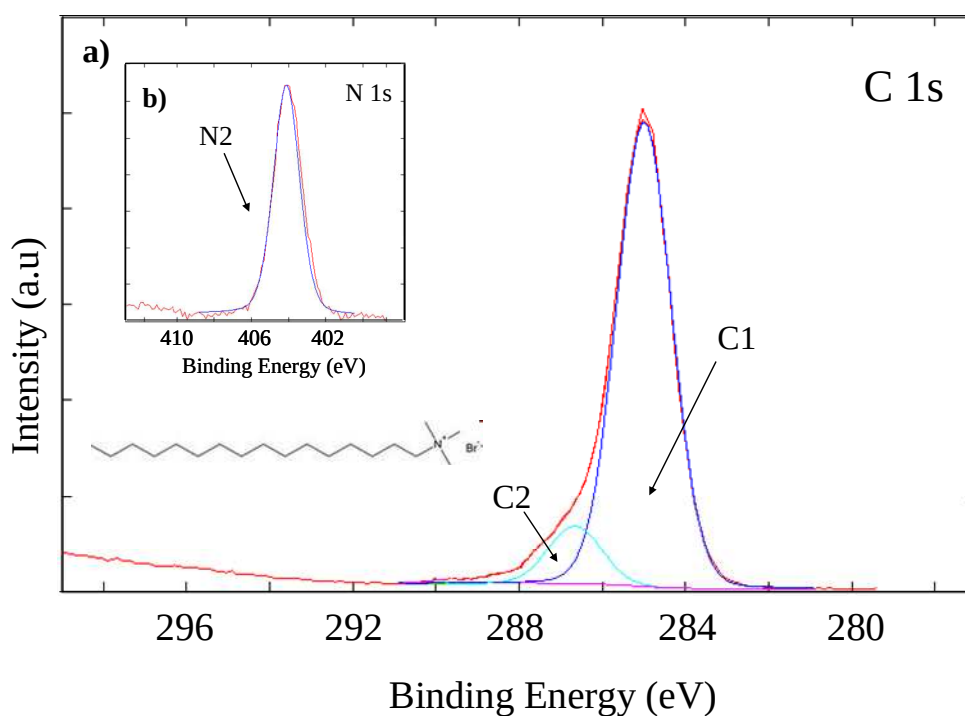
Figure 66: High resolution a) C 1s and b) N 1s spectra of CTAB grafted on helium activated PP plates ( P = 75 W, flow = 30 sccm and t = 3 min; t_{\text{dipping}} = 5 h and C_{\text{CTAB}} = 1 mM).
