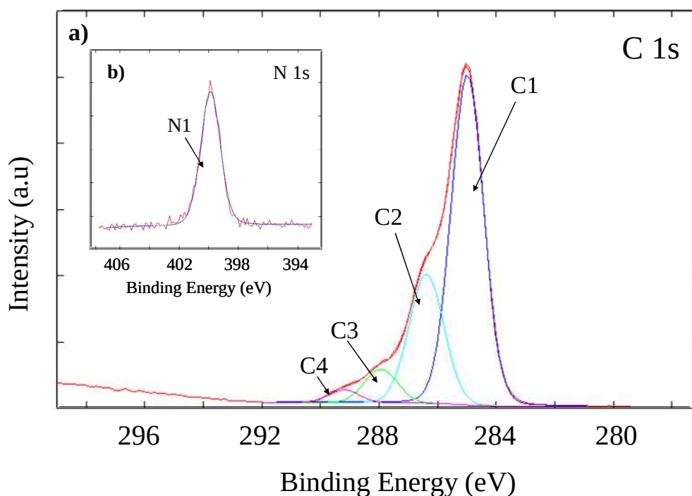
Figure 69: High resolution a) C 1s and b) N 1s spectra of MIX II grafted on helium activated PP plates (P= 75 W, flow= 30 sccm and t= 3 min; t_{\text{dipping}} = 5 h; W_{\text{Tween20}} = 0.05% and C_{\text{PNIPAM}} =0.5g/L).
