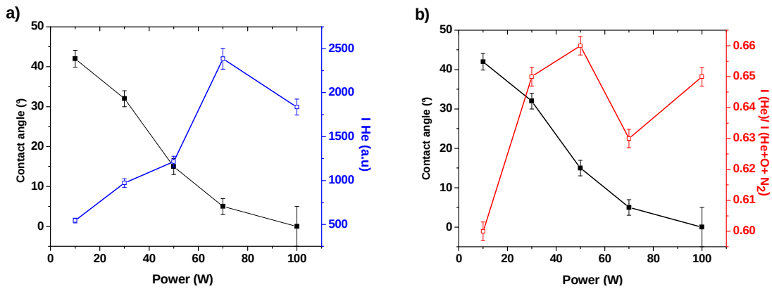
Figure 53: Effect of power on water contact angles of He plasma treated PP plates vs. a) He intensity lines and b) relative intensity of He line toward impurities ( \text{He} / \text{He} + \text{O} + \text{N}_2 ) obtained from optical emission spectroscopy.
