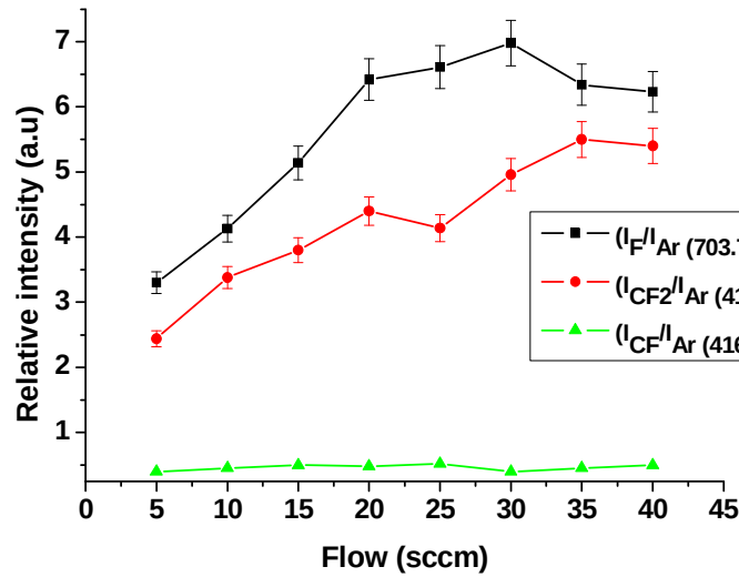
Figure 38: Evolution of relative intensities of F, CF and CF_2 lines as a function of gas flow at P= 50W ; p= 8.2 \times 10^{-3} mbar (5 sccm) to 3.9 \times 10^{-2} mbar (40 sccm).
