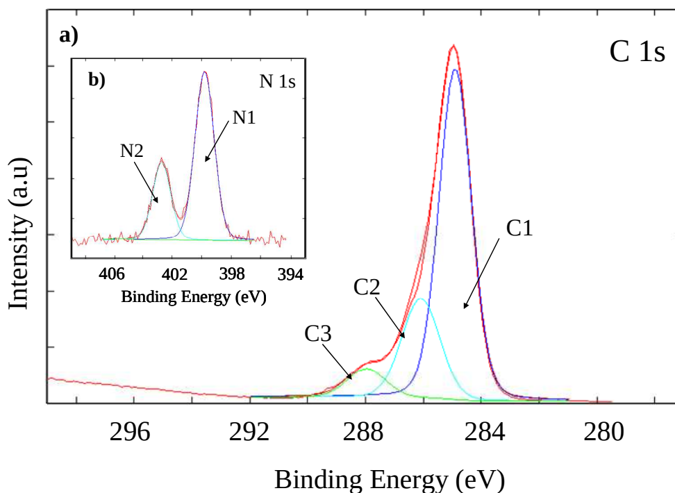
Figure 67: High resolution a) C 1s and b) N 1s spectra of CTAB grafted on helium activated PP plates ( P = 75 W, flow = 30 sccm and t = 3 min; t_{\text{dipping}} = 5 h; C_{\text{CTAB}} = 1 mM and C_{\text{PNIPAM}} = 0.5 g/L).
