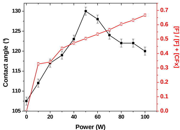
Figure 39: Effect of discharge power on water contact angles of CF 4 treated PP plates (black curve) and on relative concentration of fluorine species in the discharge obtained from actinometry measurements (red curve).
