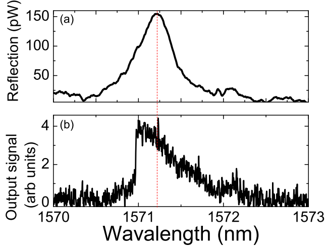
Figure 5.13: Upper trace: Linear resonance obtained using the 30 nm-broadband resonant signal (as in fig.5.11), resolution: 0.05 nm. Lower trace: Resonance obtained by means of a CW modulated signal and a Lock-in detection. Peak power=0.5 mW, integration time: 300 ms, resolution: 5 pm. Note the resonance asymmetry and the abrupt switch at the blue side of the resonance.
