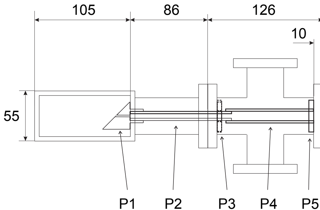
Figure C.11: Schematic of the 2D-MOT vacuum parts showing the glass cell, a standard CF40 cross and homemade stainless steel pieces, including a polished mirror (P1), two differential pumping tubes (P2, P4) and two support rings (P3, P5), which are detailed in the subsequent figures. The inner diameter of the glass-to-metal junction of the glass cell is 32 mm and of the CF40 cross 34.9 mm, the thickness of the walls of the glass cell is 5 mm. The total differential pumping tube has a diameter of 2 mm over 20 mm, 5 mm over 106 mm and 10 mm over 86 mm.
