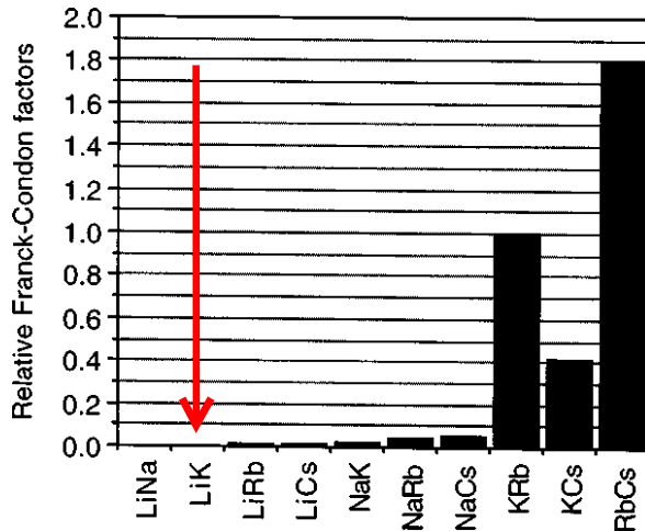
Figure 4.2: Relative values of the Franck-Condon factors for the different heteronuclear alkali dimers for PA at long-range, based on the reflection approximation [197]. The small value for \text{LiK} indicates that the photoassociative creation of \text{LiK}^* molecules is expected to be much more difficult than for the other dimers. Figure taken from Ref. [197].
