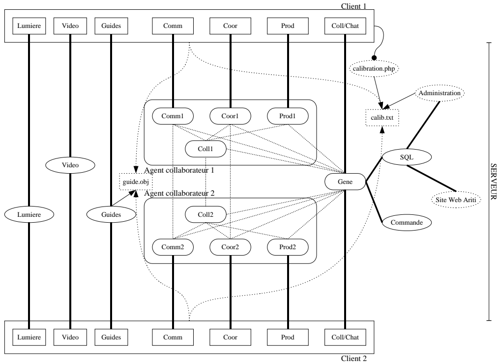
(a) Architecture générale
