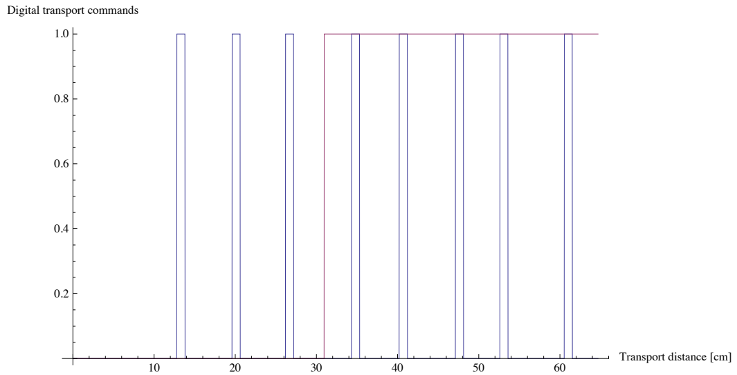
Figure 4.30: Digital clock sequence to drive the transport shift logics (blue), and switch at the elbow (pink).
