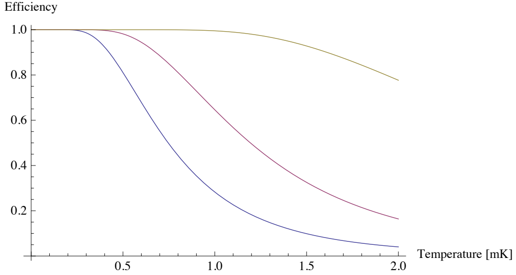
Figure 5.10: Theoretical efficiency of trapping {}^6\text{Li} and {}^{40}\text{K} atoms in a static magnetic trap of gradient 93\text{ G}\cdot\text{cm}^{-1} as a function of temperature, for three different tubes: DN10 (blue), DN16 (pink), and DN38 (yellow). The model used is given in equations 5.2 and 5.4.
