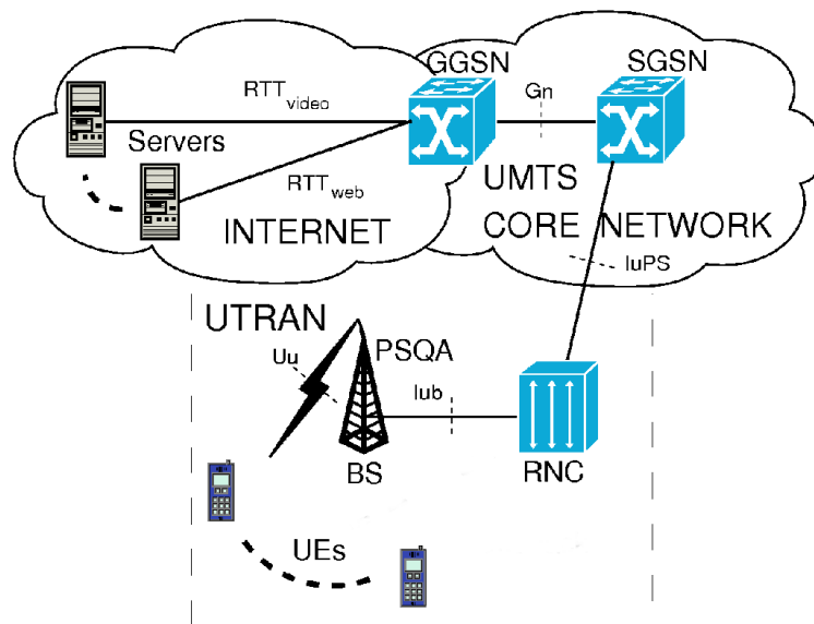
Figure 6.1: Simulation topology.
