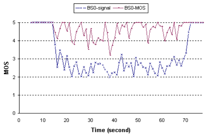
Figure 7.5: Overall User Mean Opinion Score in BS0.
