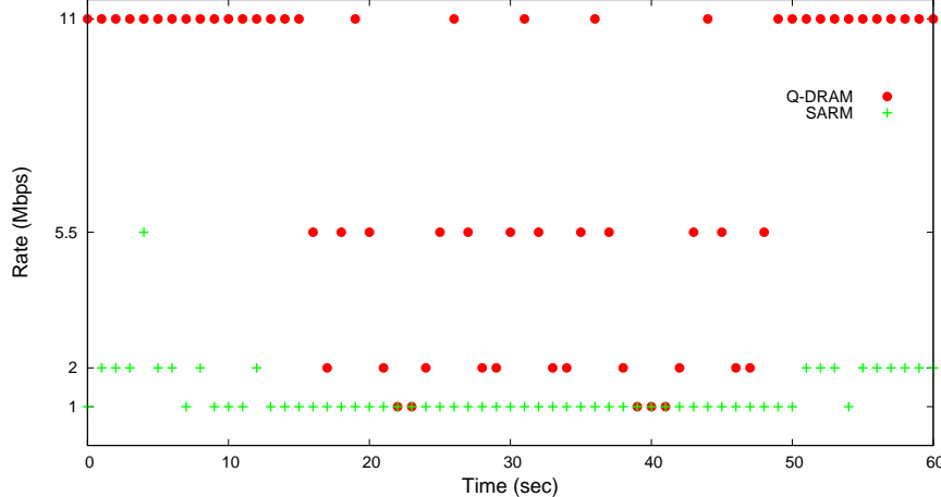
Figure 5.16: Selected rates of Q-DRAM and SARM during the test scenario.
