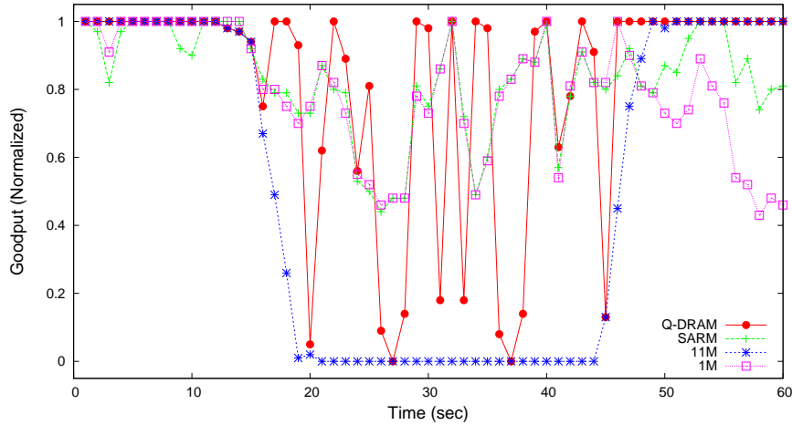
Figure 5.18: Goodput of a moving station (st1).
