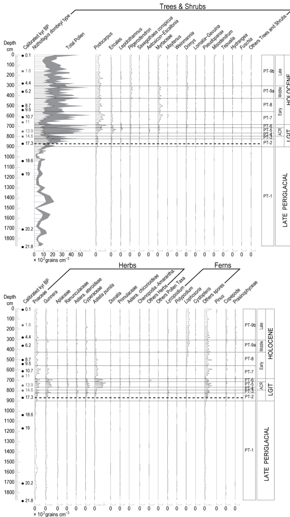
Figure 4.4: Concentration Pollen diagram from core MD07-3088 with the pollen zones and chronostratigraphy indicated on the right and calibrated ages pointed on the left. The dashed line shows the sedimentation rate change from the glacial period to the deglacial and Holocene periods.
