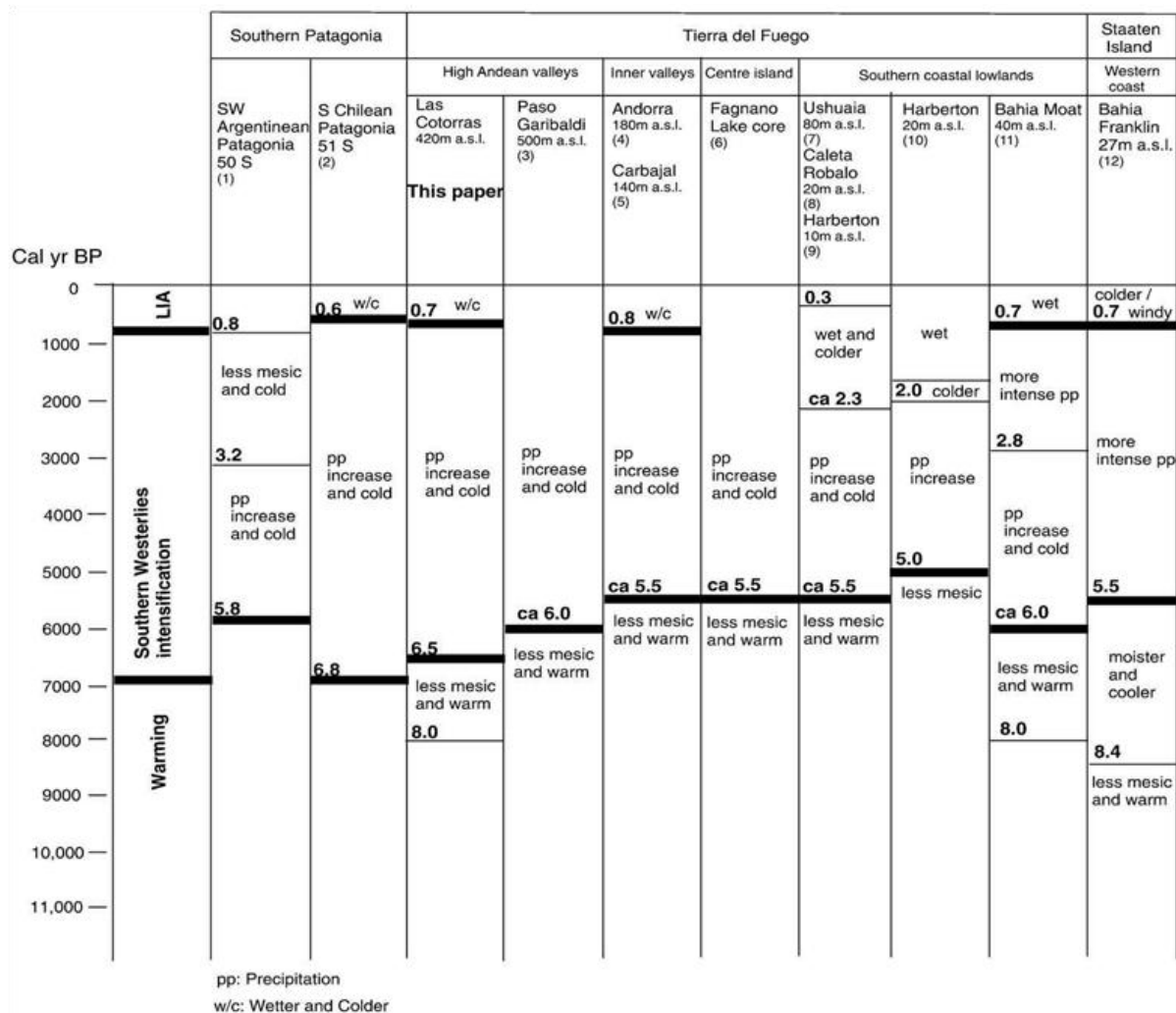
Figure 5.8: Comparative Holocene climate changes from selected peat and lake records from Southern Patagonia and the Fuegian Archipelago after Borromei et al. (2010). Black lines show the onset of Southern Westerlies and the localities where the Little Ice Age event has been reported. References: 1, (Mancini, 2009); 2, (Moreno et al. , 2009a; Villa-Martínez & Moreno, 2007); 3, (Markgraf, 1993); 4, (Borrromei, 1995; Mauquoy et al. , 2004); 5, (Borrromei et al. , 2007); 6, (Waldmann et al. , 2010); 7, 8, 9, (Heusser, 2003); 10, (Pendall et al. , 2001); 11, (Heusser, 1995); 12, (Ponce et al. , 2011).
