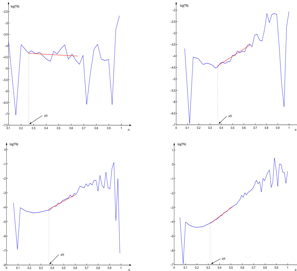
FIGURE 2.1 – Log-log graphs for different samples of X^{(D,D')} with D = 0.5 and D' = 1 when N = 10^3 (up and left, \widehat{\widehat{D}}_N \simeq 1.04 ), N = 10^4 (up and right, \widehat{\widehat{D}}_N \simeq 0.66 ), N = 10^5 (down and left, \widehat{\widehat{D}}_N \simeq 0.62 ) and N = 10^6 (down and right, \widehat{\widehat{D}}_N \simeq 0.54 ).
