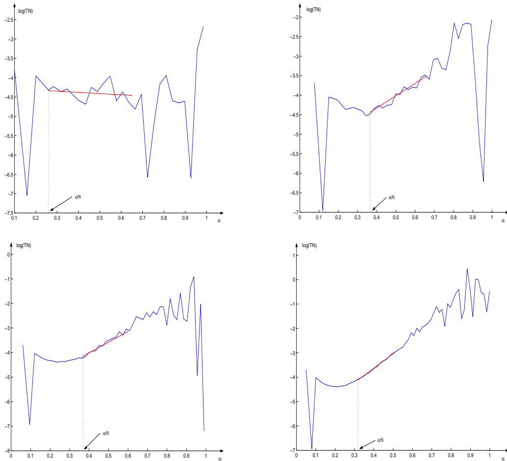
FIGURE 2.1 – Log-log graphs for different samples of X^{(D,D')} with D = 0.5 and D' = 1 when N = 10^3 (up and left, \hat{\tilde{D}}_N \simeq 1.04 ), N = 10^4 (up and right, \hat{\tilde{D}}_N \simeq 0.66 ), N = 10^5 (down and left, \hat{\tilde{D}}_N \simeq 0.62 ) and N = 10^6 (down and right, \hat{\tilde{D}}_N \simeq 0.54 ).
