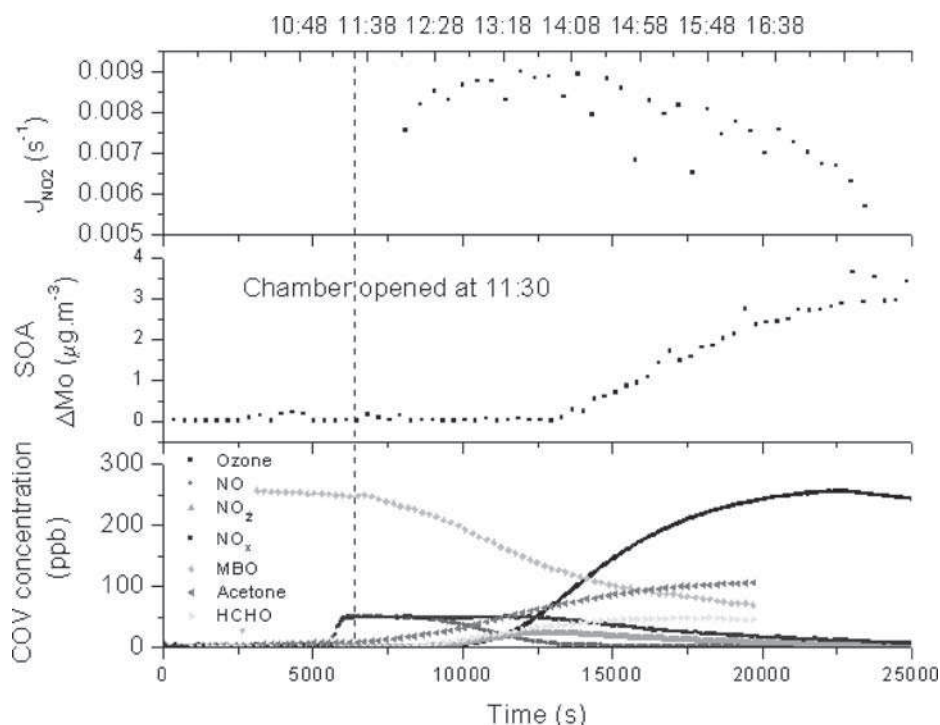
Figure 11 J_{\text{NO}_2} , SOA yield and concentrations of COV, ozone and \text{NO}_x during a photo-oxidation experiment in EUPHORE : [\text{MBO}]_0=250 ppb, [\text{NO}]_0=50 ppb, natural irradiation at 11:30.
