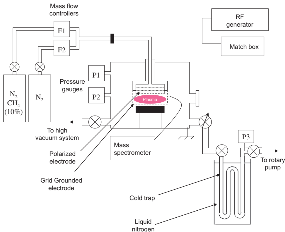
Fig. 1. Schematic of the PAMPRE experimental setup.
