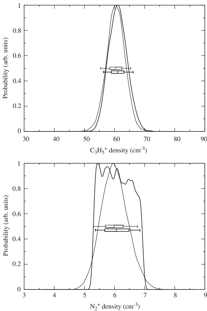
Fig. 5. C_3H_5^+ and N_2^+ density distributions at 1200 km obtained by uncertainty propagation with log-uniform (thick line) and log-normal (dotted line) rate constant uncertainties. Horizontal boxplots depict the 5/25/50/75/95 quantiles.
