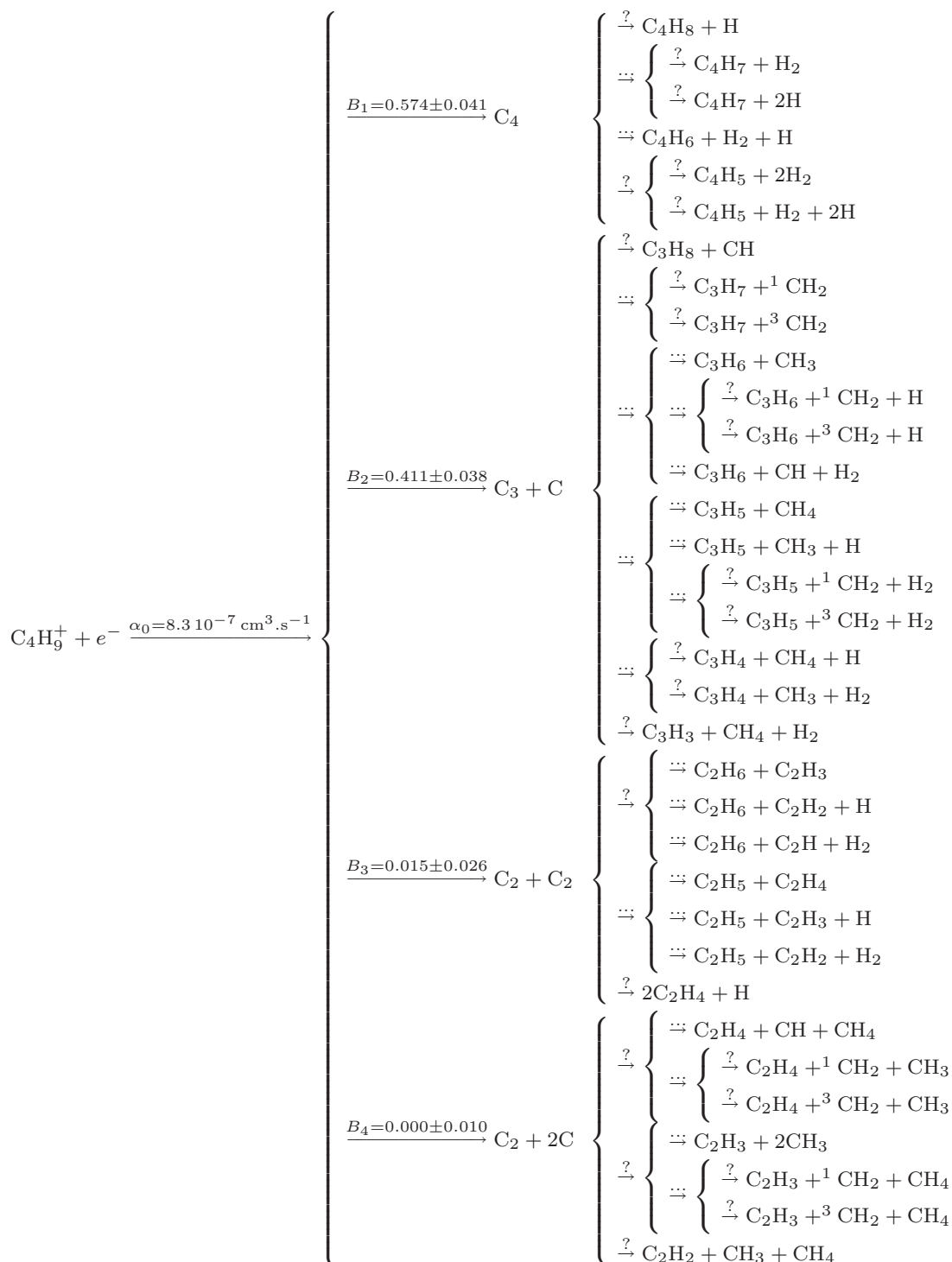
FIG. 1. Tree structure of the putative products for the DR of C_4H_9^+ . The first level implements available experimental data about the carbon fragmentation pattern (Ref. 16); deeper levels are built according to a list of exoergic channels and the list of species involved in the chemical system of interest. The deep tree structure presented here is obtained according to a heuristic explained in the text.
