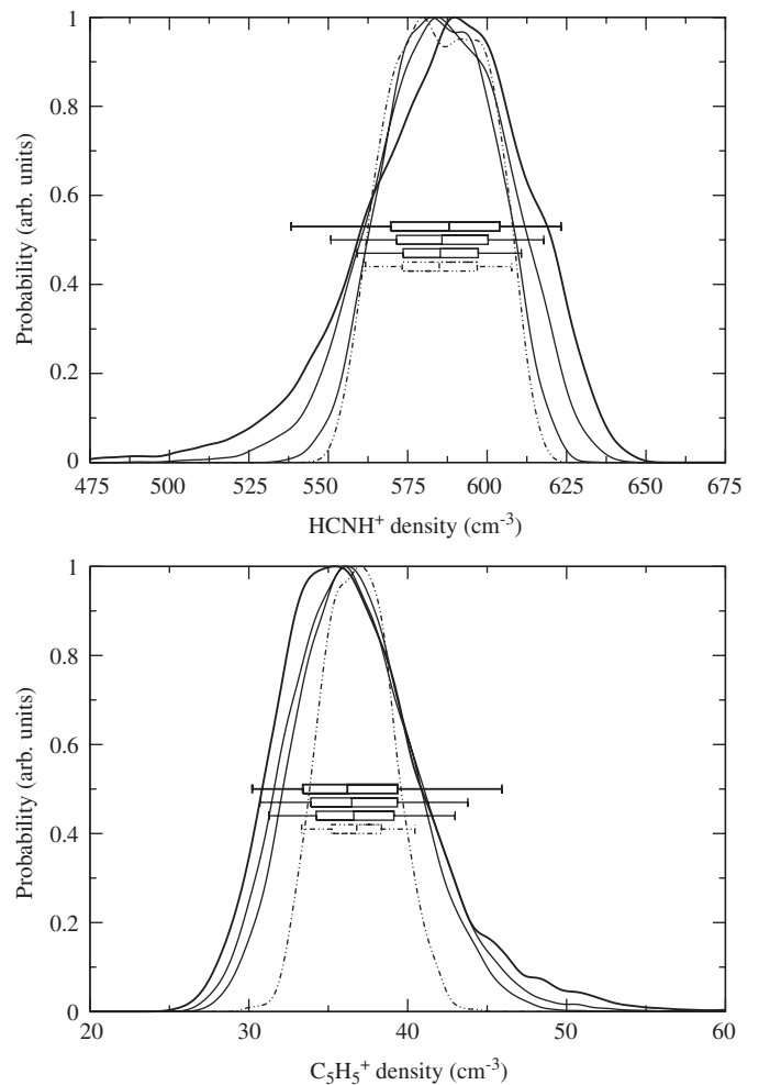
Fig. 6. HCNH^+ and C_5H_5^+ density distributions at 1200 km for night-time chemistry: with no (dashed line)/25% (thin line)/50% (normal line)/75% (thick line) relative uncertainty on the branching ratios. Horizontal boxplots depict the 5/25/50/75/95 quantiles.
