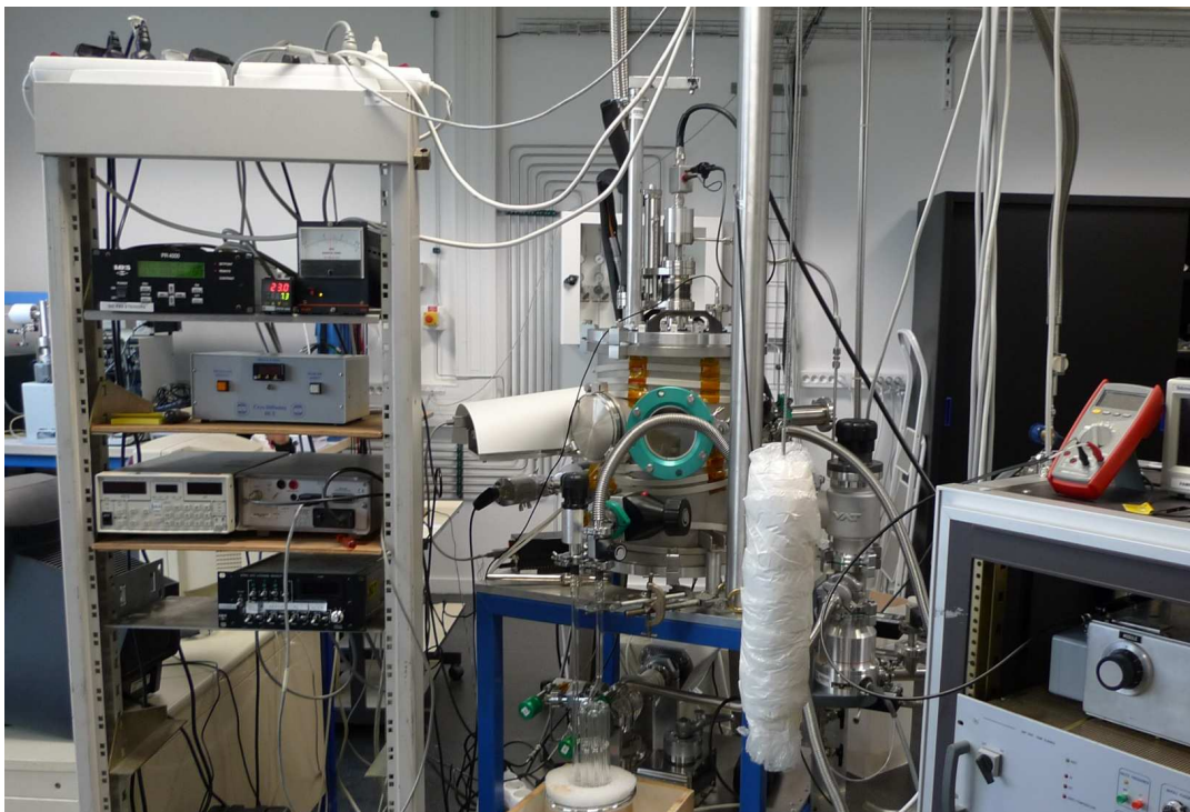
Figure 10: Installation PAMPRE au LATMOS.
