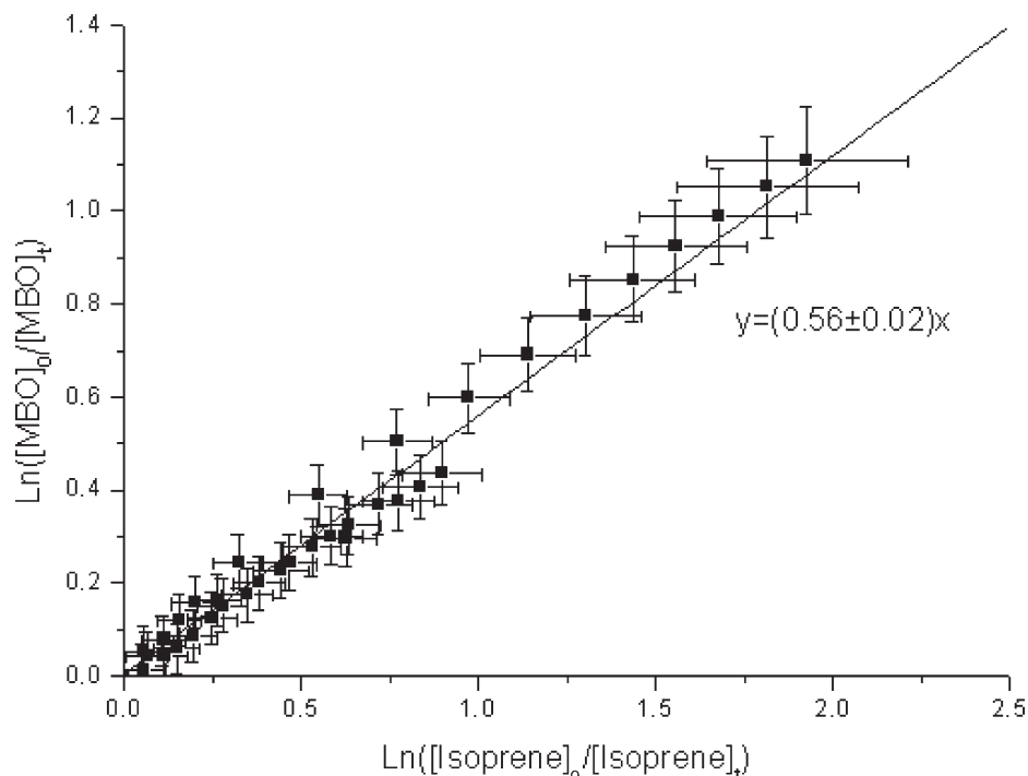
Figure 1 Relative decay of MBO versus Isoprene when exposed to OH radicals.
