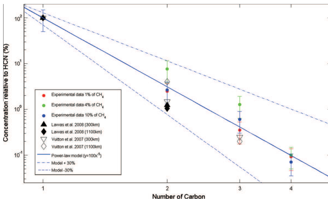
Fig. 5. Relative concentration of the nitriles as a function of the number of carbon in the molecules. The red, green and blue dots represent the experimental data from this work, for experiments with 1%, 4% and 10% of methane in the reactor, respectively. The blue line is the empirical power law model ( y = ax^b ) associated to these experimental data. The dot-dashed line represents the model value plus 30% ( a' = a + 30\% ; b' = b - 30\% ) while the dashed line is the model value minus 30% ( a'' = a - 30\% ; b'' = b + 30\% ). The empty black diamonds and triangles are observational data (Vuitton et al., 2007, and reference herein), at 1100 and 300 km from Titan's ground, respectively. The full diamonds and triangles are data from computer modeling (Lavvas et al., 2008) at 1100 and 300 km from Titan's ground, respectively. (For interpretation of the references to color in this figure legend, the reader is referred to the web version of this article.)
