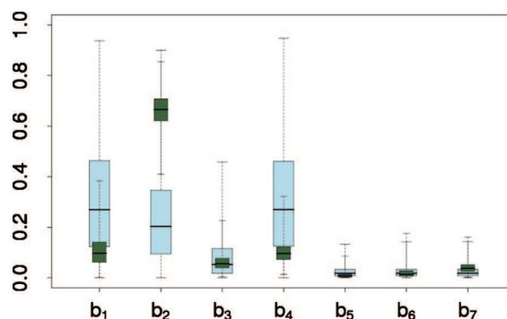
FIG. 9. Comparison of branching ratios \{b_1, \dots, b_7\} for the DR of \text{C}_2\text{H}_4^+ , as measured (dark green boxplots) and recovered from an aggregated version of these data (light blue boxplots).
