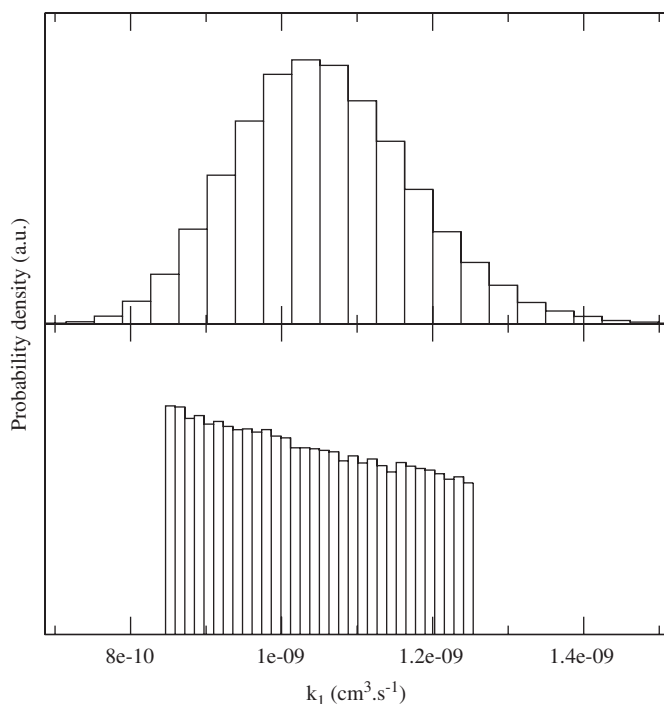
Fig. 1. Elicitation of the probability density function for the rate constant of the reaction \text{N}_2^+ + \text{CH}_4 \rightarrow \text{CH}_2^+ + \text{NH}_2 ( b_1 = 0.7 ), with preferred value for the global rate k^0 = 1.5 \times 10^{-9} and relative uncertainty x = 0.2 . Comparison of probability densities for: (upper panel) a log-normal distribution ( k^0 b_1 = 1.05 \times 10^{-9} , F = 1.25 ); (lower panel) a log-uniform distribution ( k_{\min} b_1 = 0.84 \times 10^{-9} , k_{\max} b_1 = 1.26 \times 10^{-9} ).
