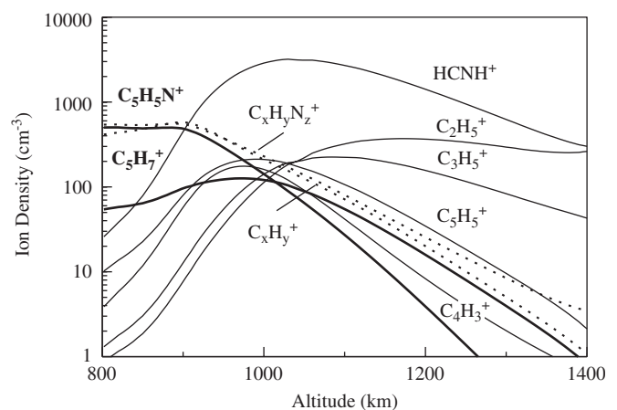
Fig. 3. Ion density profiles with and without specification of pseudo-ions in the model: (thin solid lines) common major ions; (thick solid lines) major former pseudo-ions; (dashed lines) C_xH_yN_z^+ and C_xH_y^+ pseudo-ions in the original model.
