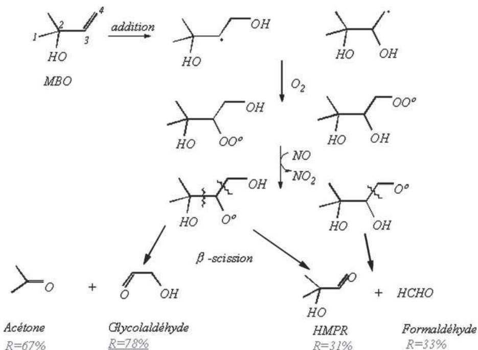
Figure 4 Oxidation scheme of MBO with OH radicals in the presence of \text{NO}_x .
