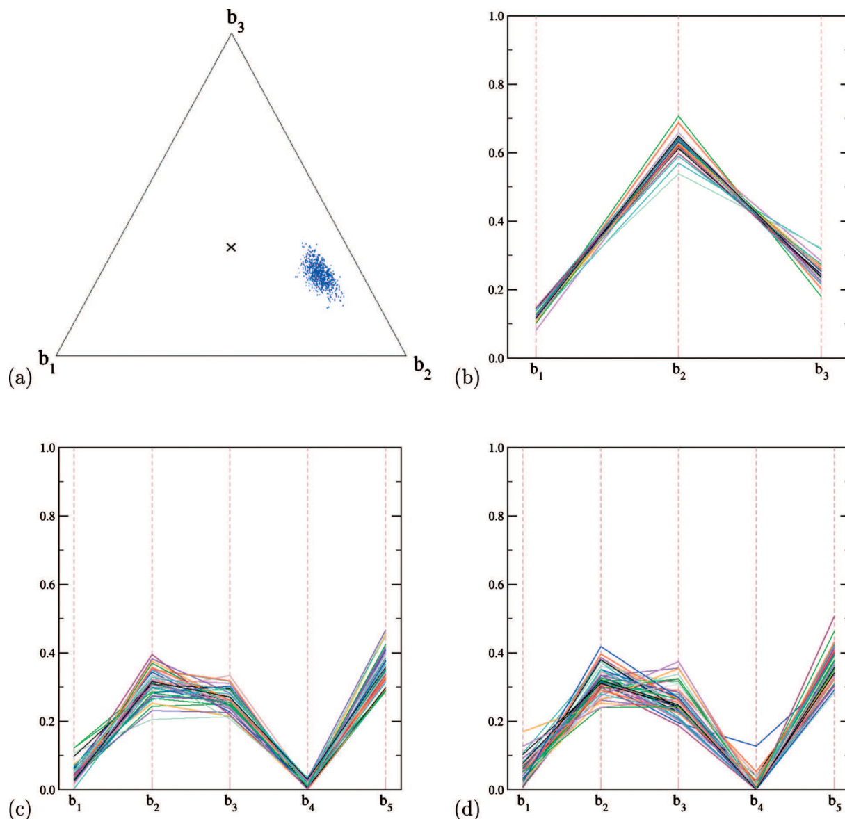
FIG. 7. Samples of uncertain branching ratios for some species of interest: [(a) and (b)] \text{CH}_2^+ with nested Dirg and [(c) and (d)] \text{NH}_2^+ with nested (c) Dirg and (d) one-level Dirg.
