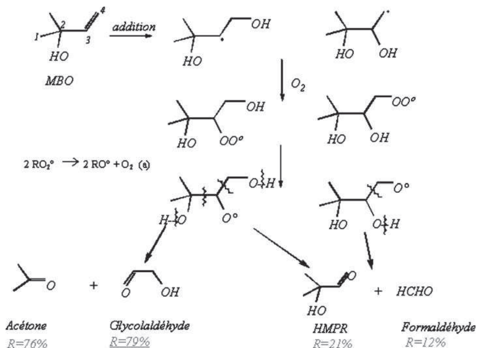
Figure 5 Oxidation scheme of MBO with OH radicals in the absence of NO_x . (a) Horie et al., (1990); Niki et al., (1982); Lightfoot et al., (1991); Wallington et al., (1989).
