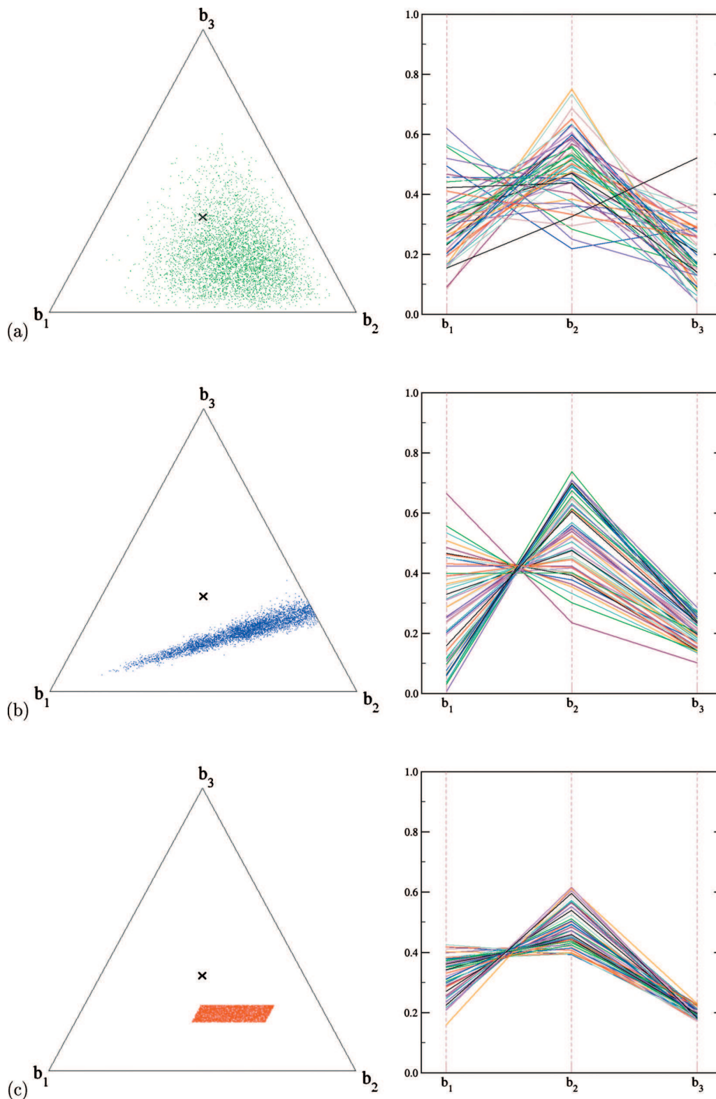
FIG. 4. Ternary (left) and parallel (right) graphs of samples of Dirichlet-type distributions for a set of three branching ratios \{b_1, b_2, b_3\} to represent the following information b_1=0.30 \pm 0.30 , b_2=0.50 \pm 0.04 , and b_3=0.20 \pm 0.01 : (a) \text{Diri}(0.3,0.5,0.2;13.7) , (b) \text{Dirg}(0.3,0.5,0.2;0.3,0.04,0.01) , and (c) \text{Diut}([0.00,1.00],[0.38,0.62],[0.17,0.23]) .
