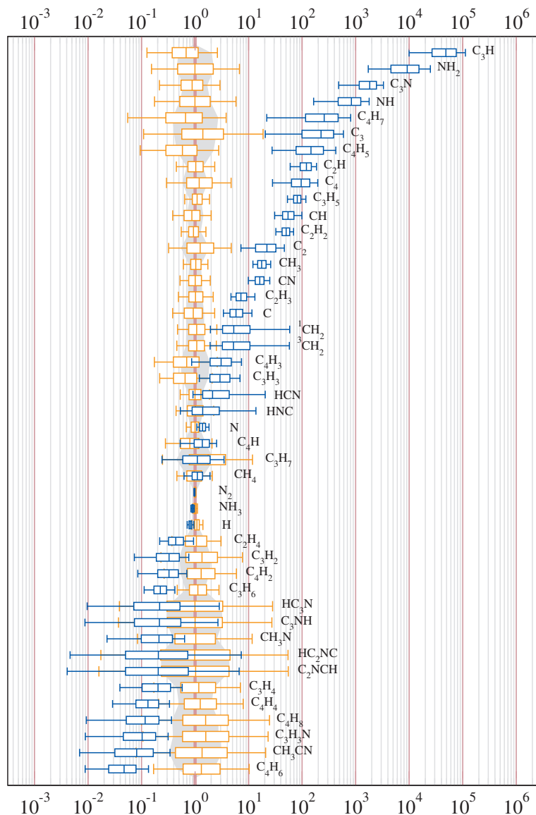
FIG. 10. Comparison of the production rates of neutral species between different DR model implementations: (brown) ratio v_M^{\text{full}}/v_M^{\text{flat}} between the nested and flat versions of the “full” model (see text); (blue) ratio v_M^{\text{full}}/v_M^{\text{H-loss}} between the full and “H-loss” models. The gray zone depicts the intrinsic dispersion due to the Monte Carlo estimation of production rates ratios: symmetric 50% probability interval for the ratio v_M^{\text{full}}/v_M^{\text{full}} estimated from two independent samples.
