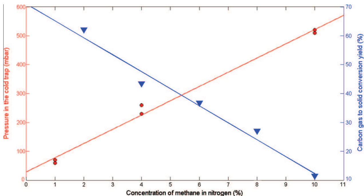
Fig. 2. Evolution of the gas pressure measured in the cold trap after warming up to room temperature (red dots) and of the carbon gas to solid conversion yield (blue triangles, from Sciamma-O'Brien et al. (2010) as a function of \text{CH}_4 concentration). (For interpretation of the references to color in this figure legend, the reader is referred to the web version of this article.)
