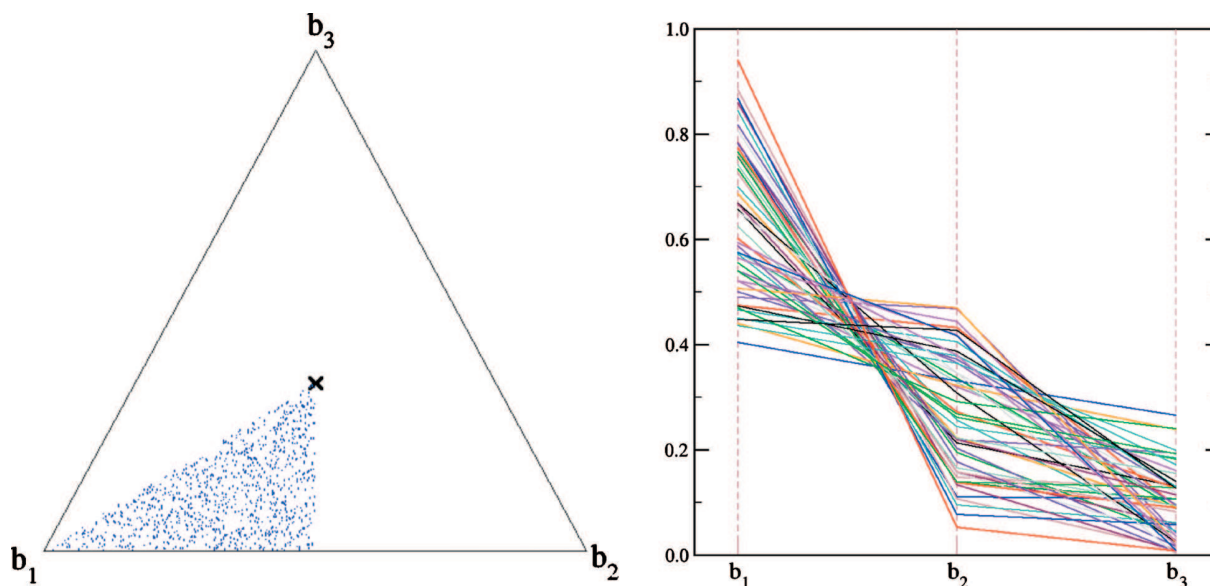
FIG. 5. Dirichlet distributions for a set of three branching ratios \{b_1, b_2, b_3\} when only ordering information ( b_1 \geq b_2 \geq b_3 ) is available: Dior(3).
