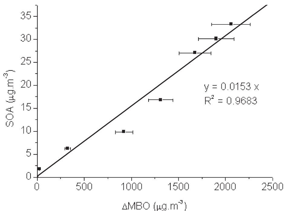
Figure 10 SOA production yield plot during a typical MBO ozonolysis experiment. [\text{MBO}]_0=1.5 ppm v , [\text{O}_3]=3.0 ppm v .
