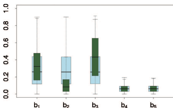
FIG. 8. Influence of the nesting pattern on the distribution of branching ratios \{b_1, \dots, b_5\} for the DR of \text{C}_3\text{H}_2^+ ; (blue/light) flat representation of the subchannels; (green/dark) nesting of auxiliary information.
