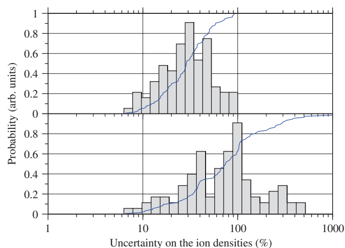
Fig. 7. Distribution of the uncertainties for all ions densities. The full line represents the sample cumulative density function. The simulations were performed by night-time chemistry at 1000 km of altitude for two cases of uncertainty on the branching ratios: (above) no uncertainty; (below) 50% relative uncertainty.
