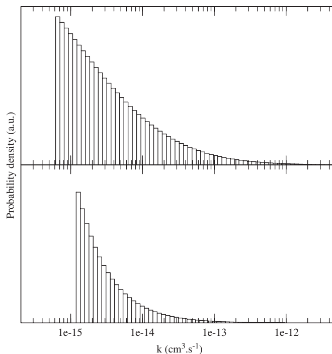
Fig. 2. Elicitation of probability density function for the rate constant of the reaction \text{H}^+ + \text{H}_2 \rightarrow \text{H}_2^+ + \text{H} . Comparison of probability densities for: (upper panel) a log-normal distribution ( k^0 = 5 \times 10^{-13} , F = 435 ); (lower panel) a log-uniform distribution ( k_{\min} = 1.2 \times 10^{-15} , k_{\max} = 1.0 \times 10^{-12} ).
