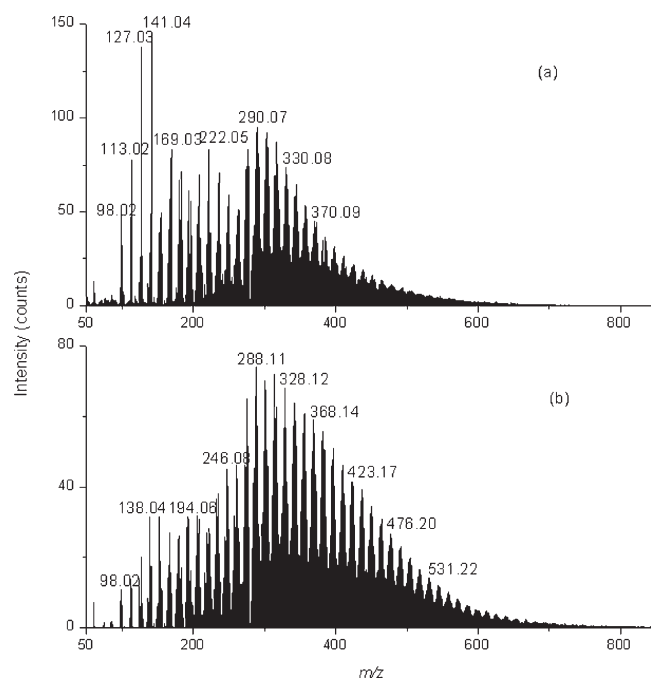
Figure 5. APPI mass spectra of tholins soluble fraction in methanol in positive ion mode: (a) SA98; (b) SA90. \text{CH}_4 inlet percentage effect on tholins composition.
