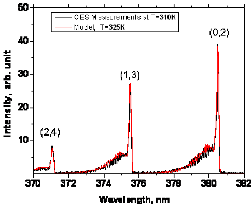
Figure 18 : Spectre UV d'un plasma N 2 (98%)-CH 4 (2%)
