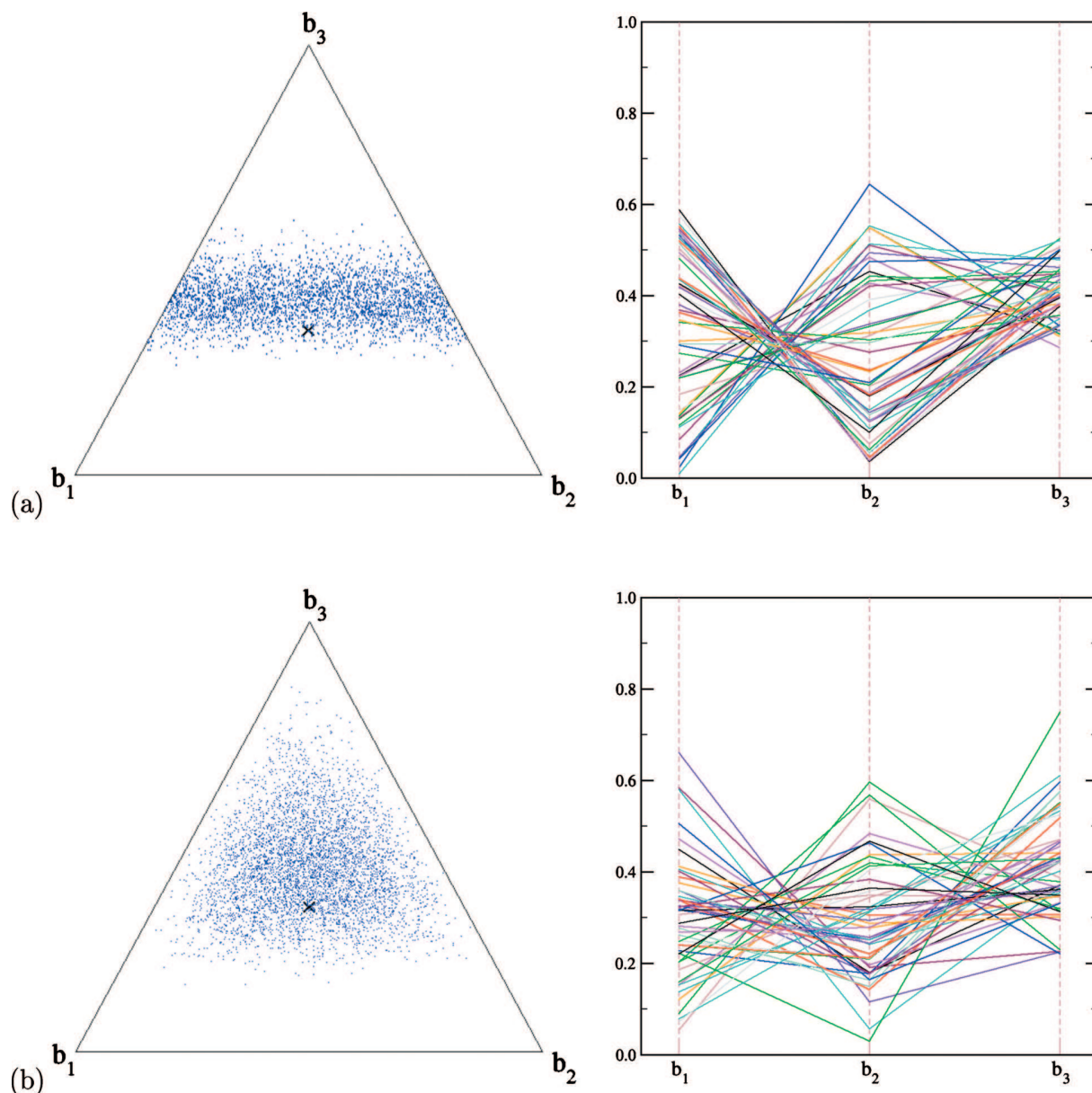
FIG. 6. Comparison of two representations for the consolidation of complementary branching ratios information (see text for details): (a) \{b_1, b_2, b_3\} \sim \text{Dirg}(0.6 \otimes \text{Diun}(2), 0.4; 0.1, 0.05) and (b) \{b_1, b_2, b_3\} \sim \text{Dirg}(0.30, 0.30, 0.40; 0.18, 0.18, 0.05) .
