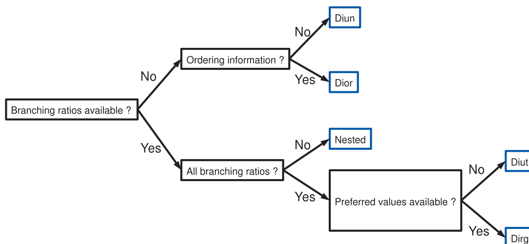
FIG. 3. Decision tree for the choice of a Dirichlet-type distribution.
