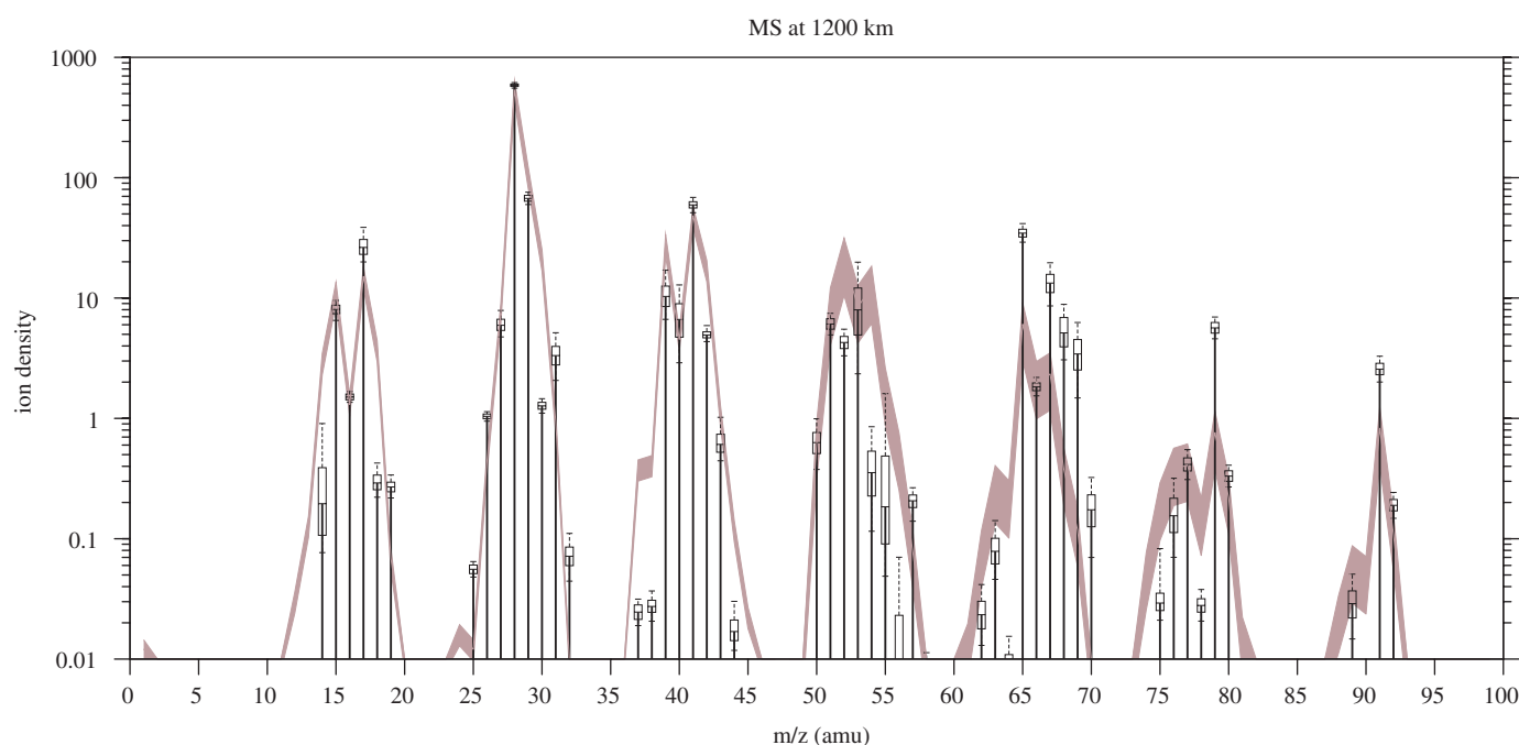
Fig. 9. Simulated (drop lines) and measured (envelope) mass spectra of Titan ionosphere at 1200 km of altitude by night time. Box-plots and error bars correspond to confidence intervals of 50% and 90% for the calculated mass spectrum. Vertical boxplots depict the 5/25/50/75/95 quantiles.
