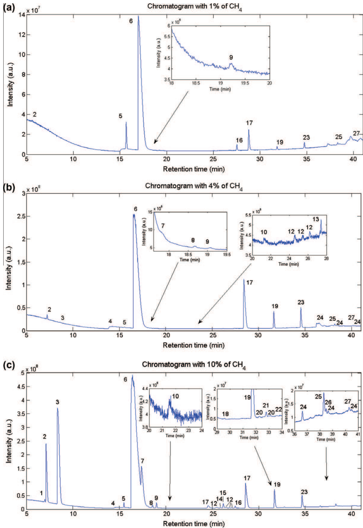
Fig. 3. (a–c) Chromatograms of gas samples trapped during experiments with, respectively, 1% (a), 4% (b) and 10% \text{CH}_4 (c) from GC–MS analysis. Peaks are numbered in agreement with Table 1. Minor peaks are shown in the insets.
