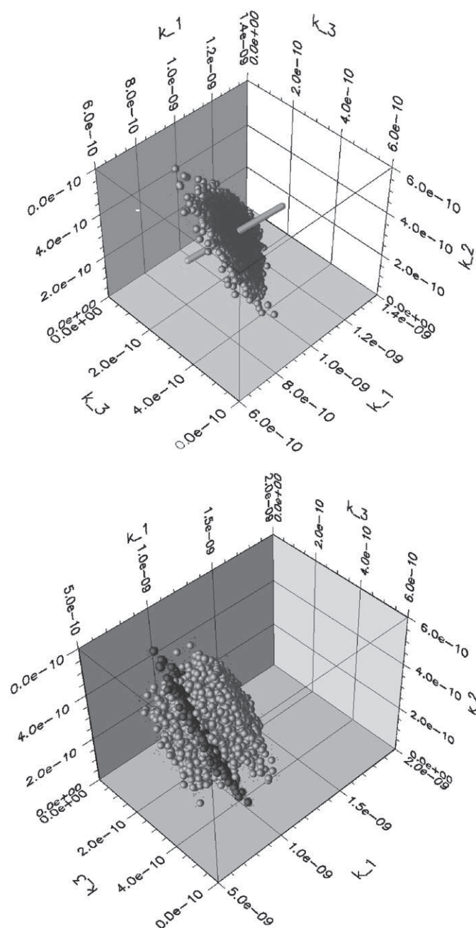
Fig. 4. Partial rates of reaction (7). The samples have been generated according the following scheme: (top panel, clear dots) fixed branching ratios and log-uniform distribution for k^0 ; (both panel, dark dots) fixed k^0 and Dirichlet distribution for the branching ratios; and (bottom panel, clear dots) log-uniform distribution for k^0 and Dirichlet distribution for the branching ratios.
