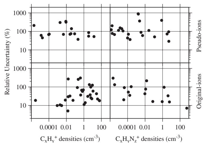
Fig. 8. Relative uncertainties versus ion densities at 1200 km of altitude by night-time chemistry.
