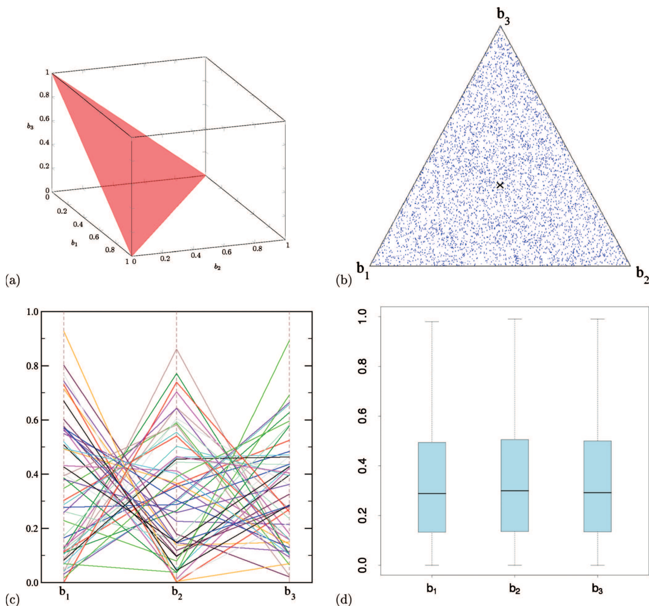
FIG. 2. (a) Visualization of the simplex in a three-dimensional space ( b_1, b_2, b_3 ) and alternative representations of a sample of the uniform distribution within this simplex: (b) ternary graph, (c) parallel graph, and (d) boxplots for the one-dimensional marginal densities p(b_i) , i=1,3 .
