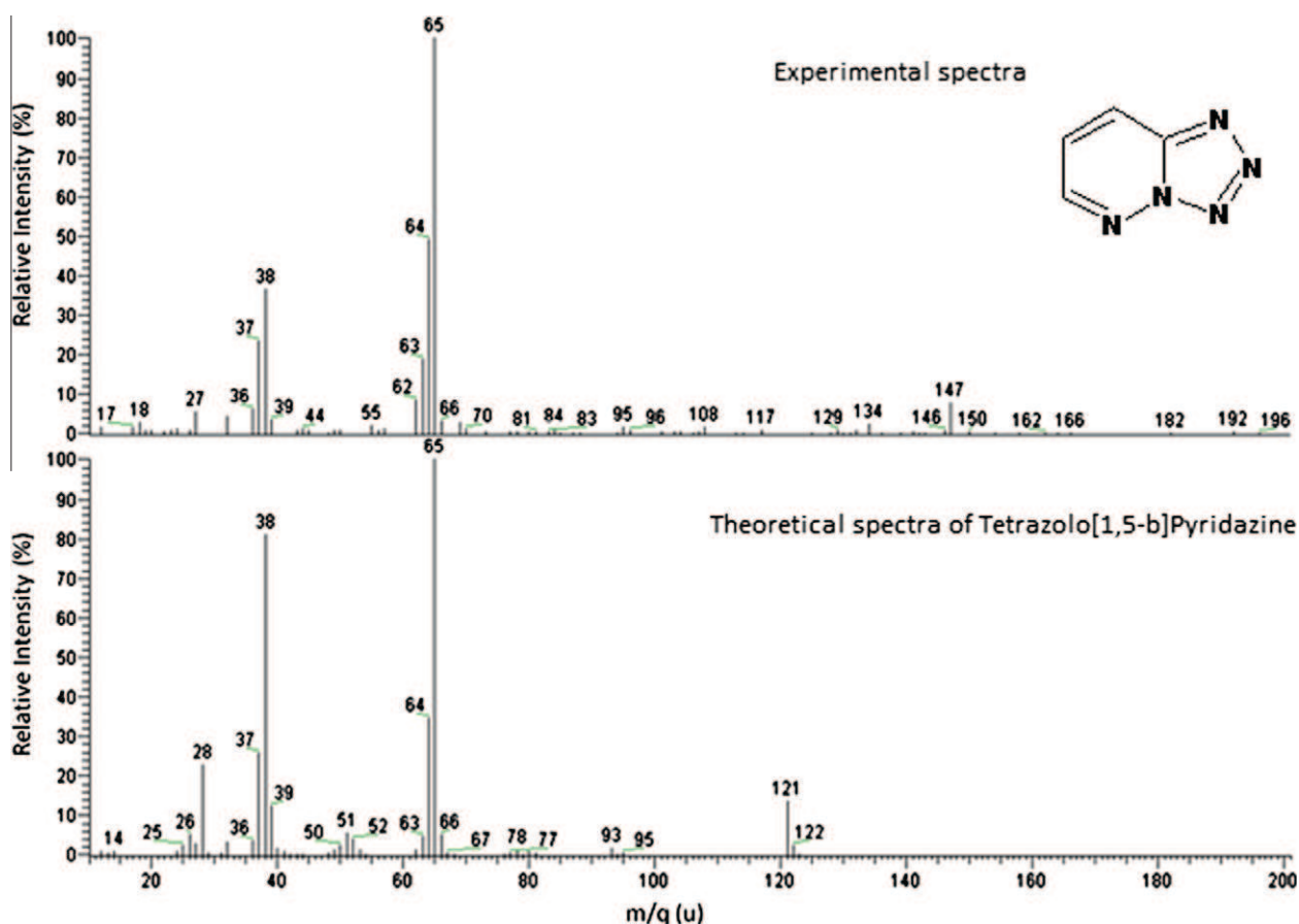
Fig. 4. Experimental (up) and theoretical (down) spectra of tetrazolo[1,5-b]pyridazine. The topological scheme of tetrazolo[1,5-b]pyridazine is given in the up spectra.
