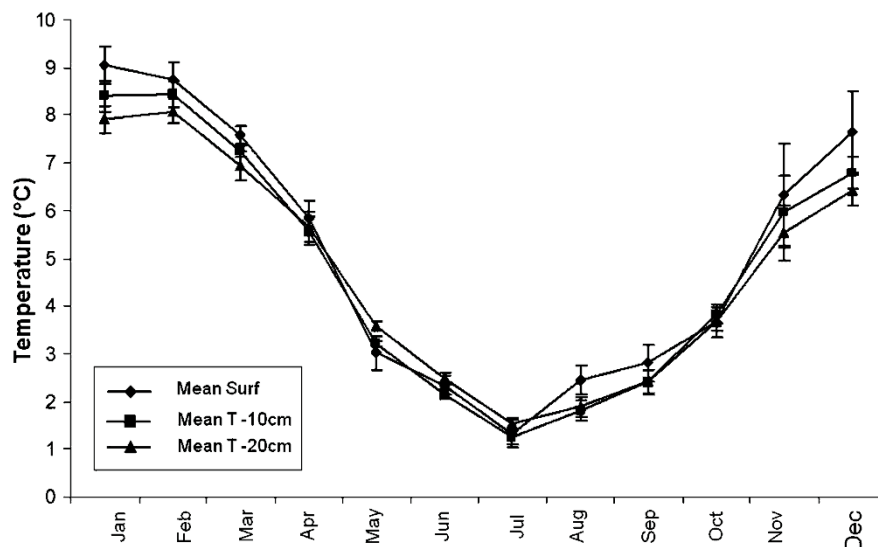
Fig. 2 Time series of mean monthly temperatures ( \pm SEM) at the Kerguelen Islands (Port aux Français) from 2000 to 2005. Temperatures ( ^{\circ} C) were recorded at the ground level, 10 and 20 cm below the ground level with a Delta T data logger (Delta T devices, Cambridge, UK)
