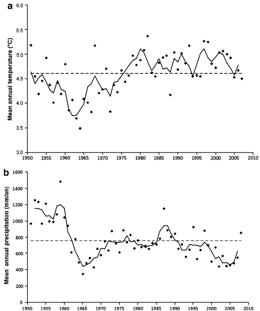
Fig. 1 Annual mean air temperature ( ^{\circ}\text{C} , a ) and annual precipitation ( \text{mm y}^{-1} , b ) at the Kerguelen Islands (Port aux Français) over the period 1951–2008. The broken lines indicate the average annual temperature ( a ) and precipitations ( b ) for the period 1951–2008; the solid lines represent the 3-year running mean. Source: Météo France data
