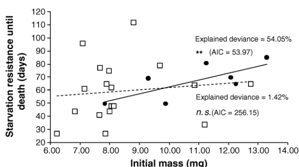
Fig. 2. Generalized Linear Models depicting the relationship between initial mass and starvation resistance in males and females starved until death (see Fig. 1). Open squares and dashed line: males; solid circles and solid line: females. Significance codes: <0.01 “**”; not significant “n. s.”.
