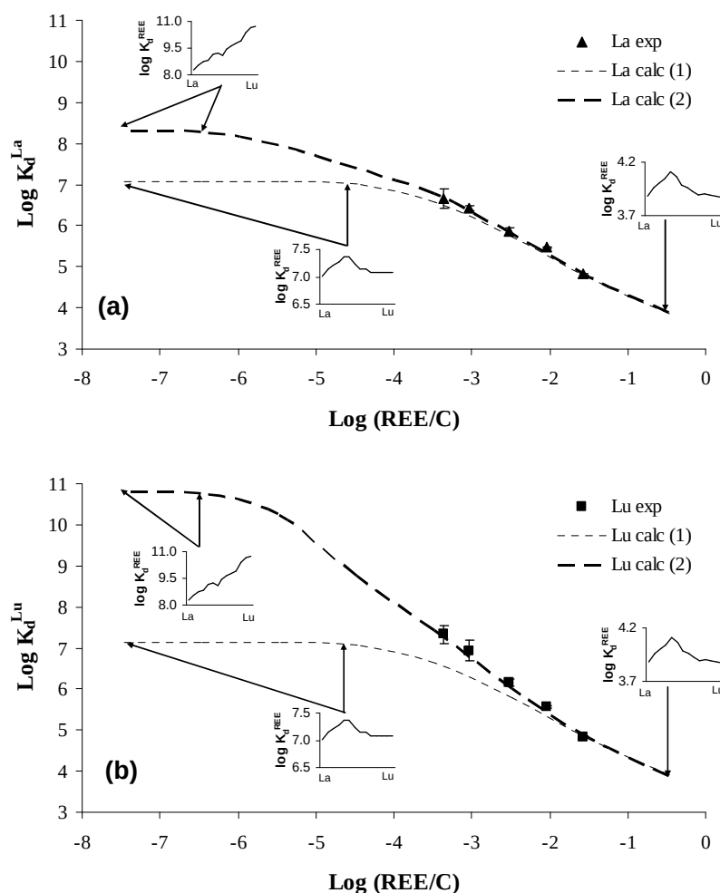
Figure II.6. Variation of (a) \log K_d^{\text{La}} and (b) \log K_d^{\text{Lu}} relative to the \log (\text{REE}/\text{C}) , on a large range of metal loading. Comparison of Model VI prediction with (1) \Delta LK_2 = 0.29 (dashed line) and (2) with the optimized \Delta LK_2 (bold dashed line). Symbols represent experimental data. Error bars correspond to standard deviation of triplicates.
