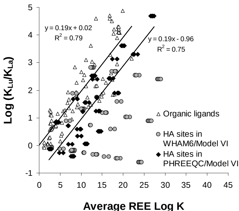
Figure III.3. \log (K_{Lu}/K_{La}) versus the average REE \log K_{REE} values obtained for 101 organic ligands (Byrne and Li, 1995) and for the 80 ligands defined in WHAM 6/Model VI and PHREEQC/Model VI. \log (K_{Lu}/K_{La}) is used as an indicator of the REE-ligand pattern. The linear regression for the 101 organic ligands (Byrne and Li, 1995) and for the 80 HA sites obtained here with PHREEQC/Model VI are also presented.
