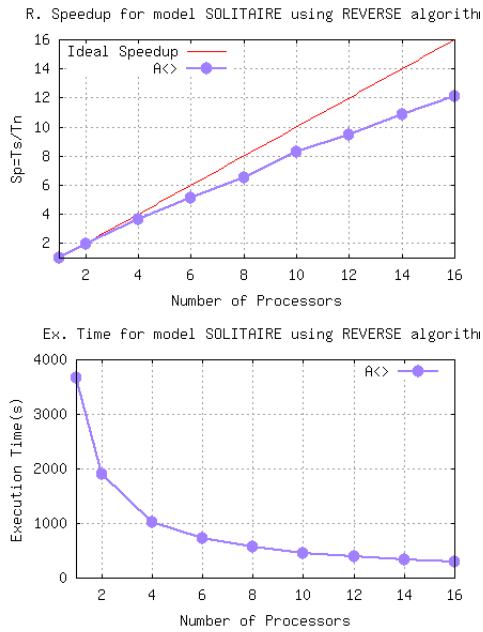
Figure 4.12: Peg with Reverse alg.
