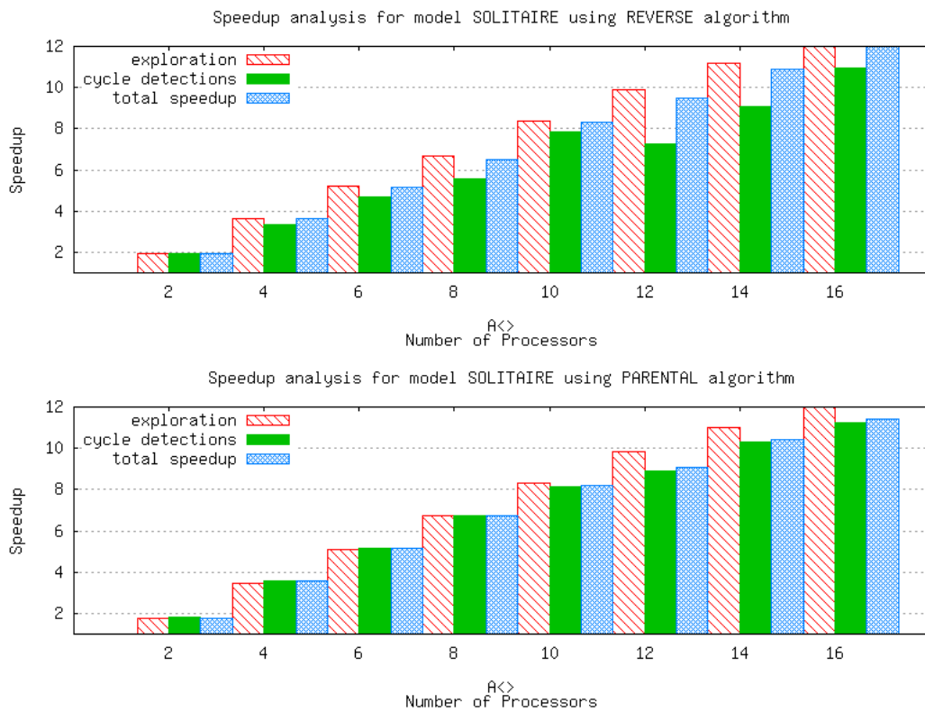
Figure 4.14: Exploration and cycle detection speedup analysis for Peg model.
