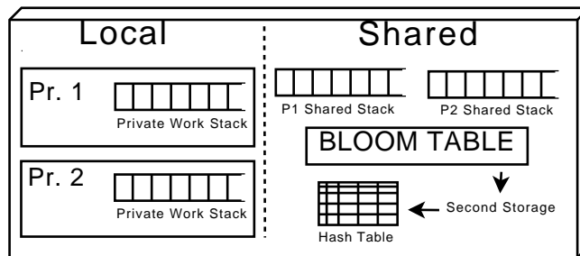
Figure 5.9: Parallel probabilistic verification algorithm overview.
