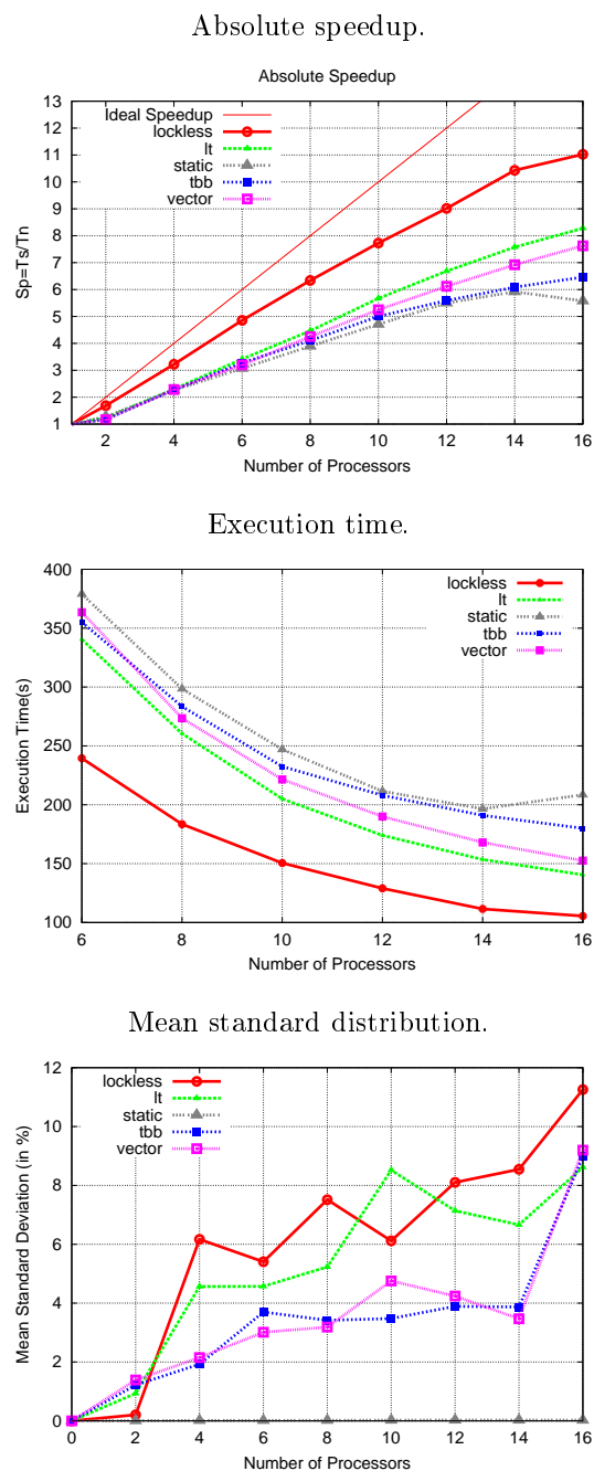
Figure A.2: Parallel State Space Construction for the Sokoban and Peg-Solitaire models.
