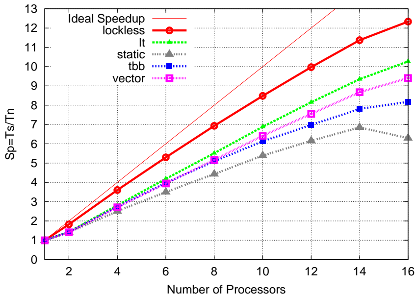
Figure 3.18: Average Speedup.
