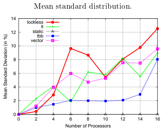
Figure A.5: Parallel State Space Construction for the Kanban and PH models.
