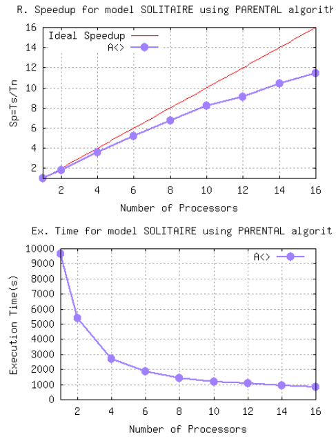
Figure 4.13: Peg with Parental alg.
