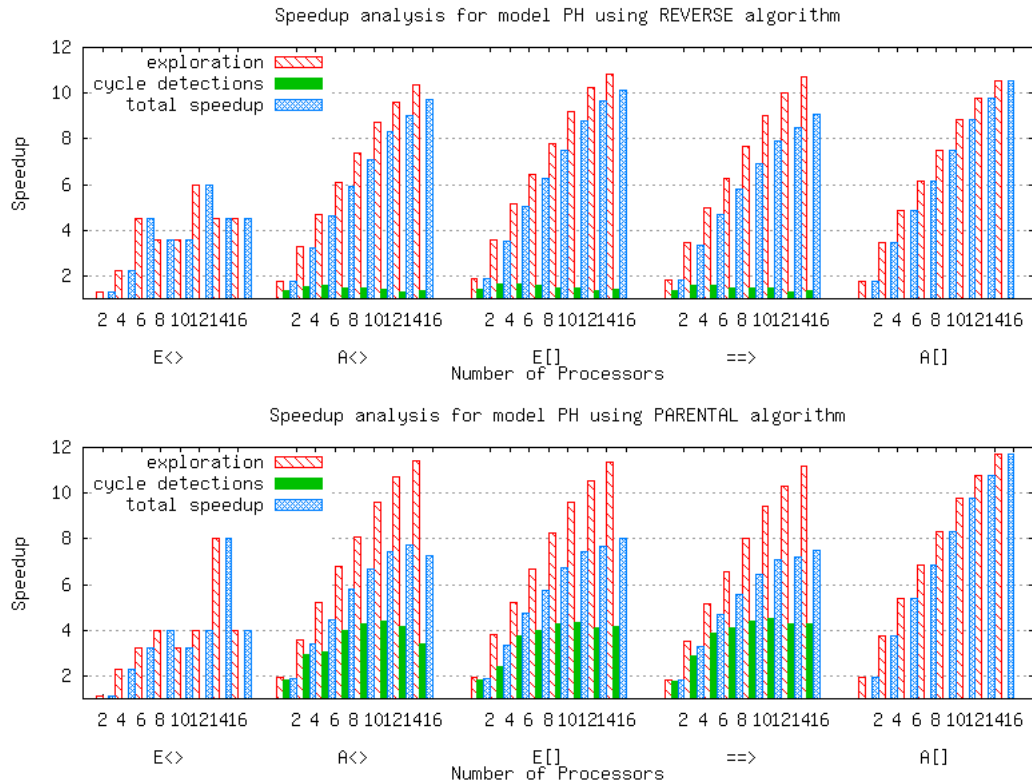
Figure 4.11: Exploration and cycle detection speedup analysis for PH model.
