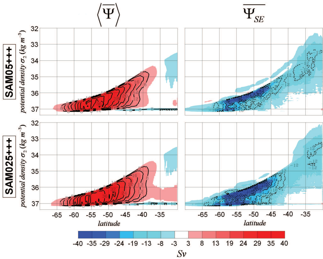
FIG. 5.7 – MOC (in \text{Sv} ) in \sigma_2 potential density coordinates : (left) the Eulerian mean circulation zonally averaged \langle \bar{\Psi} \rangle , (right) the standing eddy-driven circulation \overline{\Psi}_{SE} for (from top to bottom) SAM05+++ and SAM025+++ experiments. Red cells correspond to clock-wise flows and blue cells to counter-clockwise flows.
