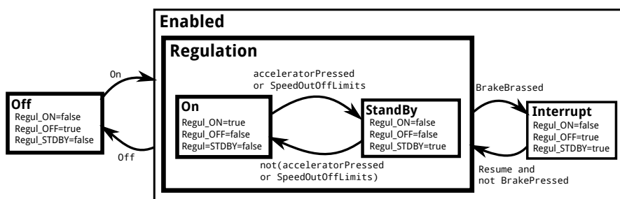
FIGURE 5.4: Automate CruiseControl .
