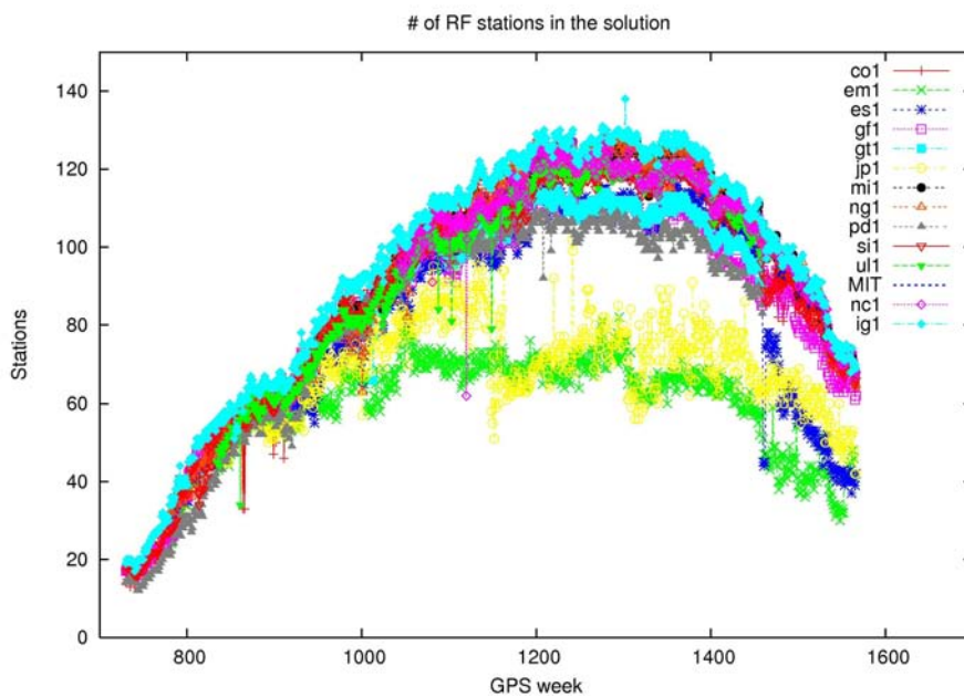
Figure 7.1. Number of IGS reference frame stations (IGS05) analyzed by solution contributing to the IGSr 3 .
