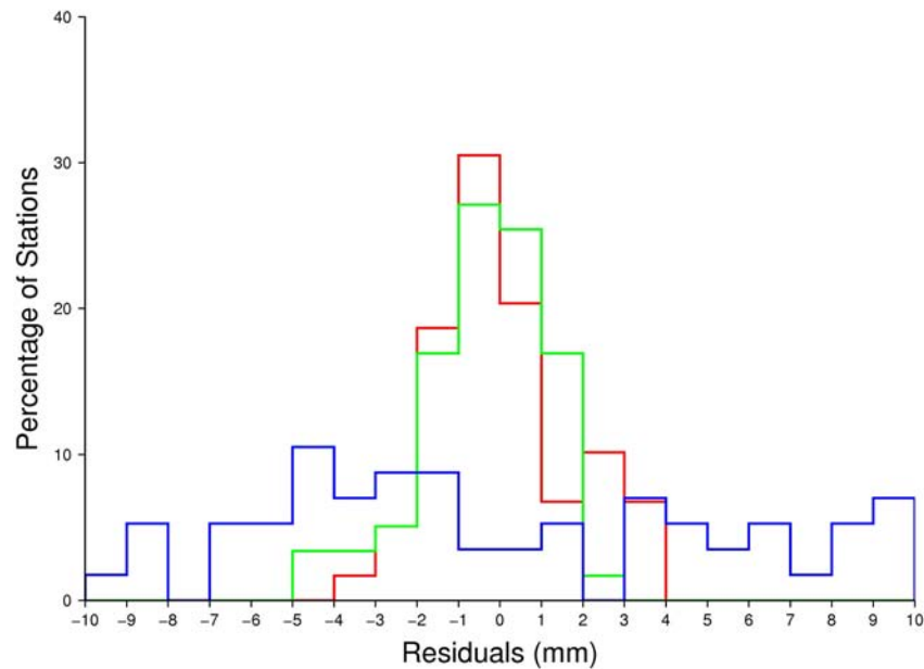
Figure 5.8. East (red), North (green) and Up (blue) position residuals of datum stations.
