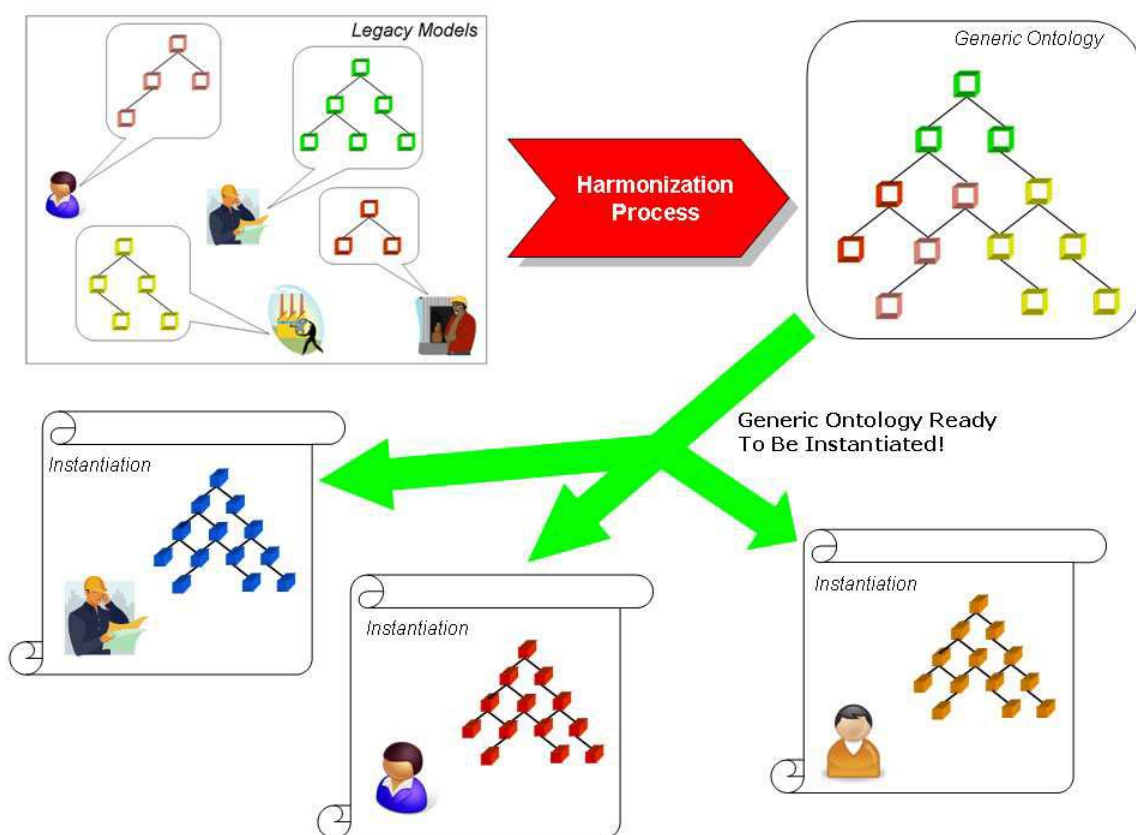
Figure 6.10 – Harmonization Process
