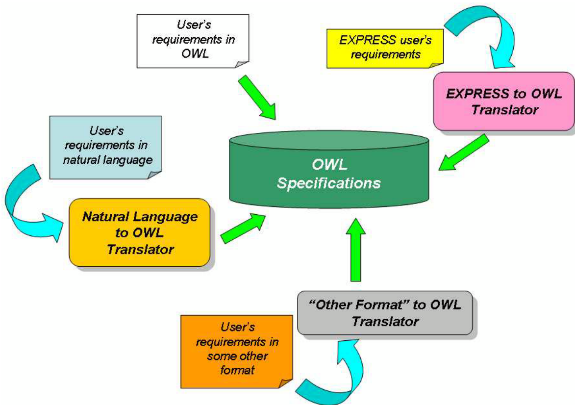
Figure 6.1– Formalization Process
