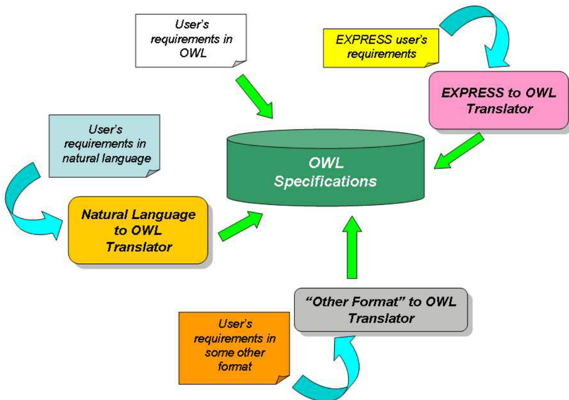
Figure 6.1– Formalization Process
