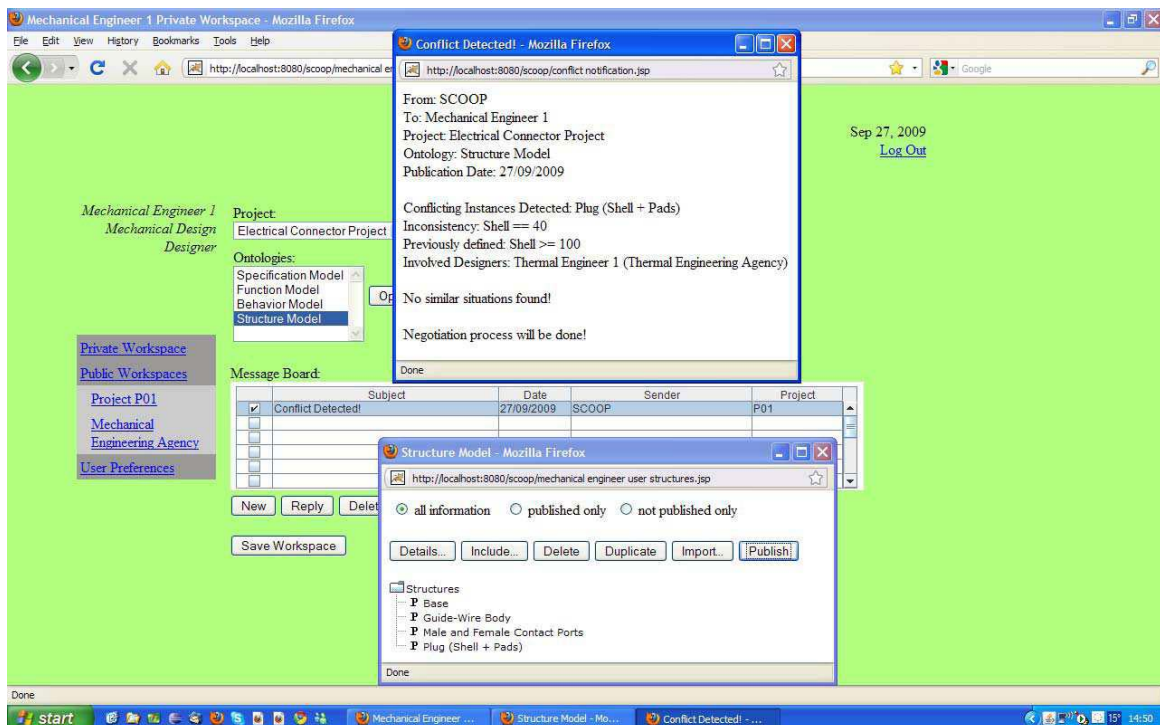
Figure 8.18 – Conflict Detected
