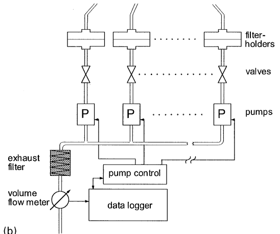
Fig. 1. Design of the sampling head (a) and the arrangement of filter pack units (b) of the automatic aerosol sampler.
