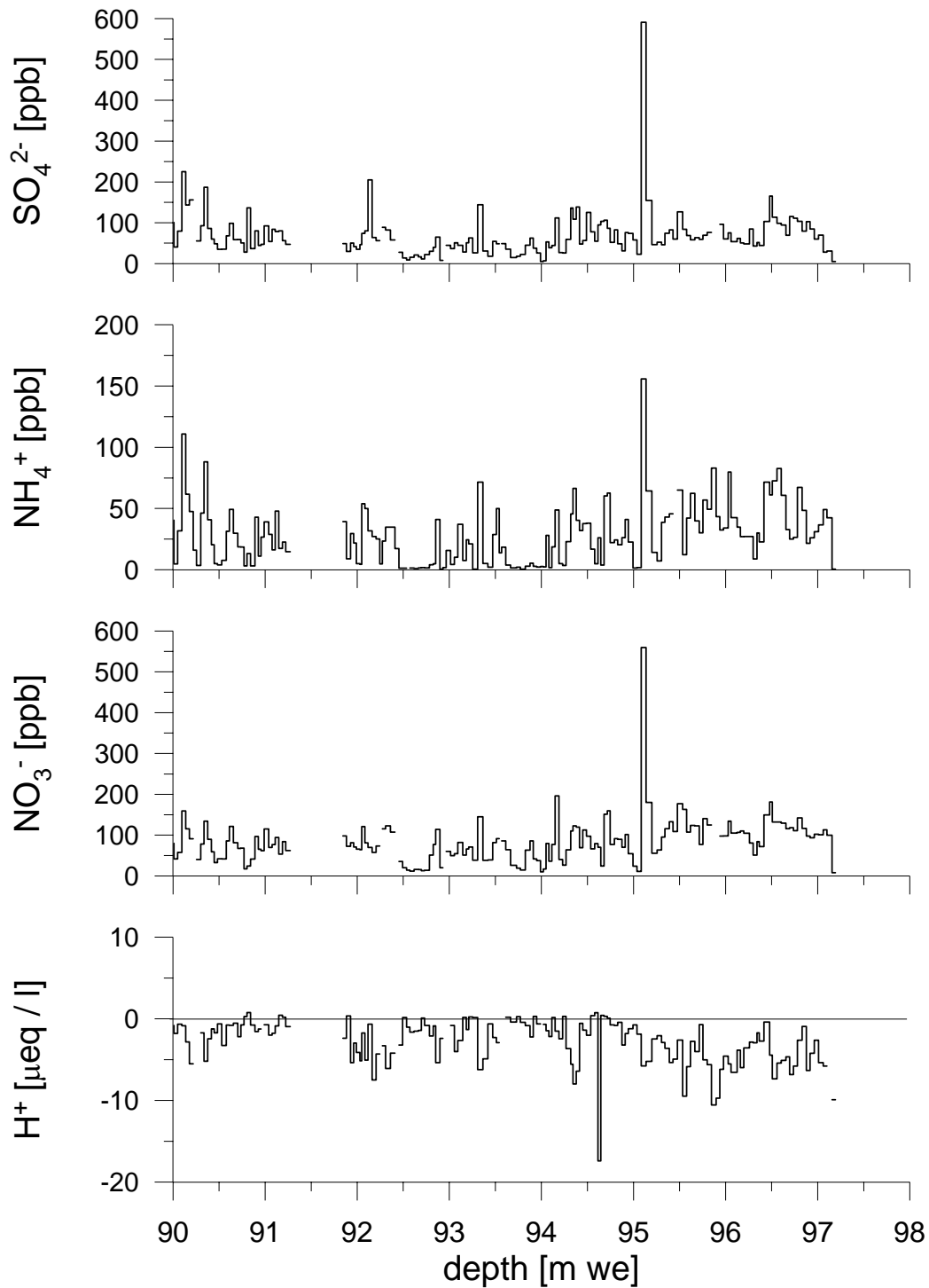
Figure 2.1a: Raw data profiles of \text{SO}_4^{2-} , \text{NH}_4^+ , \text{NO}_3^- , and \text{H}^+ versus depth along the bottom part of the C10 core.
