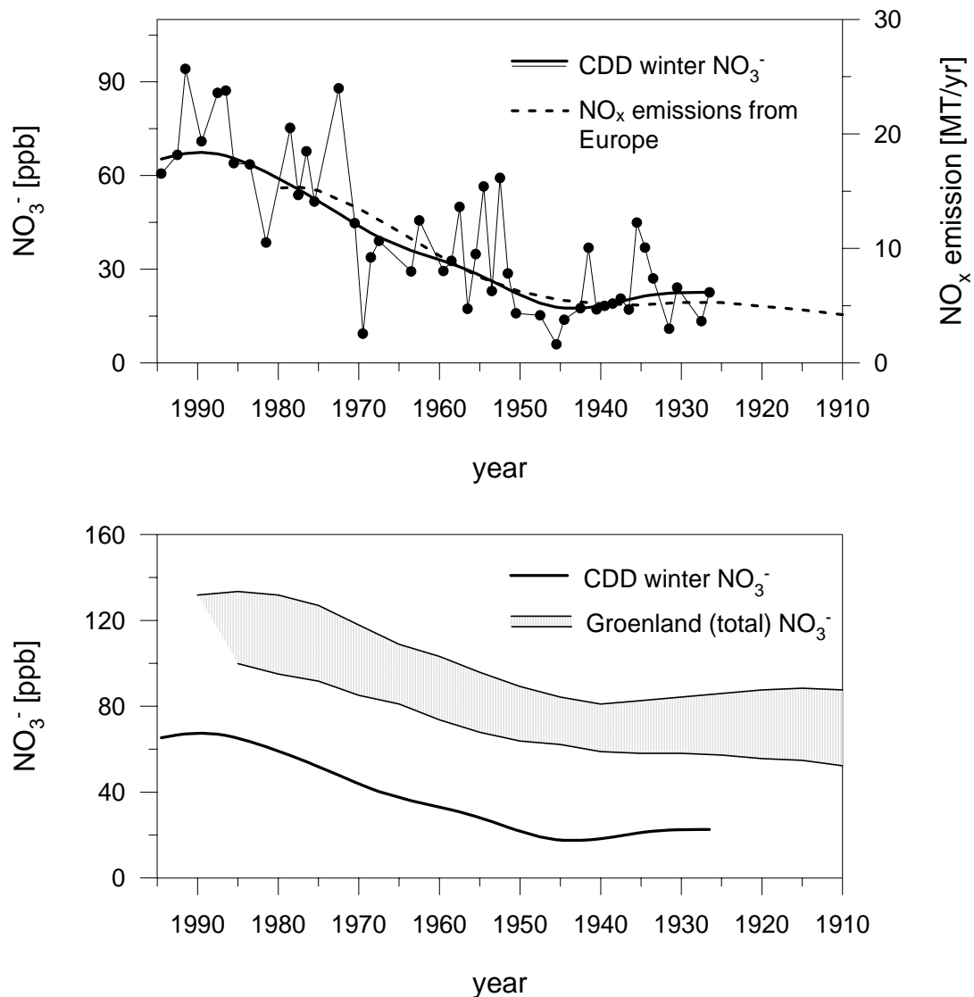
Figure 4.2: The CDD nitrate winter trend over the 20 th century. (Top) \text{NO}_x emissions from Europe (Hov et al., 1987) and nitrate winter trend (background conditions) derived from the CDD C10 core. The thin line with dots refers to the winter means of individual years. The solid line is the smoothed trend profile (robust spline smoothing). (Bottom) Smoothed nitrate winter trend from CDD (same as top) together with the envelop of nitrate annual trends observed at different Greenland drill sites (Fischer et al., 1998b and references there).
