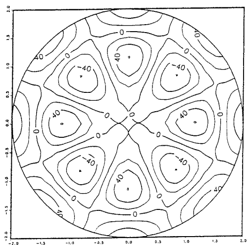
F.P. 24 m=4 \lambda=0.0044
