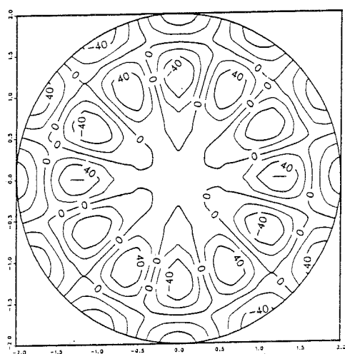
F.P. 42 m=6 \lambda=0.0019
