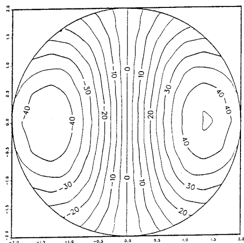
F.P. 2 m=1 \lambda=1.57
