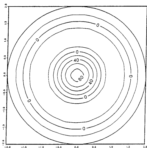
F.P. 15 m=0 \lambda=0.13
