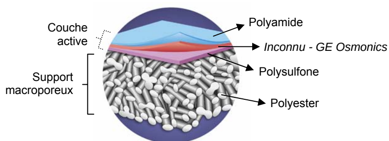
Figure III-1 . Membrane Desal DK
