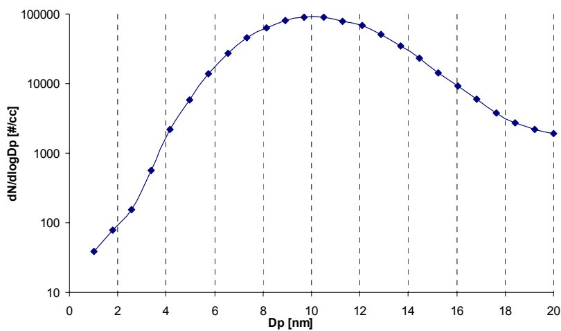
Figure A.1.15a: Size distribution from the wire generator (current 5 A, flow 3 \text{lmin}^{-1} ) measured by DMA and TSI Electrometer.
