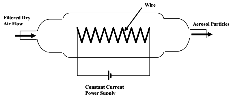
Figure A.1.14: Schematic of the hot wire generator. The cover is Pirex glass and the removable pure Cu-Zn wire have a spiral shape.
