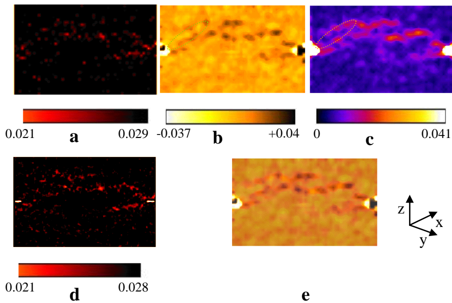
Fig. 6.11: Results from specimen Ve6: (a), (d) Vertical projections of the standard deviation values of HR x-ray images. Calculations were performed over sub-volumes of 20 \times 20 \times 20 \text{ voxels}^3 at a step of 20 and 5 voxels in each direction, respectively. Lower values of standard deviation were located inside compaction bands. Standard deviation values higher than 0.029 are visualised in black; (b) Volumetric strain fields for the same position; (c) Shear strain fields for the same position; (e) Volumetric and shear strain fields superposition ( x=15.676 \text{ mm} ). Calculations of the strain fields were performed over sub-volumes of 20 \times 20 \times 20 \text{ voxels}^3 at spacing of 20 voxels in each direction.
